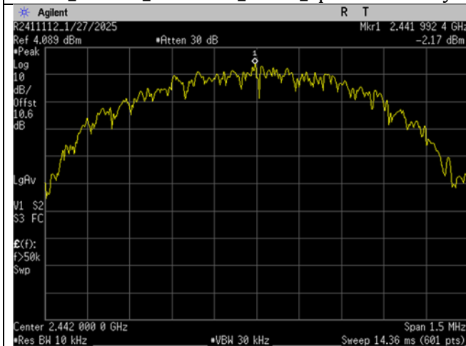
BLE_Mid Ch_2442MHz_1MBit_Spectral Density
