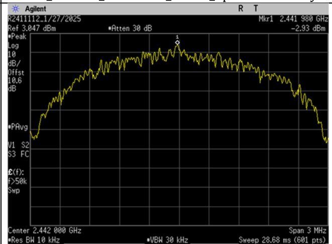
BLE_Mid Ch_2442MHz_2MBit_Spectral Density
