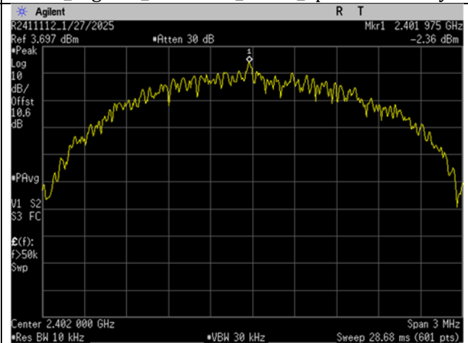
BLE_Low Ch_2402MHz_2MBit_Spectral Density
