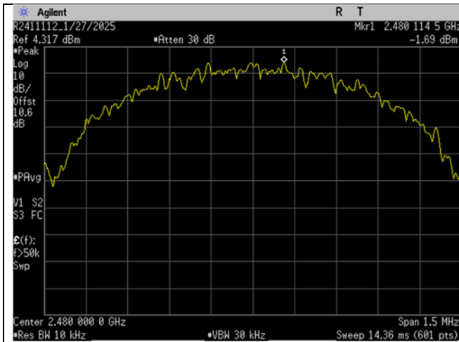
BLE_High Ch_2480MHz_1MBit_Spectral Density
