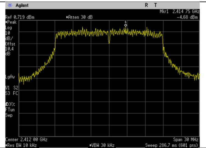
WIFI_Low Ch_2412MHz_20MHz BW_n-mode_Spectral Density
