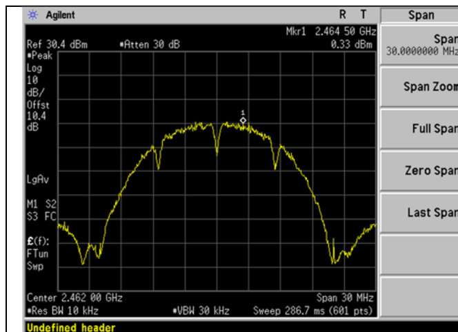
WIFI_High Ch_2462MHz_20MHz BW_b-mode_Spectral Density
