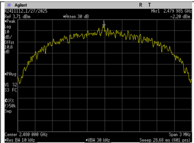
BLE_High Ch_2480MHz_2MBit_Spectral Density
