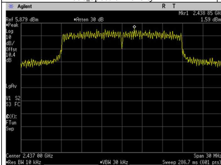
WIFI_Mid Ch_2437MHz_20MHz BW_n-mode_Spectral Density
