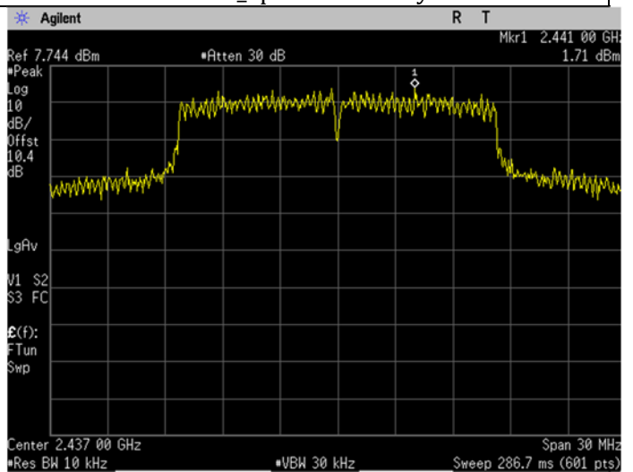
WIFI_Mid Ch_2437MHz_20MHz BW_g-mode_Spectral Density
