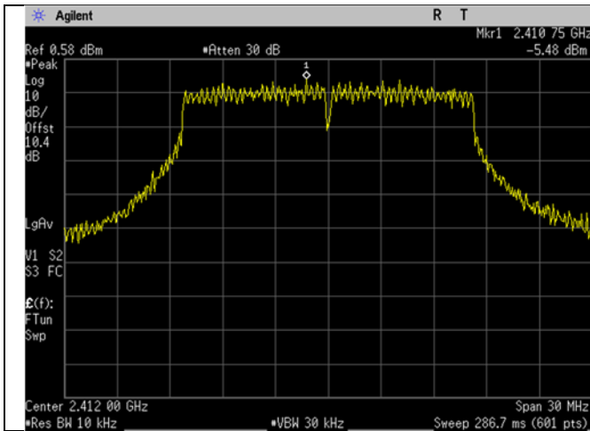
WIFI_Low Ch_2412MHz_20MHz BW_g-mode_Spectral Density
