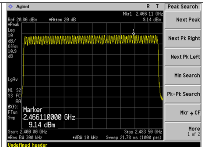
\pi/4 -DQPSK no of hopping channel
