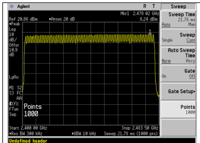
8DPSK no of hopping channel
