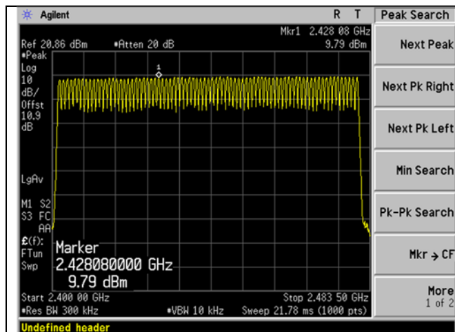
GFSK no of hopping channel
