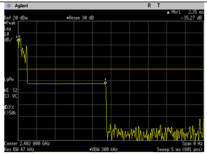
3DH3 dwell time
