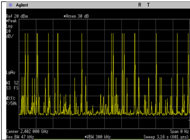
DH3 dwell time 31-6sec
