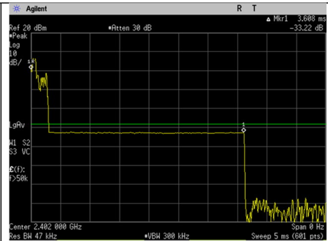
2DH5 dwell time
