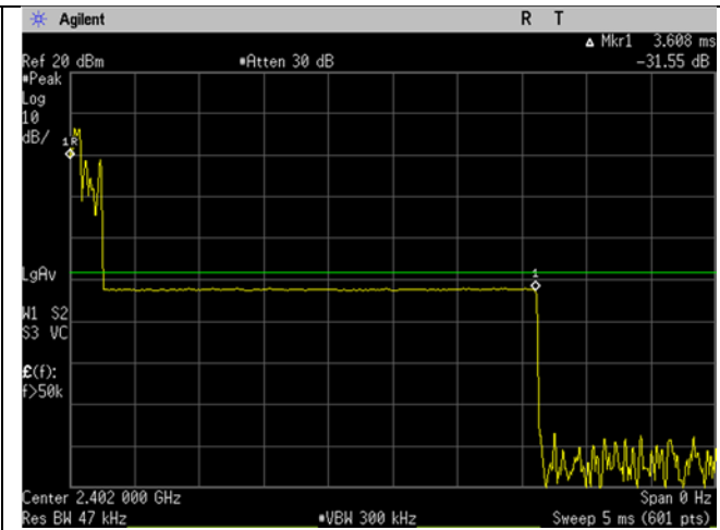
3DH5 dwell time
