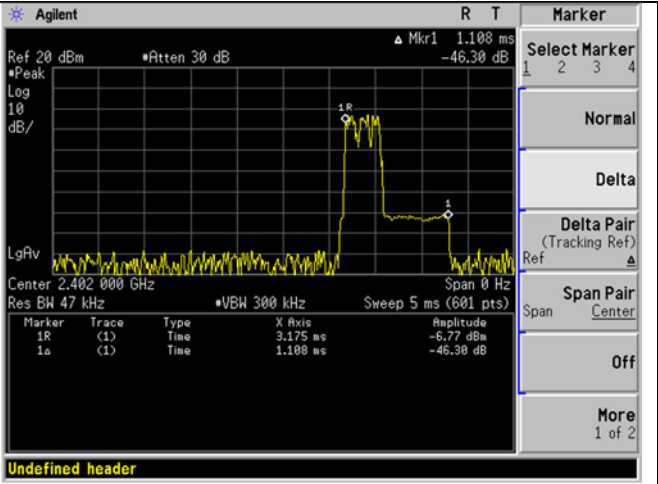
GFSK dwell time
