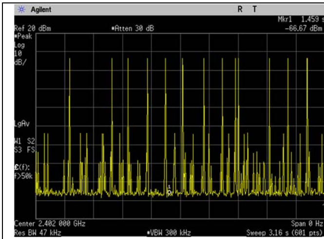
3DH3 dwell time 31-6sec
