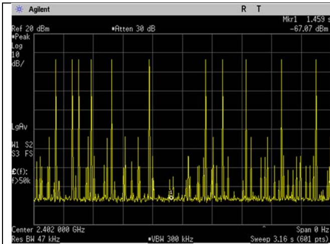
3DH5 dwell time 31-6sec
