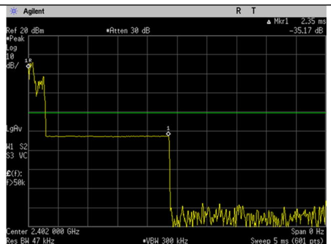
2DH3 dwell time
