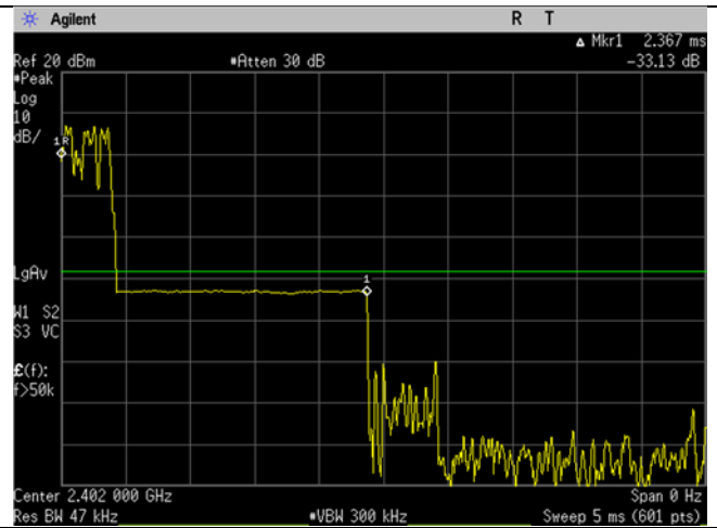
DH3 dwell time
