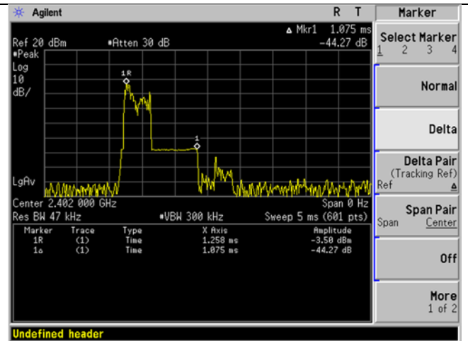
8DPSK dwell time
