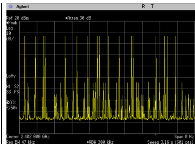
2DH3 dwell time 31-6sec
