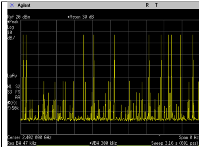
8DPSK dwell time 31-6sec
