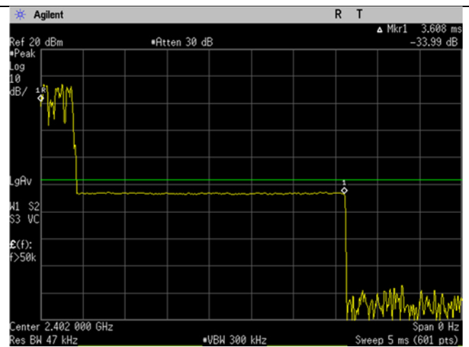
DH5 dwell time
