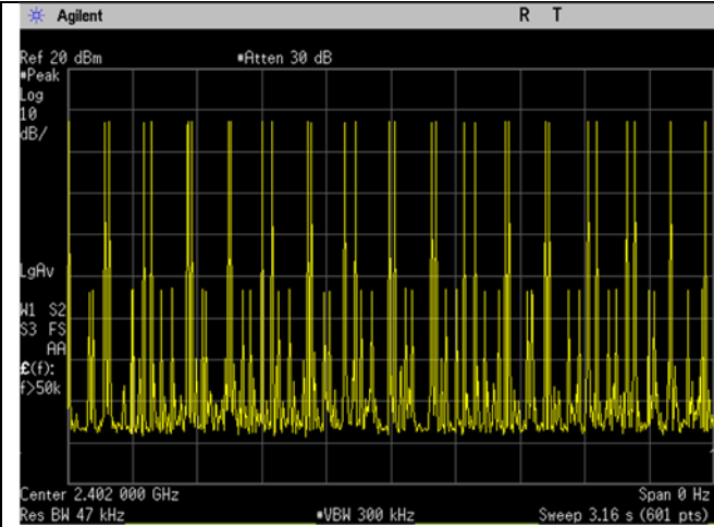
GFSK dwell time 31-6sec
