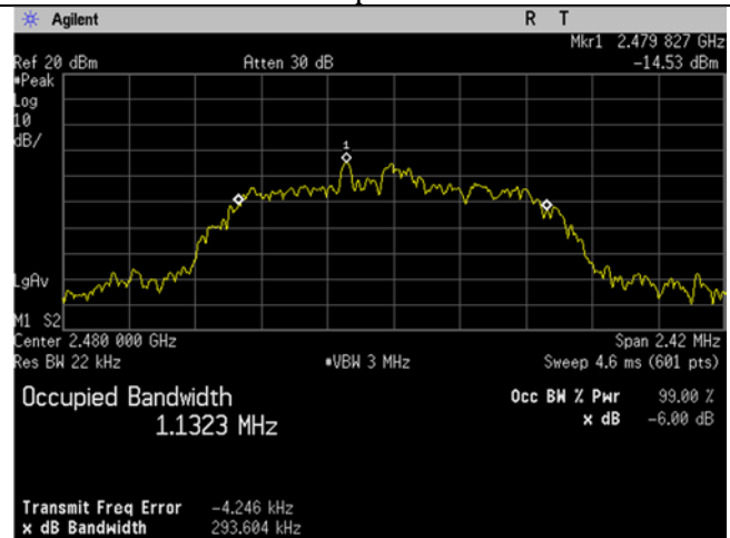
8DPSK 99 percent Occupied Bandwidth high
