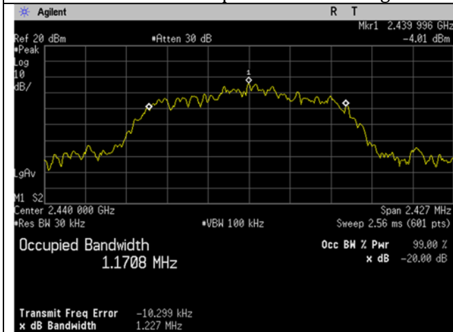
8DPSK 20db Occupied Bandwidth mid
