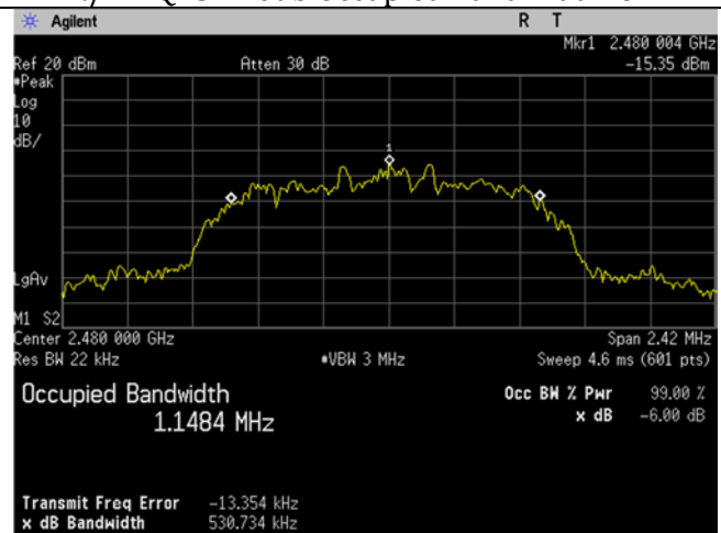
\pi/4 -DQPSK 99 percent Occupied Bandwidth high
