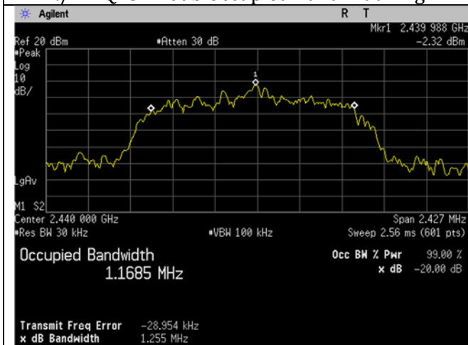
\pi/4 -DQPSK 20db Occupied Bandwidth mid
