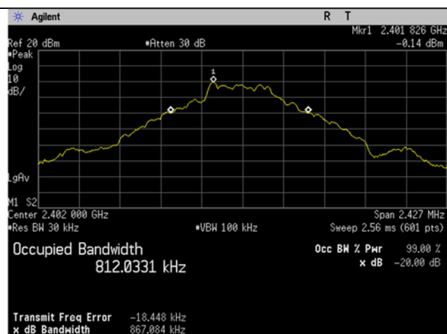
GFSK 20db Occupied Bandwidth low
