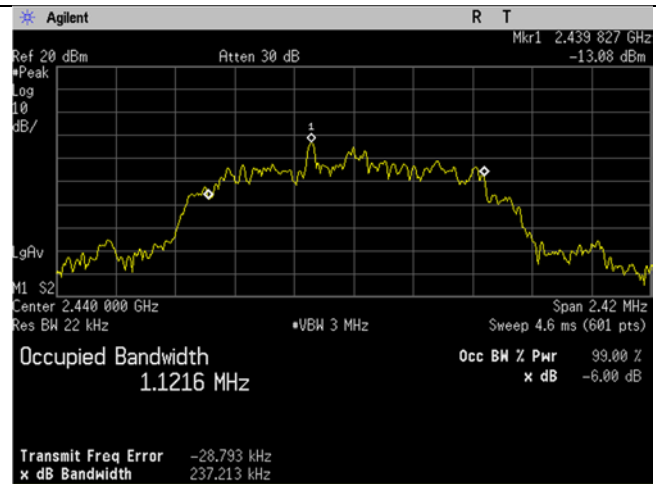
\pi/4 -DQPSK 99 percent Occupied Bandwidth mid
