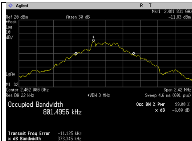
GFSK 99 percent Occupied Bandwidth low
