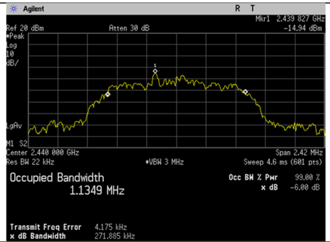
8DPSK 99 percent Occupied Bandwidth mid
