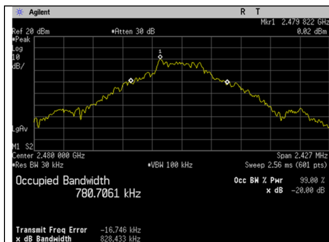
GFSK 20db Occupied Bandwidth high
