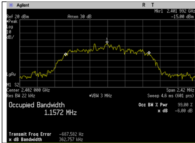
8DPSK 99 percent Occupied Bandwidth low
