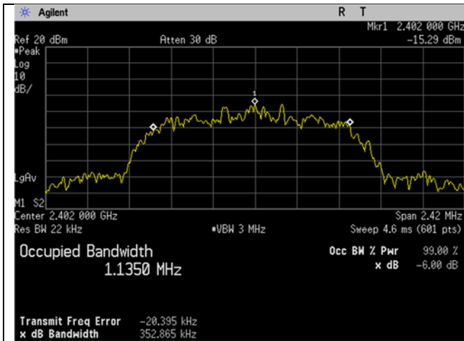
\pi/4 -DQPSK 99 percent Occupied Bandwidth low
