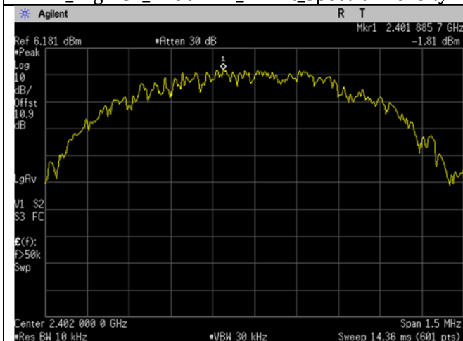
BLE_Low Ch_2402MHz_1MBit_Spectral Density
