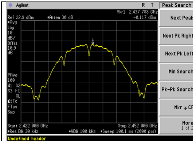
WIFI_Mid Ch_2437MHz_20MHz BW Spectral Density_b-mode
