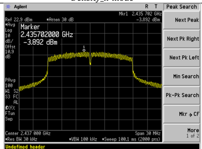
WIFI_Low Ch_2437MHz_20MHz BW Spectral Density_n-mode
