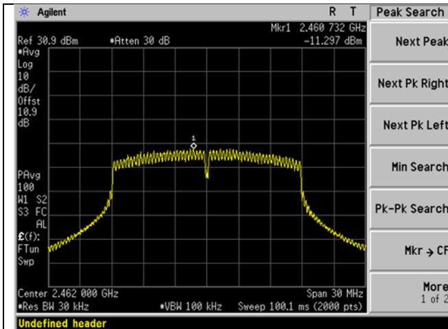
WIFI_High Ch_2462MHz_20MHz BW Spectral Density_n-mode
