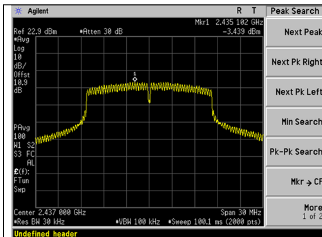
WIFI_High Ch_2437MHz_20MHz BW Spectral Density_g-mode
