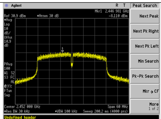
WIFI_High Ch_2452MHz_40MHz BW Spectral Density_n-mode
