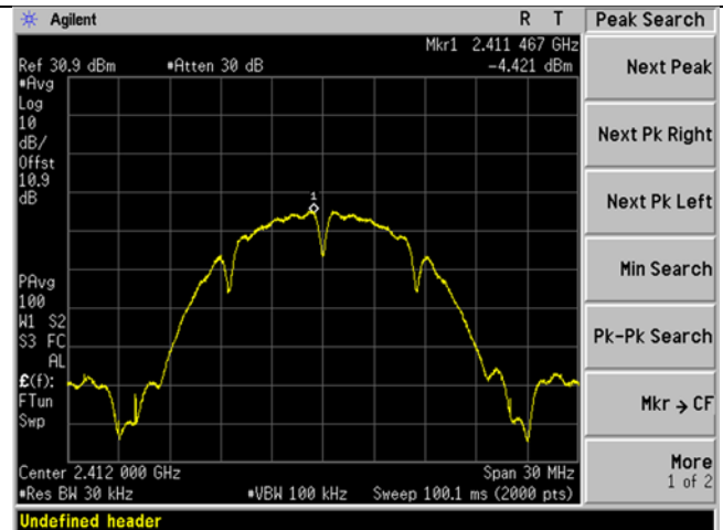
WIFI_Low Ch_2412MHz_20MHz BW Spectral Density_b-mode
