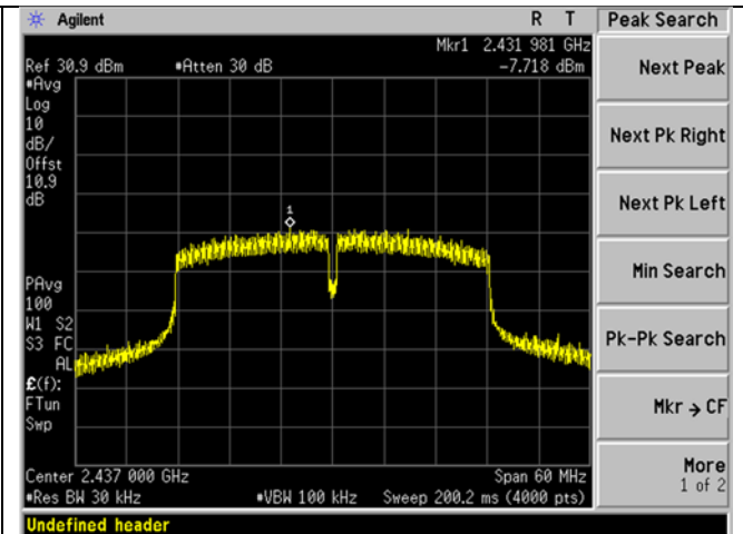
WIFI_Mid Ch_2437MHz_40MHz BW Spectral Density_n-mode
