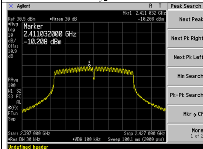
WIFI_Low Ch_2412MHz_20MHz BW Spectral Density_g-mode
