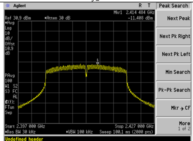
WIFI_Low Ch_2412MHz_20MHz BW Spectral Density_n-mode
