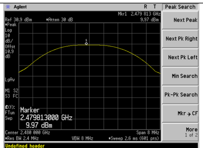
BLE_High Ch_2480MHz_2MBit_Output Power
