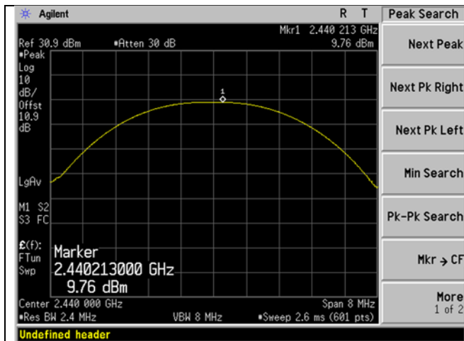
BLE_Mid Ch_2440MHz_1MBit_Output Power
