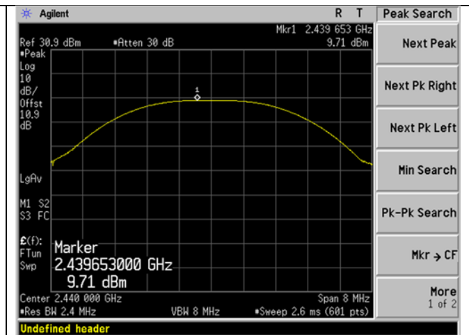
BLE_Mid Ch_2440MHz_2MBit_Output Power
