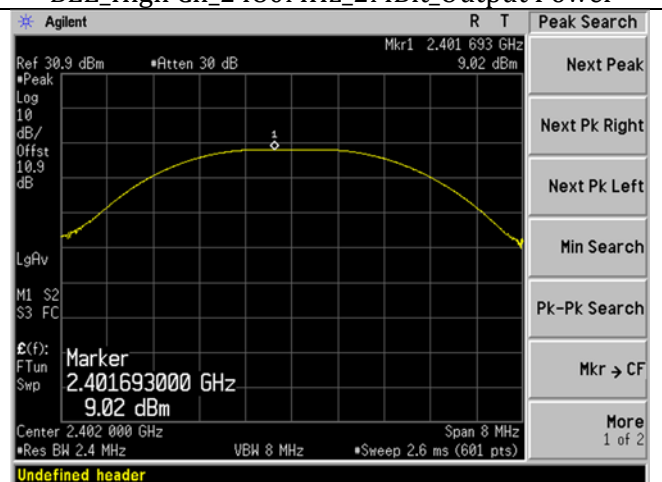
BLE_Low Ch_2402MHz_2MBit_Output Power
