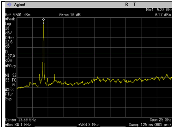
U-NII-2A_5290MHz_High_Mid Ch_58_80MHz BW_ac-mode_-27dBm_1-26GHz
