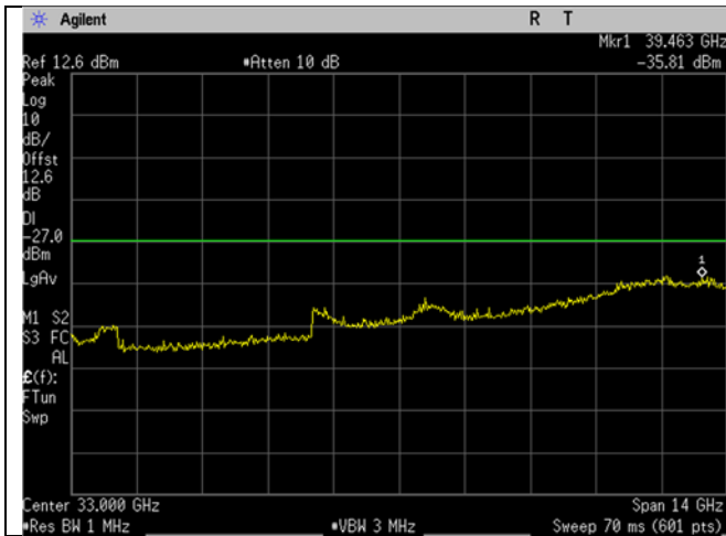
U-NII-3_5755MHz_Low Ch_151_40MHz BW_n/ac-mode_-27dBm_26-40GHz_Peak
