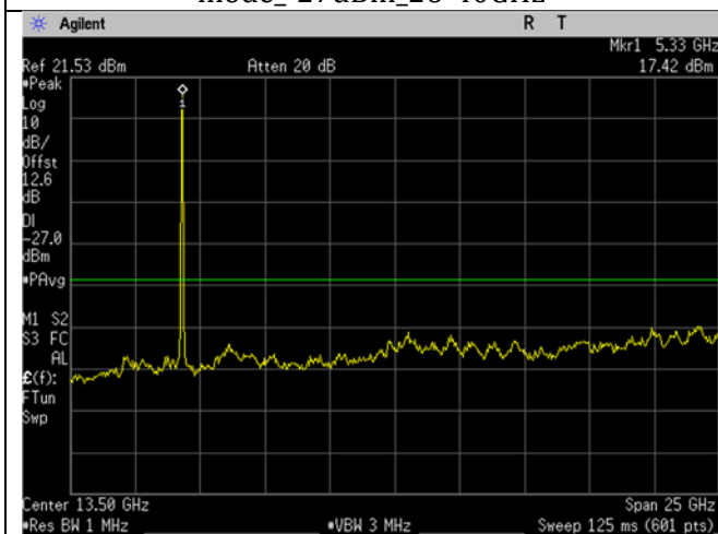
U-NII-2A_5320MHz_High Ch_64_20MHz BW_a- mode_-27dBm_1-26GHz
