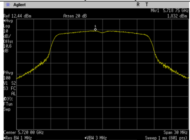
U-NII-2C_5720MHz_High Ch_144_20MHz BW_a-mode_Spectral Density
