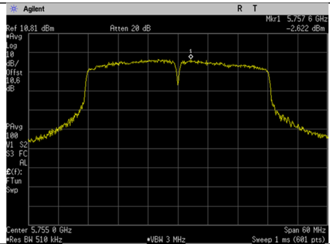
U-NII-3_5755MHz_Low Ch_151_40MHz BW_n/ac - mode_Spectral Density
