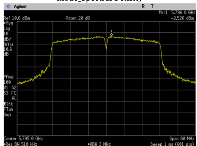
U-NII-3_5795MHz_High_Mid Ch_159_40MHz BW_n/ac - mode_Spectral Density
