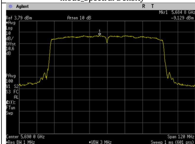
U-NII-2C_5690MHz_High Ch_138_80MHz BW_ac-mode_Spectral Density
