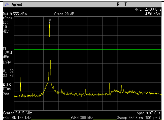
2437MHz_20MHz_g-mode_30MHz-10GHz
