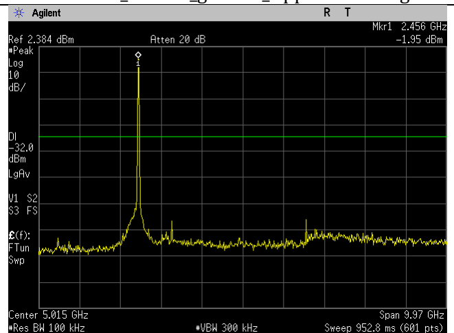
2462MHz_20MHz_n-mode_30MHz-10GHz
