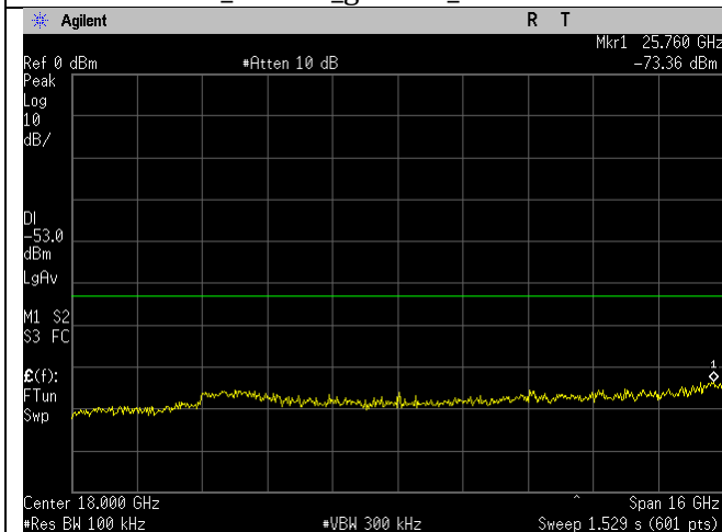
2462MHz_20MHz_n-mode_10-26GHz
