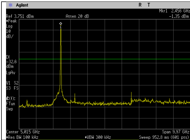
2462MHz_20MHz_g-mode_30MHz-10GHz
