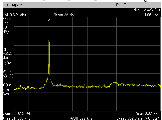
2412MHz_20MHz_g-mode_30MHz-10GHz
