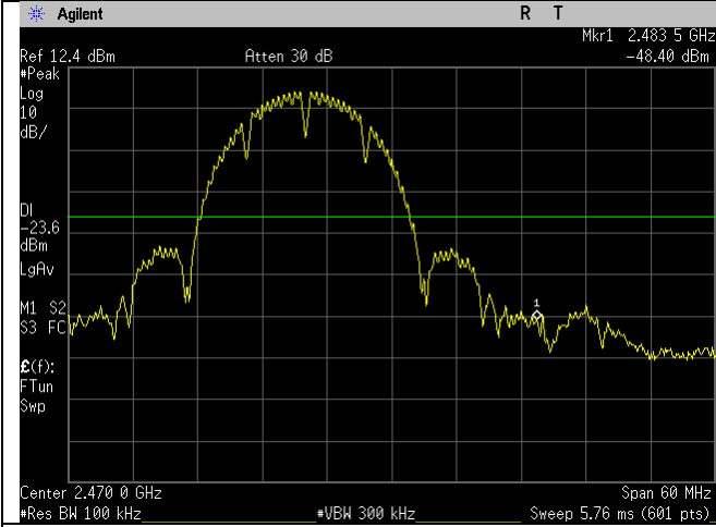
2462MHz_20MHz_b-mode_Upper Band Edge
