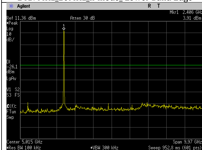
2412MHz_20MHz_b-mode_30MHz-10GHz
