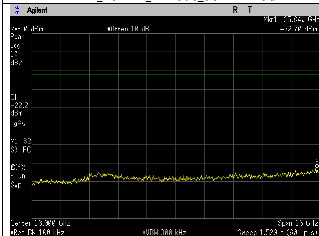
2437MHz_20MHz_b-mode_10-26GHz
