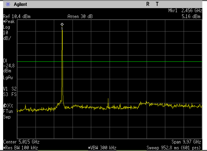
2462MHz_20MHz_b-mode_30MHz-10GHz
