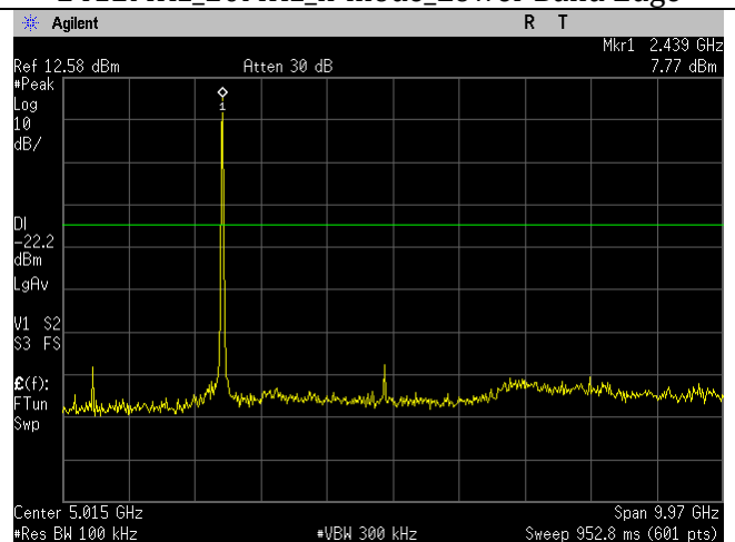
2437MHz_20MHz_b-mode_30MHz-10GHz
