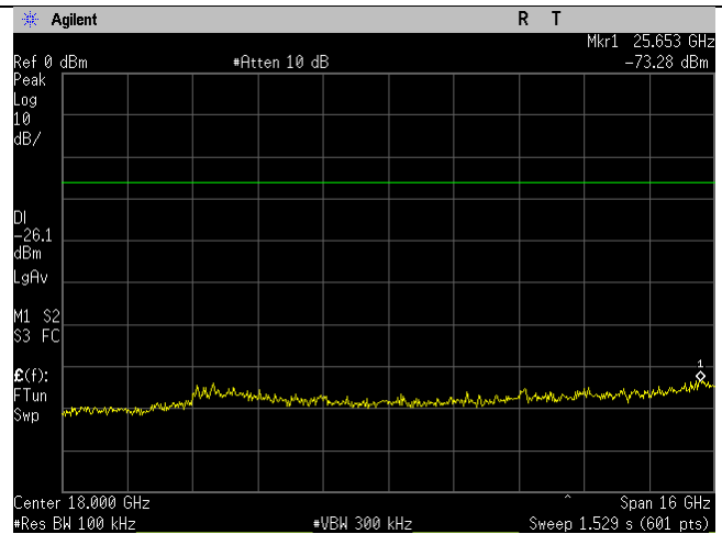
2412MHz_20MHz_b-mode_10-26GHz
