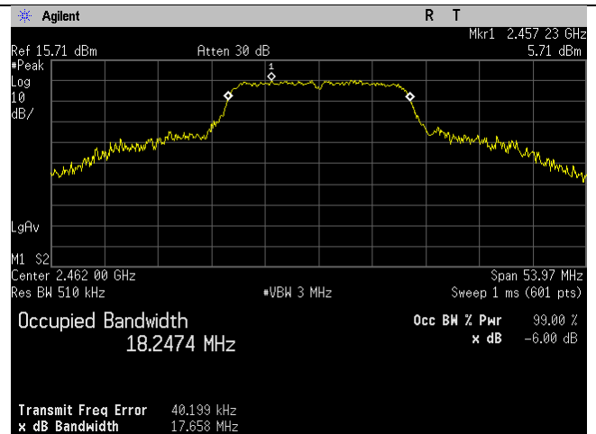
2462MHz_20MHz BW_n-mode_99 percent
