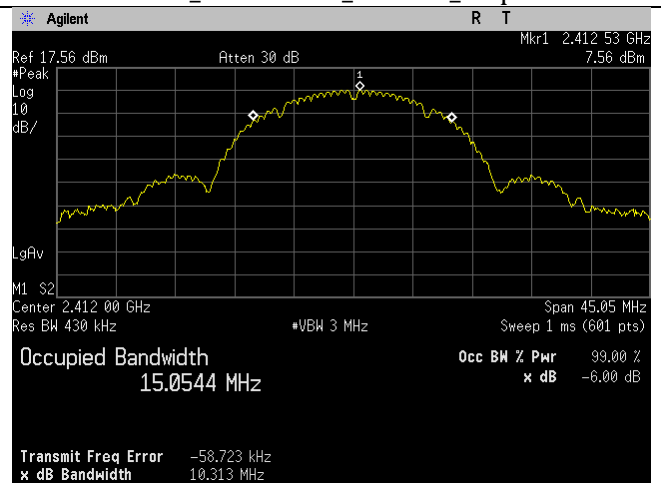
2412MHz_20MHz BW_b-mode_99 percent
