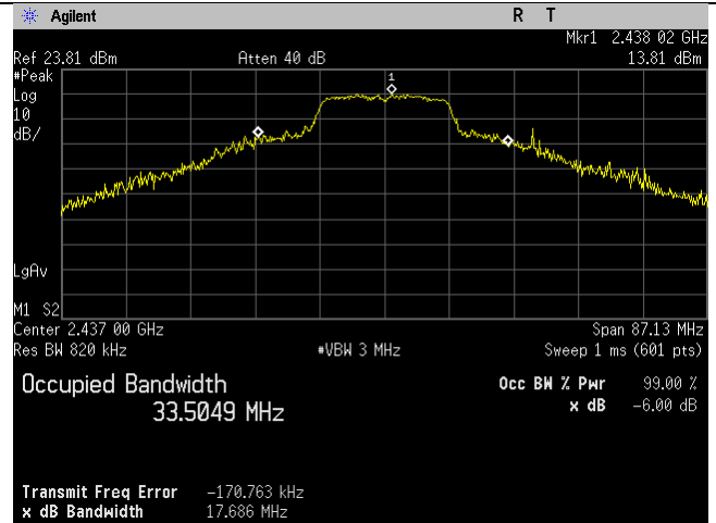
2437MHz_20MHz BW_n-mode_99 percent
