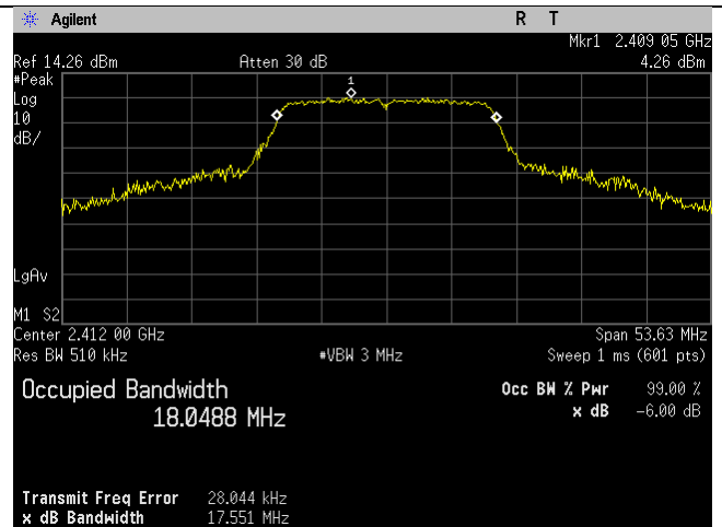
2412MHz_20MHz BW_n-mode_99 percent
