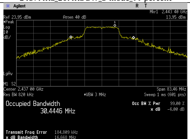
2437MHz_20MHz BW_g-mode_99 percent
