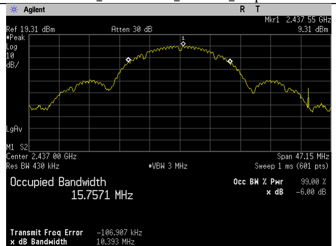
2437MHz_20MHz BW_b-mode_99 percent
