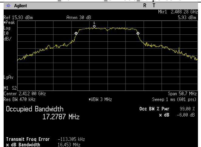
2412MHz_20MHz BW_g-mode_99 percent
