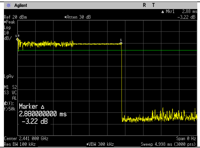
Middle Channel Dwell Time 3DH5
