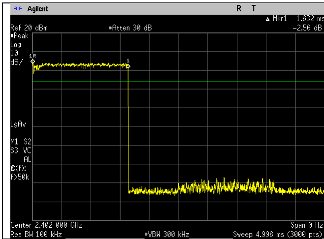
Low Channel Dwell Time DH3
