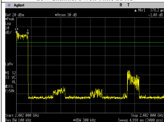
Low Channel Dwell Time 3DH1
