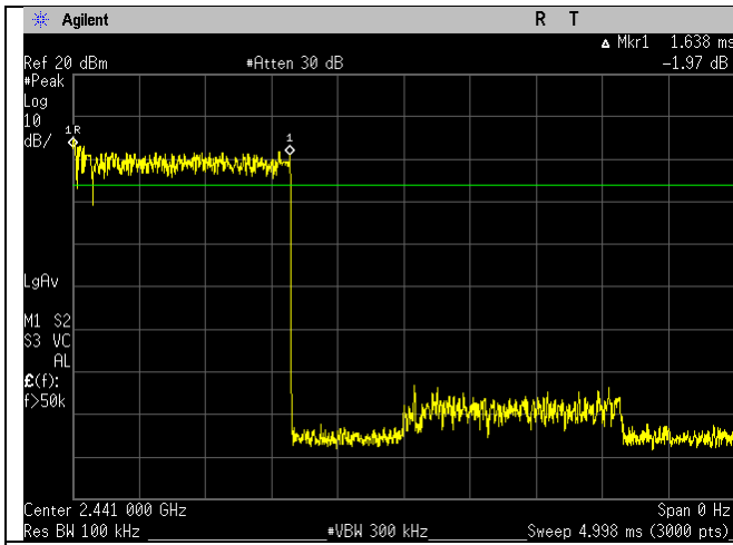
Middle Channel Dwell Time 3DH3
