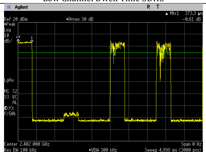
Low Channel Dwell Time DH1
