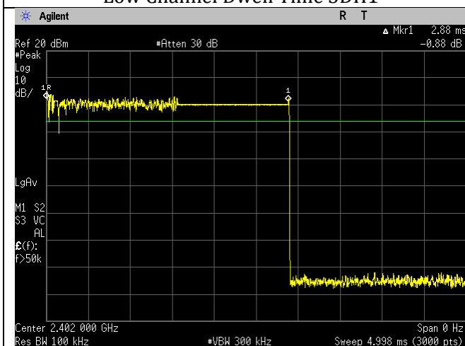
Low Channel Dwell Time 3DH5
