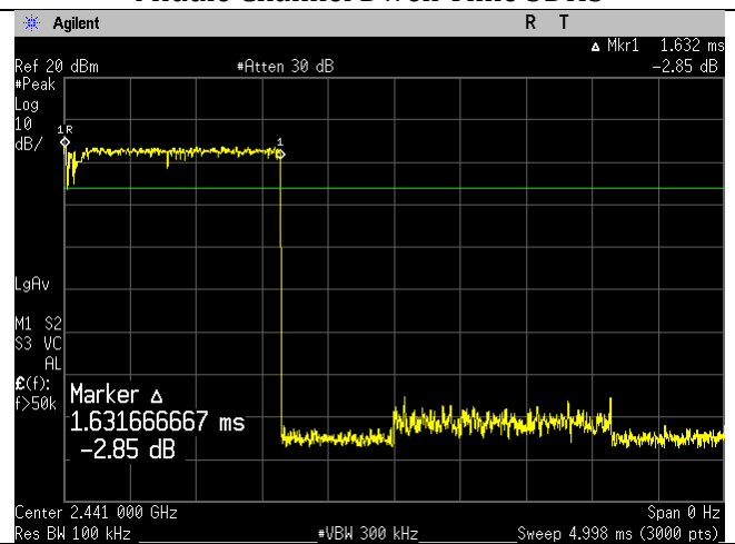
Middle Channel Dwell Time DH3
