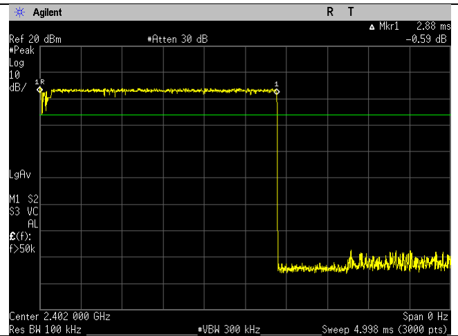
Low Channel Dwell Time DH5
