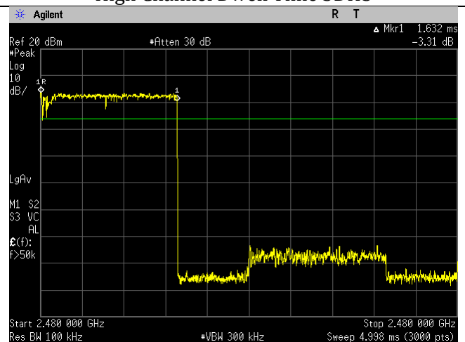
High Channel Dwell Time DH3
