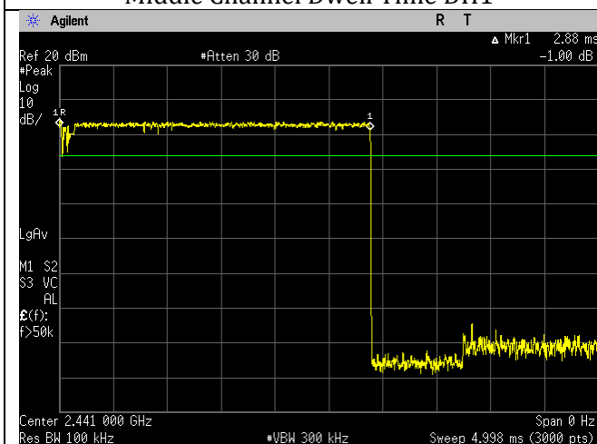
Middle Channel Dwell Time DH5
