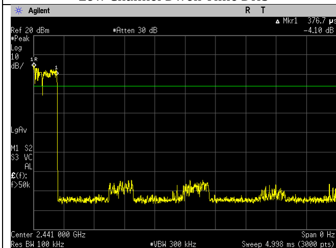
Middle Channel Dwell Time 2DH1
