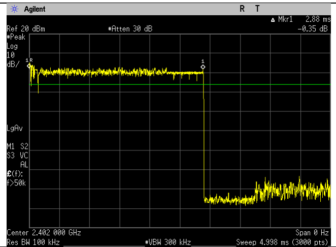
Low Channel Dwell Time 2DH5
