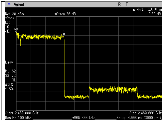
High Channel Dwell Time 3DH3
