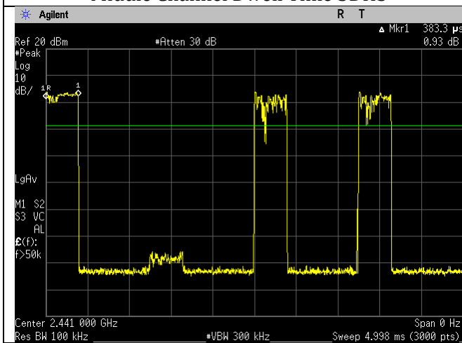
Middle Channel Dwell Time DH1
