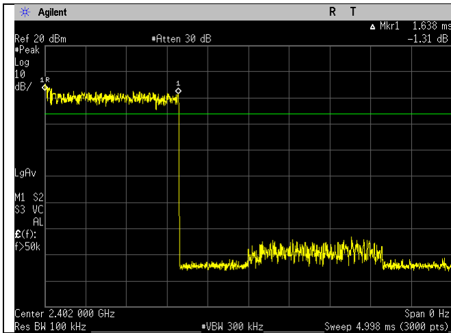
Low Channel Dwell Time 2DH3
