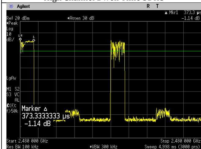
High Channel Dwell Time DH1
