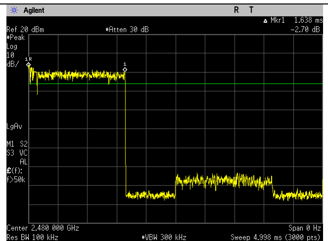
High Channel Dwell Time 2DH3
