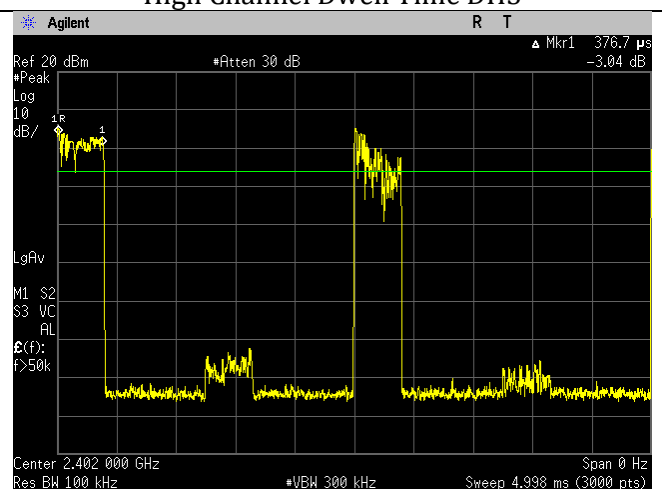
Low Channel Dwell Time 2DH1
