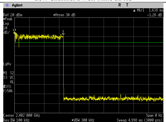
Low Channel Dwell Time 3DH3
