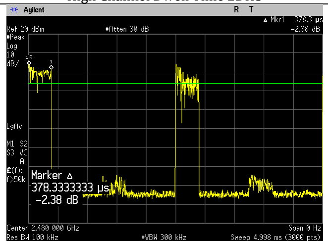
High Channel Dwell Time 3DH1
