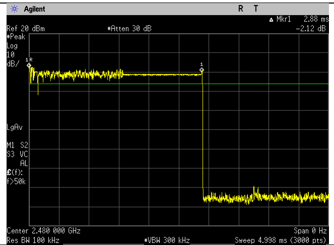
High Channel Dwell Time 3DH5
