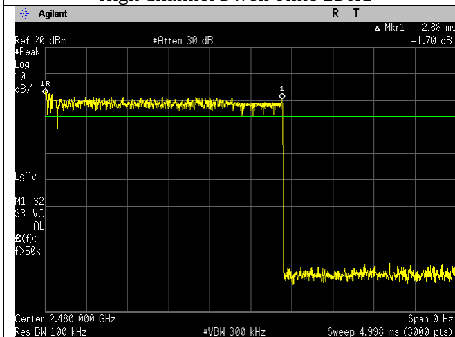
High Channel Dwell Time 2DH5
