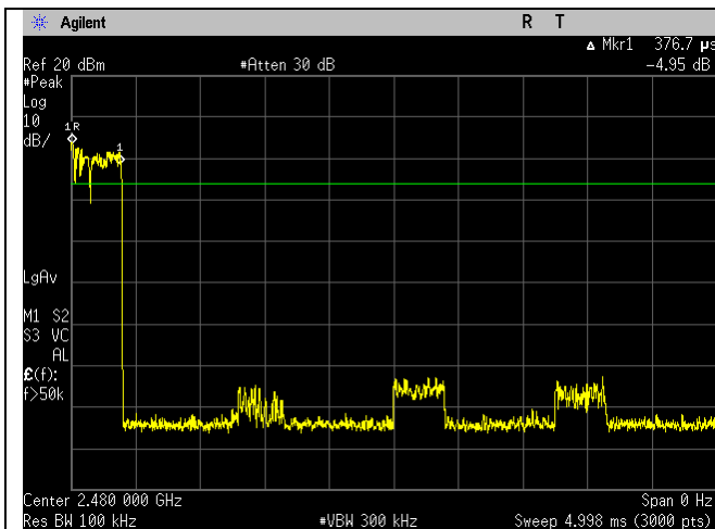
High Channel Dwell Time 2DH1
