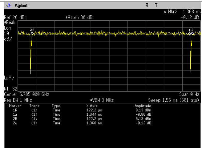
5-Band_a_mode_Duty_Cycle
