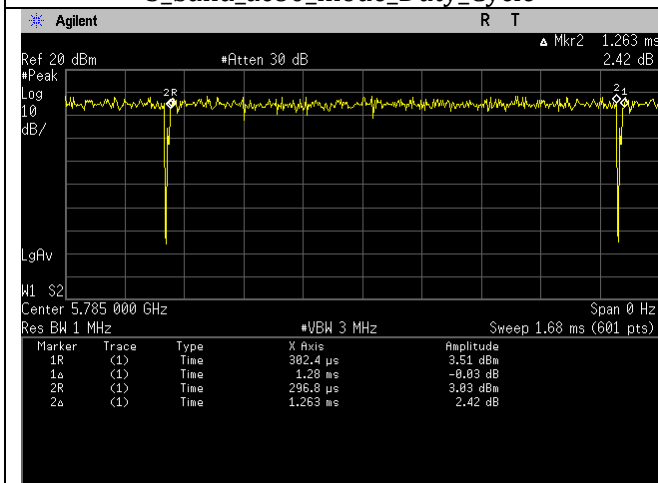
5_Band_n20_mode_Duty_Cycle
