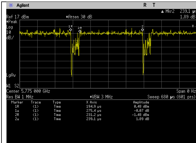
5_band_ac80_mode_Duty_Cycle
