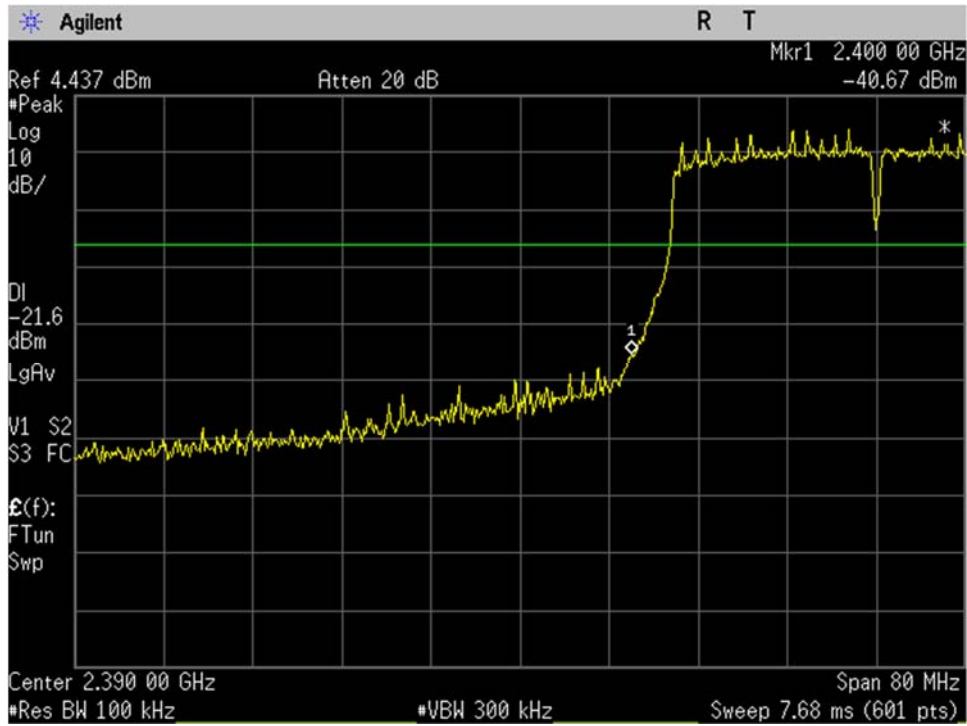
WIFI_Low Ch_2422MHz_40MHz BW_n-mode_-20dBc_Lower Band Edge_Port 1
