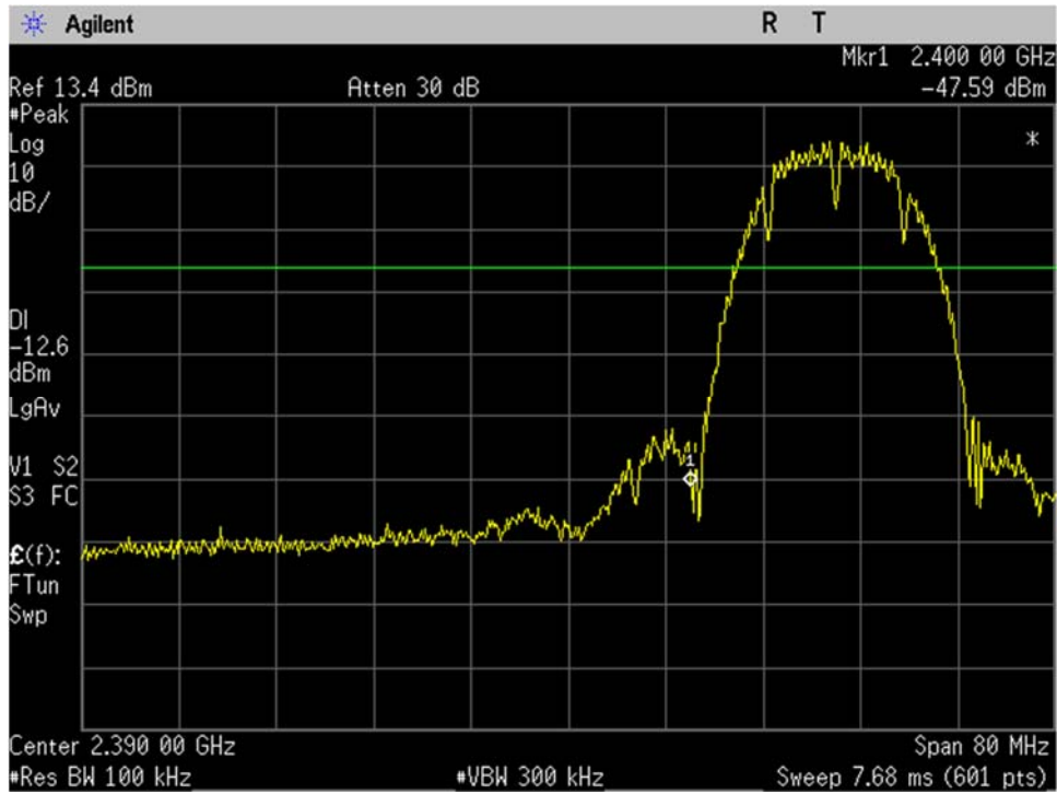
WIFI_Low Ch_2412MHz_20MHz BW_b-mode_-20dBc_Lower Band Edge_Port 2
