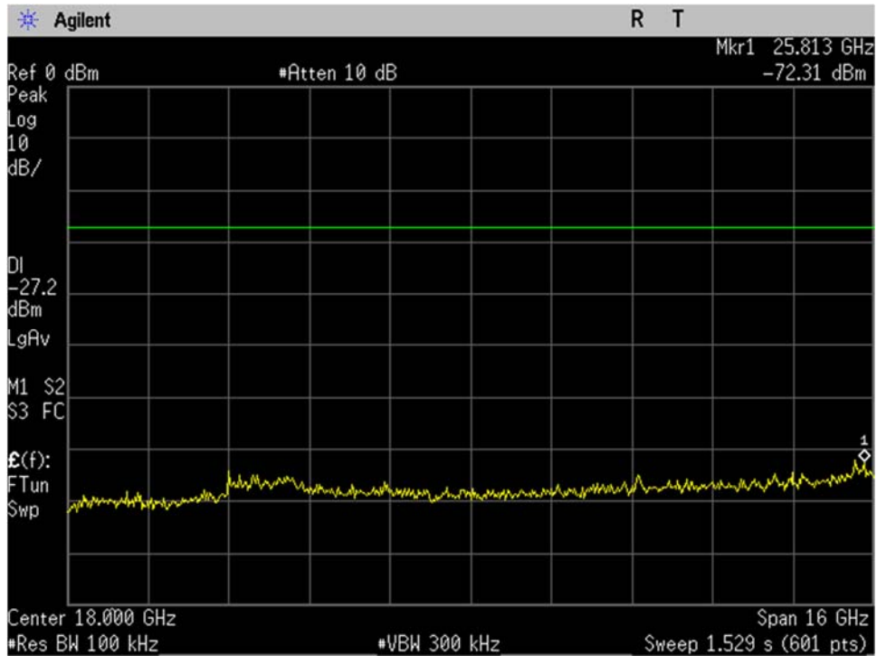
WIFI_Low Ch_2422MHz_40MHz BW_n-mode_-20dBc_10-26GHz_Port 2
