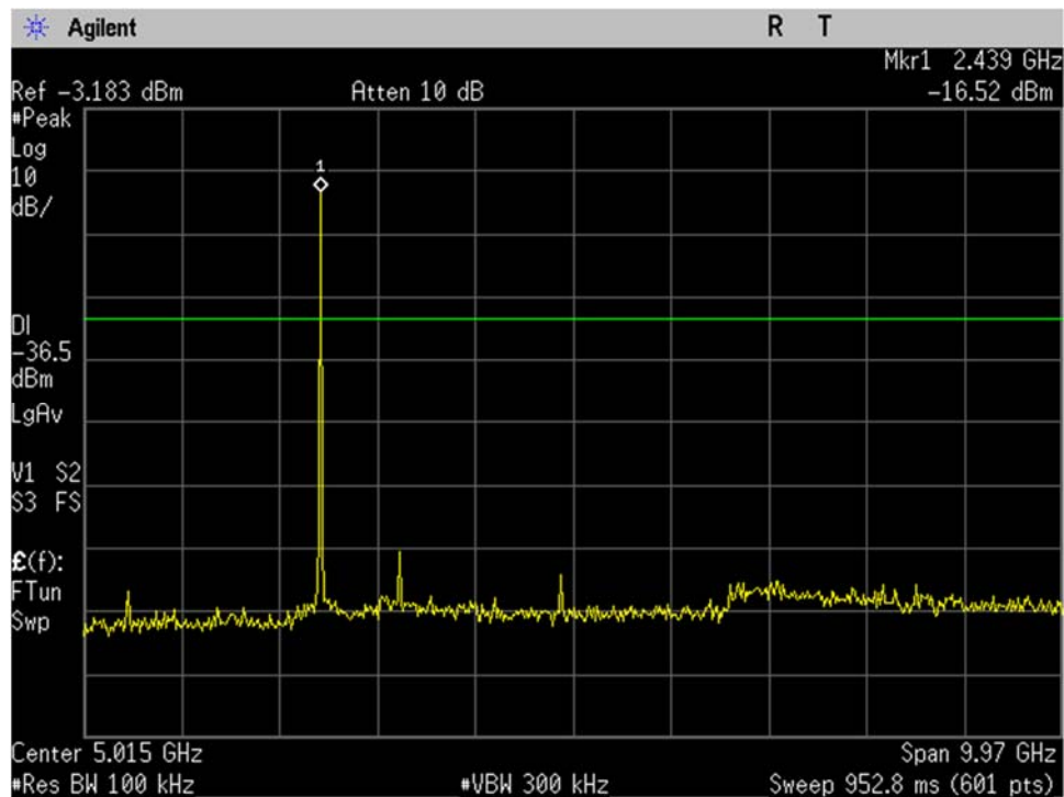
BLE_Mid Ch_2440MHz_2MBit_-20dBc_30MHz-10GHz_Port 1
