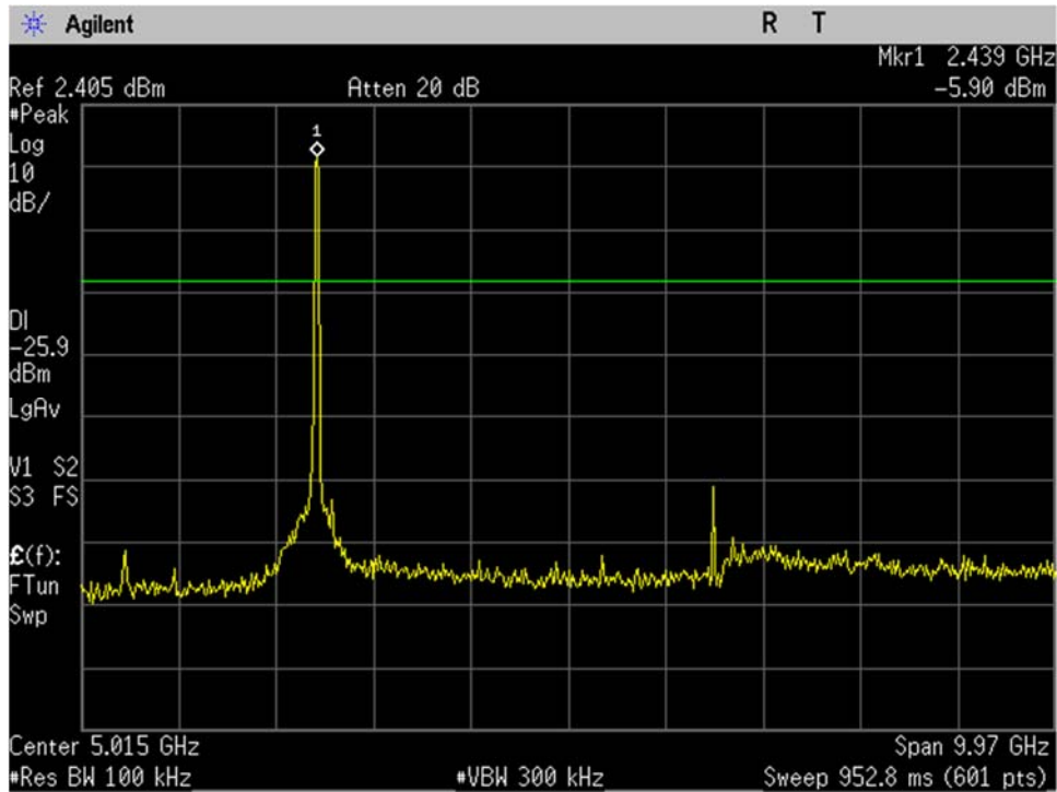
WIFI_Mid Ch_2437MHz_40MHz BW_n-mode_-20dBc_30MHz-10GHz_Port 1
