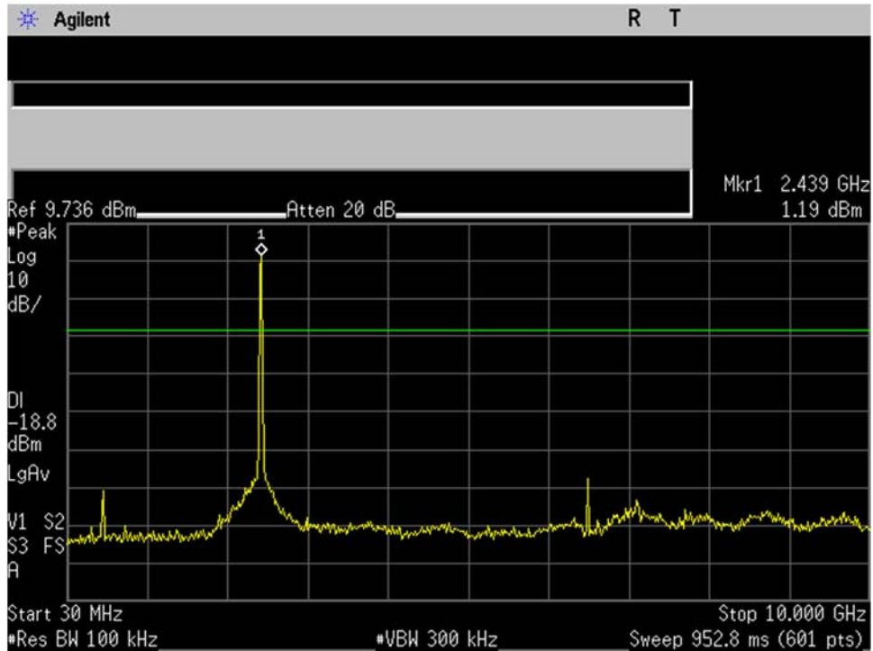
WIFI_Mid Ch_2437MHz_20MHz BW_g-mode_-20dBc_30MHz-10GHz_Port 1
