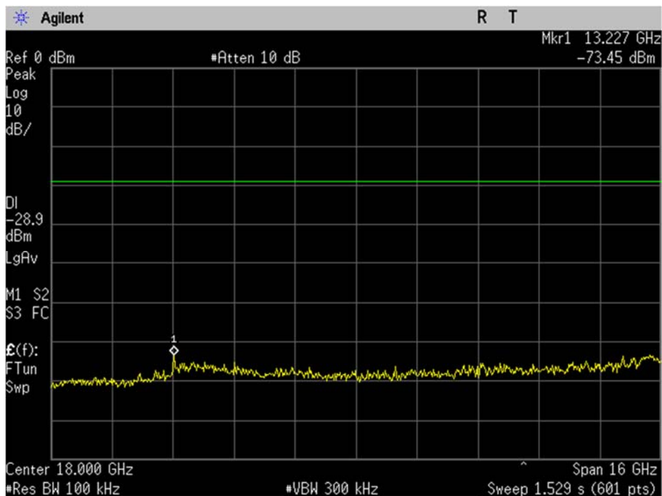
WIFI_Mid Ch_2437MHz_40MHz BW_n-mode_-20dBc_10-26GHz_Port 2
