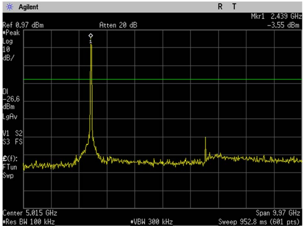
WIFI_High Ch_2452MHz_40MHz BW_n-mode_-20dBc_30MHz-10GHz_Port 1
