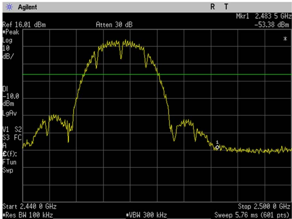
WIFI_High Ch_2462MHz_20MHz BW_b-mode_-20dBc_Upper Band Edge_Port 1
