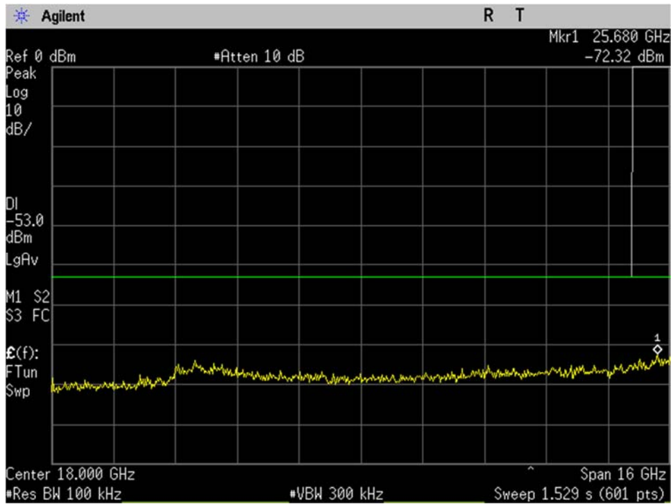
WIFI_Low Ch_2412MHz_20MHz BW_n-mode_-20dBc_10-26GHz_Port 1
