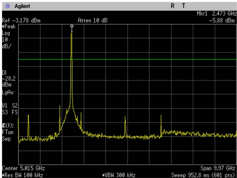
WIFI_High Ch_2452MHz_40MHz BW_n-mode_-20dBc_30MHz-10GHz_Port 2
