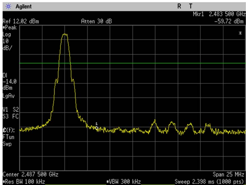
BLE_High Ch_2480MHz_1MBit_-20dBc_Upper Band Edge_Port 1
