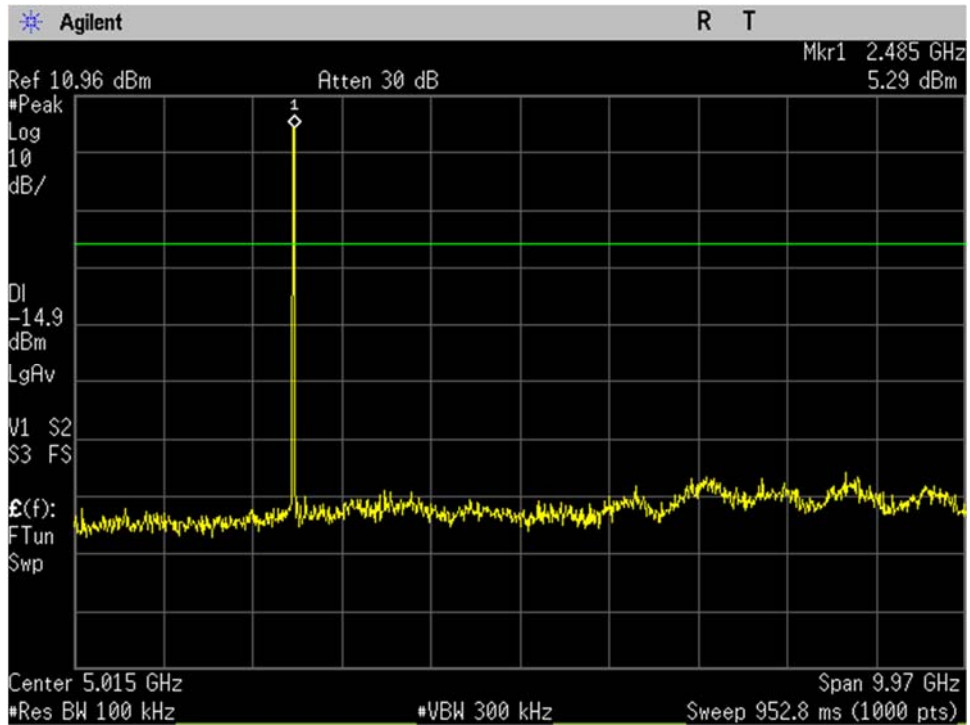
BLE_High Ch_2480MHz_1MBit_-20dBc_30MHz-10GHz_Port 1
