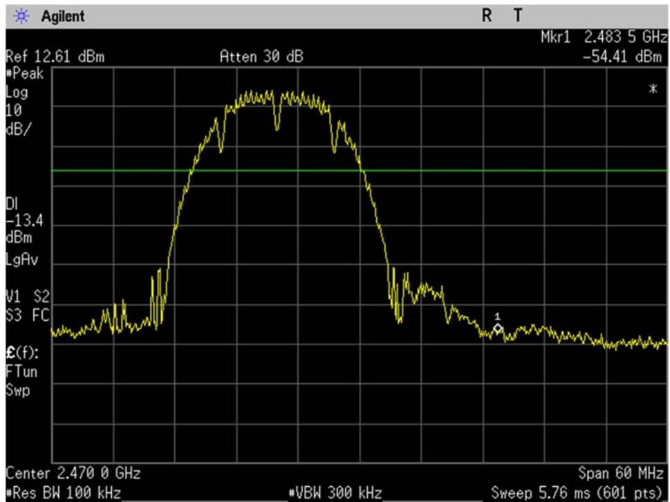
WIFI_High Ch_2462MHz_20MHz BW_b-mode_-20dBc_Upper Band Edge_Port 2
