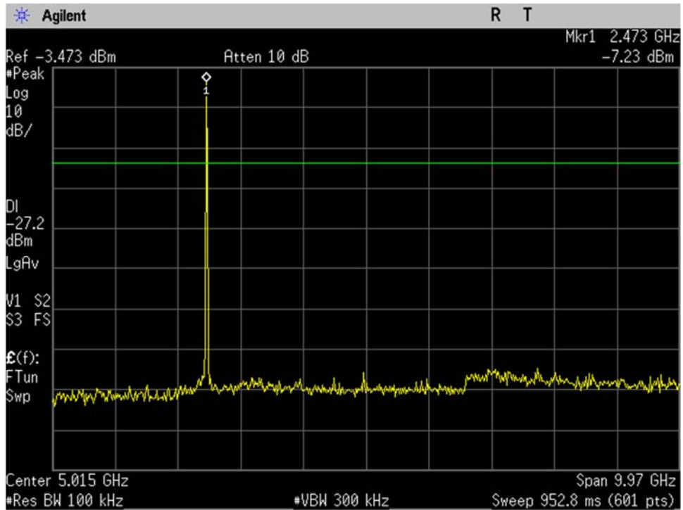
BLE_High Ch_2480MHz_2MBit_-20dBc_30MHz-10GHz_Port 1
