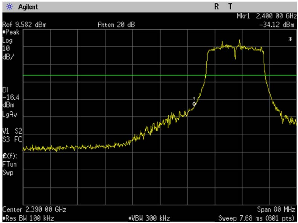
WIFI_Low Ch_2412MHz_20MHz BW_g-mode_-20dBc_Lower Band Edge_Port 2
