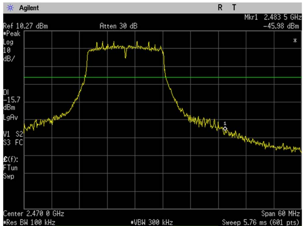
WIFI_High Ch_2462MHz_20MHz BW_g-mode_-20dBc_Upper Band Edge_Port 1
