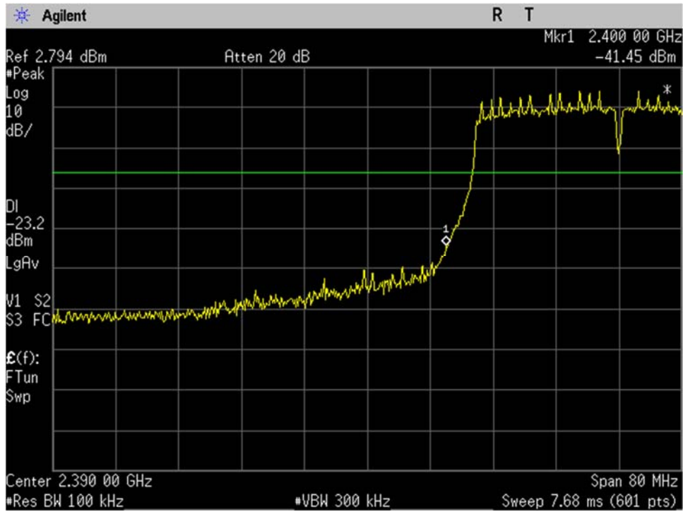
WIFI_Low Ch_2422MHz_40MHz BW_n-mode_-20dBc_Lower Band Edge_Port 2
