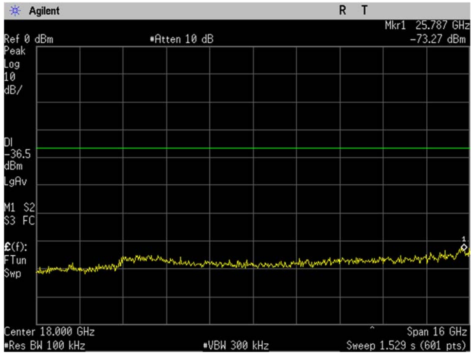
BLE_Mid Ch_2440MHz_2MBit_-20dBc_10-26GHz_Port 1
