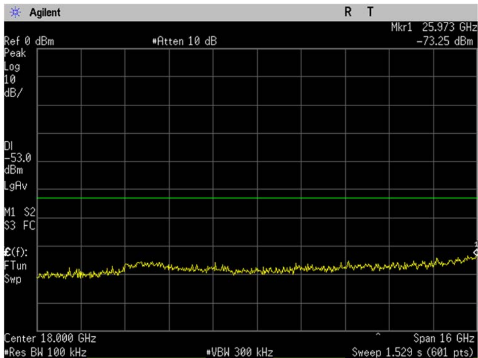
WIFI_Low Ch_2422MHz_40MHz BW_n-mode_-20dBc_10-26GHz_Port 1
