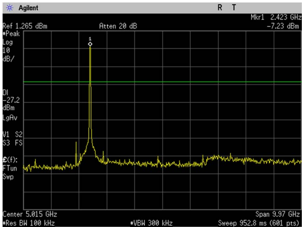
WIFI_Low Ch_2422MHz_40MHz BW_n-mode_-20dBc_30MHz-10GHz_Port 1
