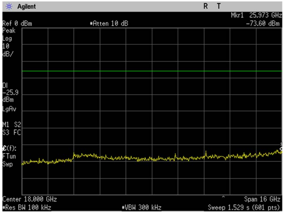
WIFI_Mid Ch_2437MHz_40MHz BW_n-mode_-20dBc_10-26GHz_Port 1
