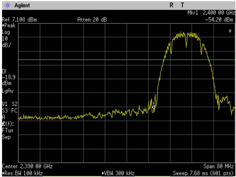
WIFI_Low Ch_2412MHz_20MHz BW_b-mode_-20dBc_Lower Band Edge_Port 1
