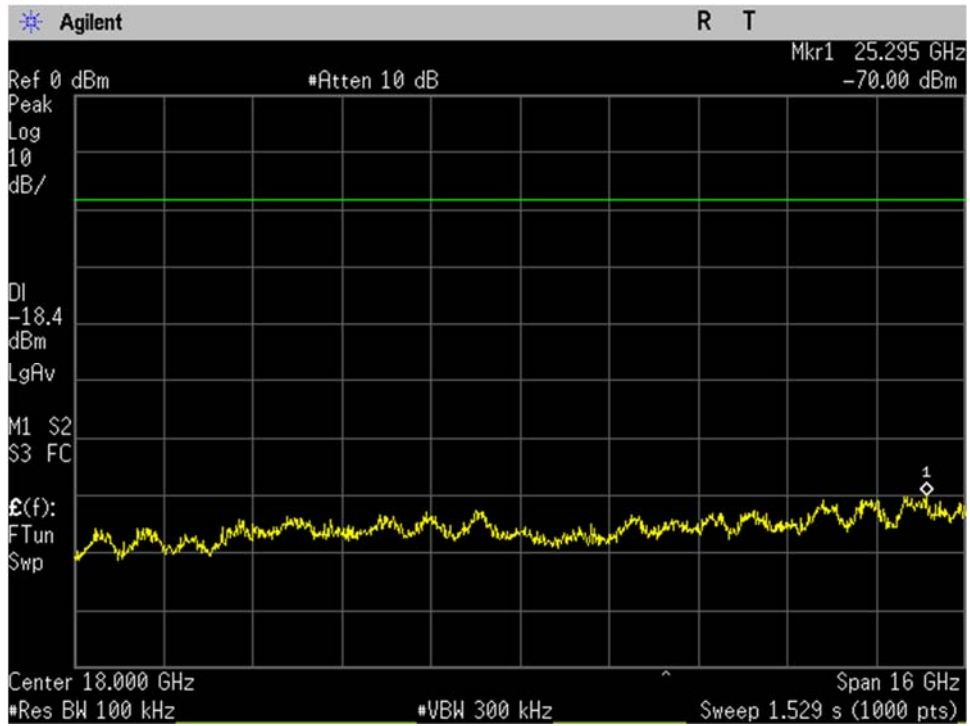
BLE_Mid Ch_2440MHz_1MBit_-20dBc_10-26GHz_Port 1
