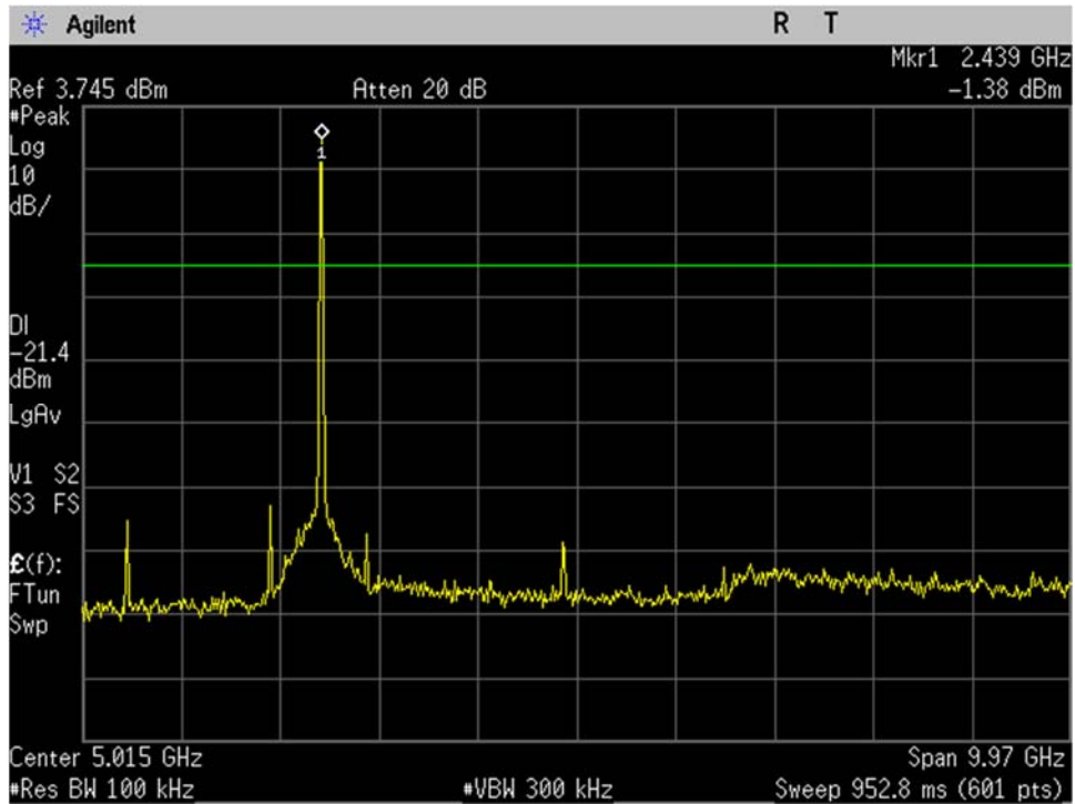
WIFI_Mid Ch_2437MHz_20MHz BW_g-mode_-20dBc_30MHz-10GHz_Port 2
