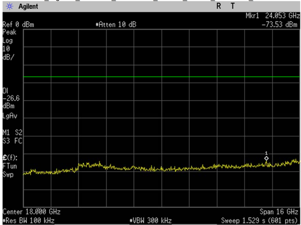
WIFI_High Ch_2452MHz_40MHz BW_n-mode_-20dBc_10-26GHz_Port 1
