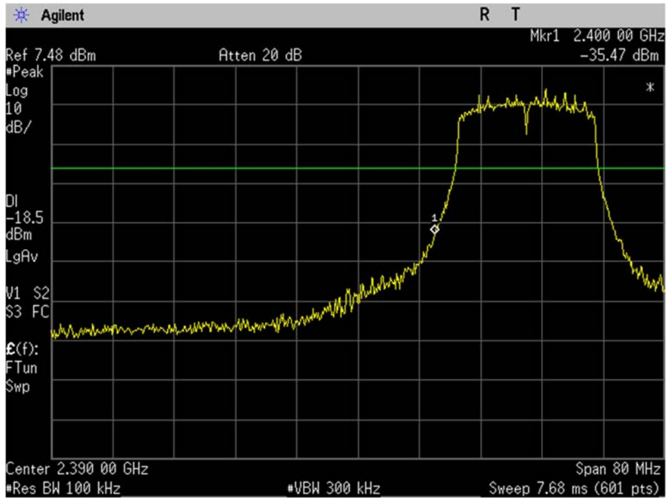
WIFI_Low Ch_2412MHz_20MHz BW_n-mode_-20dBc_Lower Band Edge_Port 2
