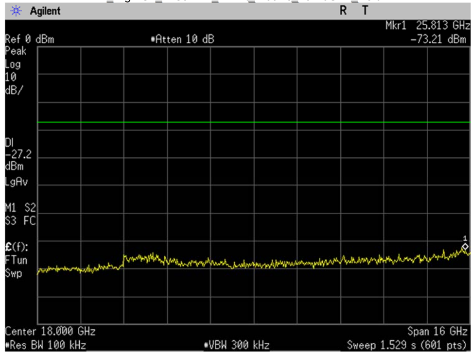
BLE_High Ch_2480MHz_2MBit_-20dBc_10-26GHz_Port 1
