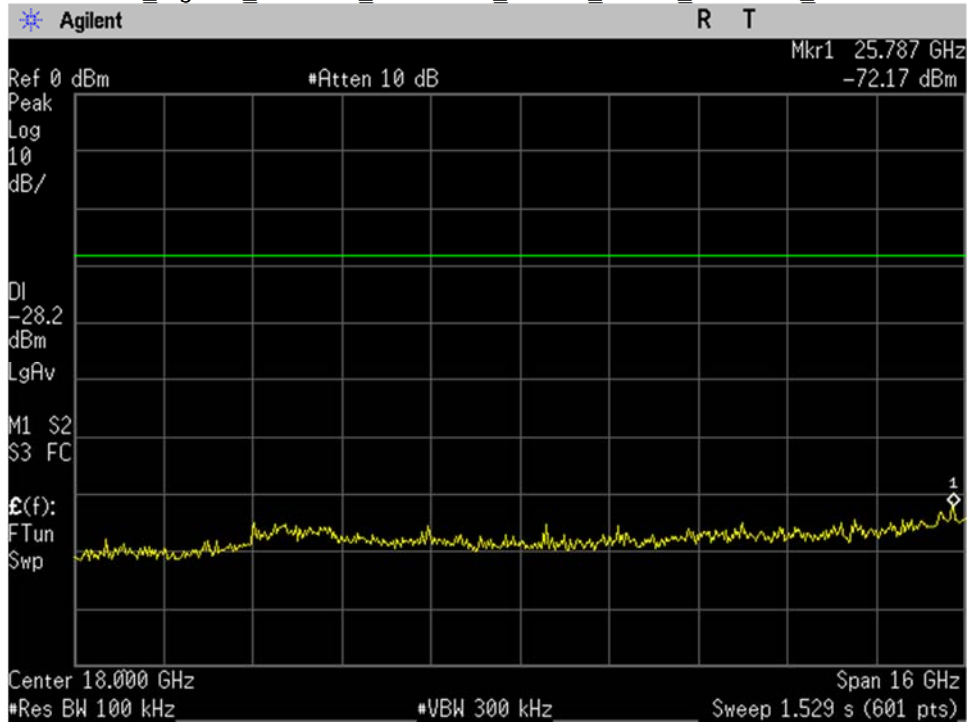
WIFI_High Ch_2452MHz_40MHz BW_n-mode_-20dBc_10-26GHz_Port 2
