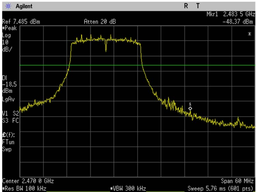
WIFI_High Ch_2462MHz_20MHz BW_n-mode_-20dBc_Upper Band Edge_Port 1
