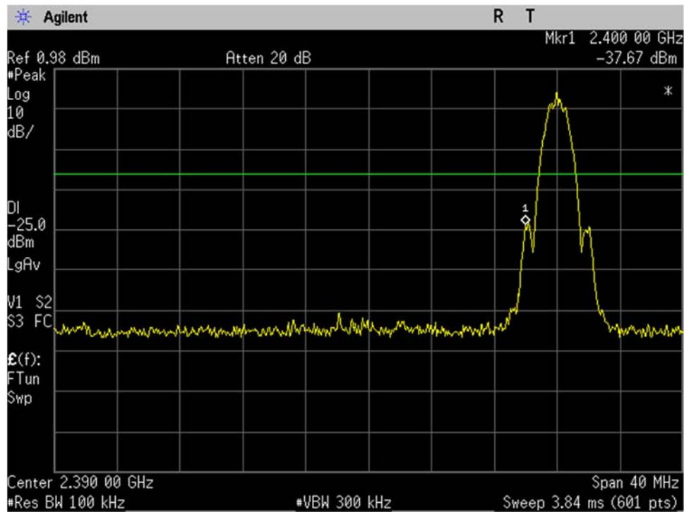
BLE_Low Ch_2402MHz_2MBit_-20dBc_Lower Band Edge_Port 1
