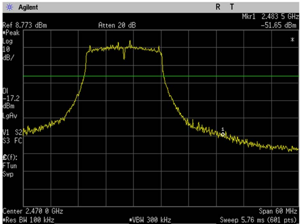
WIFI_High Ch_2462MHz_20MHz BW_g-mode_-20dBc_Upper Band Edge_Port 2
