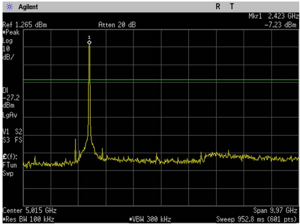
WIFI_Low Ch_2422MHz_40MHz BW_n-mode_-20dBc_30MHz-10GHz_Port 2
