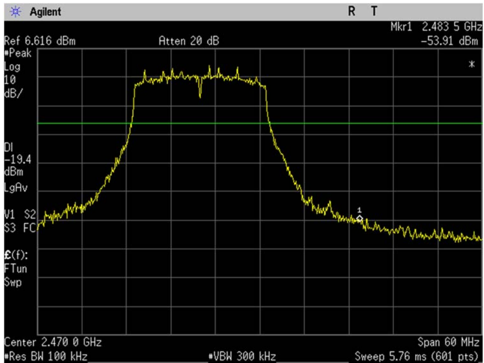
WIFI_High Ch_2462MHz_20MHz BW_n-mode_-20dBc_Upper Band Edge_Port 2
