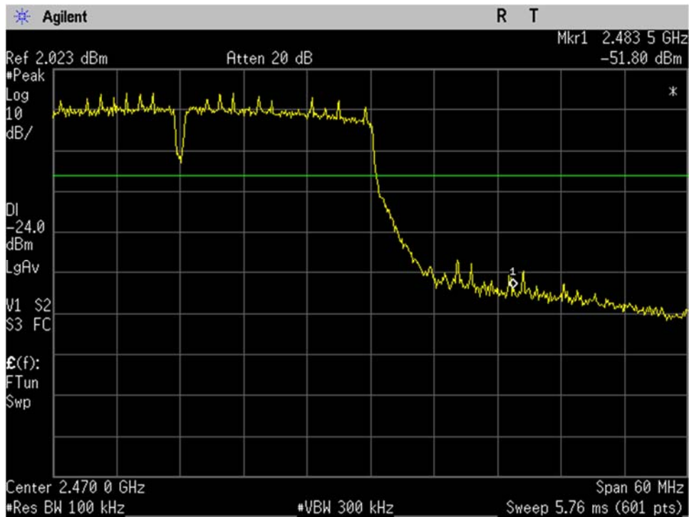
WIFI_High Ch_2452MHz_40MHz BW_n-mode_-20dBc_Upper Band Edge_Port 2
