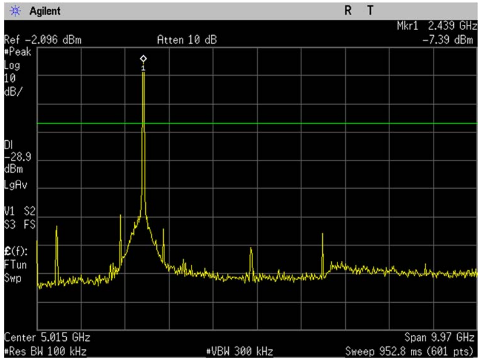
WIFI_Mid Ch_2437MHz_40MHz BW_n-mode_-20dBc_30MHz-10GHz_Port 2
