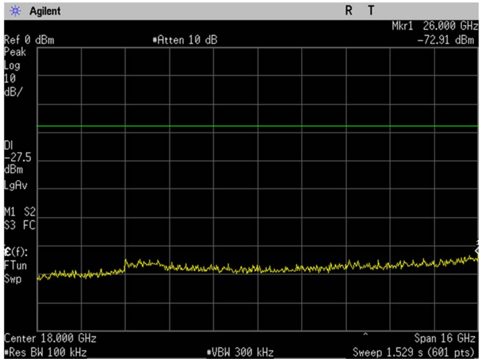
BLE_Low Ch_2402MHz_2MBit_-20dBc_10-26GHz_Port 1
