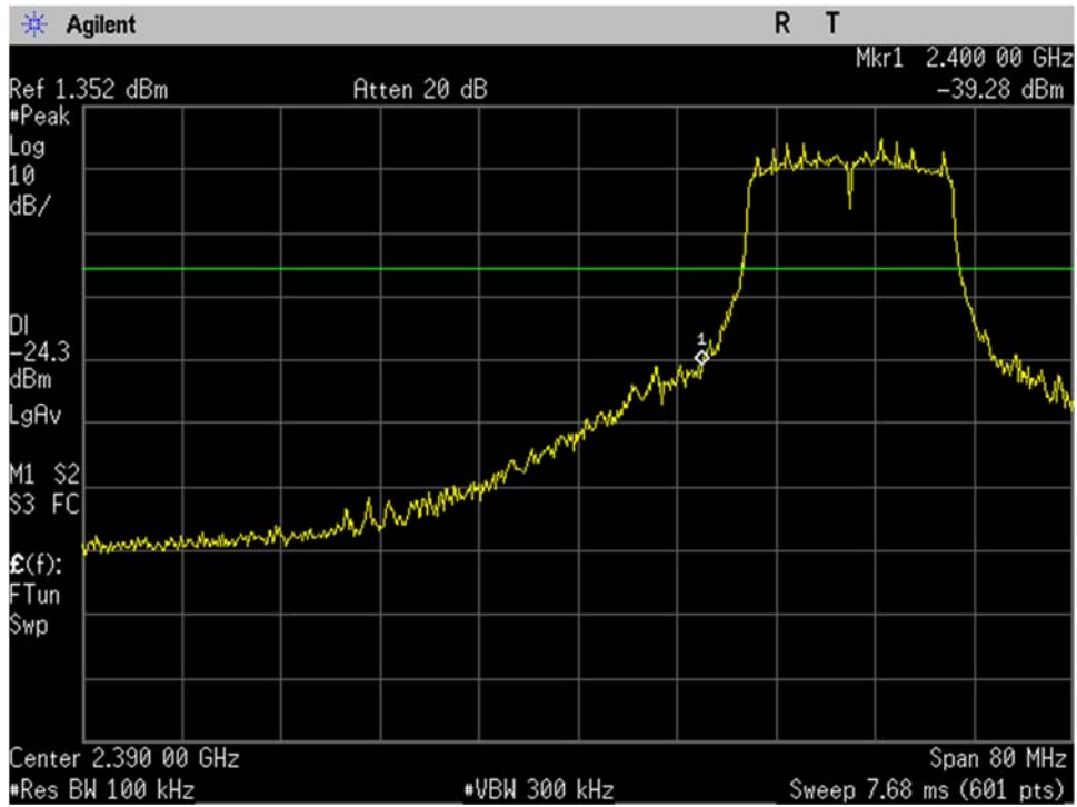
WIFI_Low Ch_2412MHz_20MHz BW_g-mode_-20dBc_Lower Band Edge_Port 1
