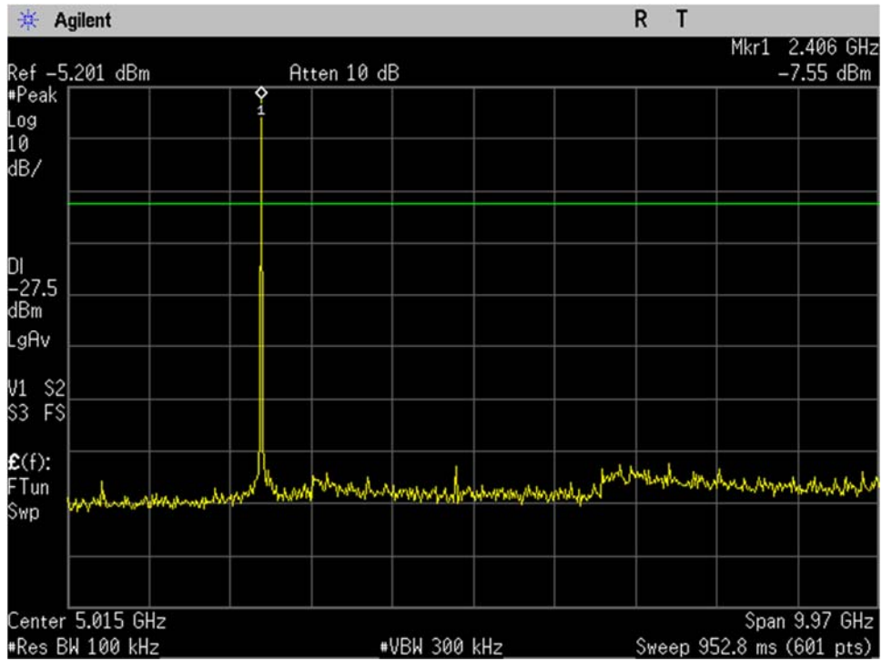
BLE_Low Ch_2402MHz_2MBit_-20dBc_30MHz-10GHz_Port 1
