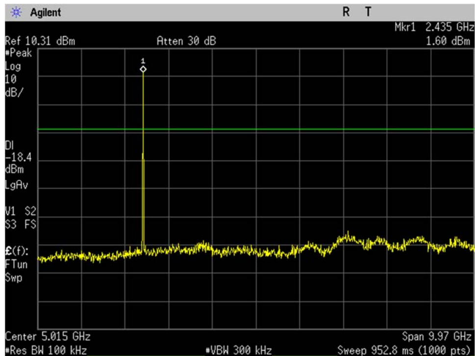
BLE_Mid Ch_2440MHz_1MBit_-20dBc_30MHz-10GHz_Port 1
