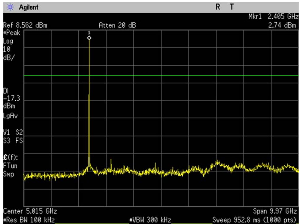
BLE_Low Ch_2402MHz_1MBit_-20dBc_30MHz-10GHz_Port 1
