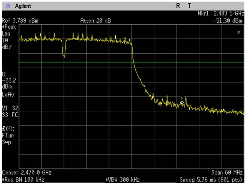
WIFI_High Ch_2452MHz_40MHz BW_n-mode_-20dBc_Upper Band Edge_Port 1
