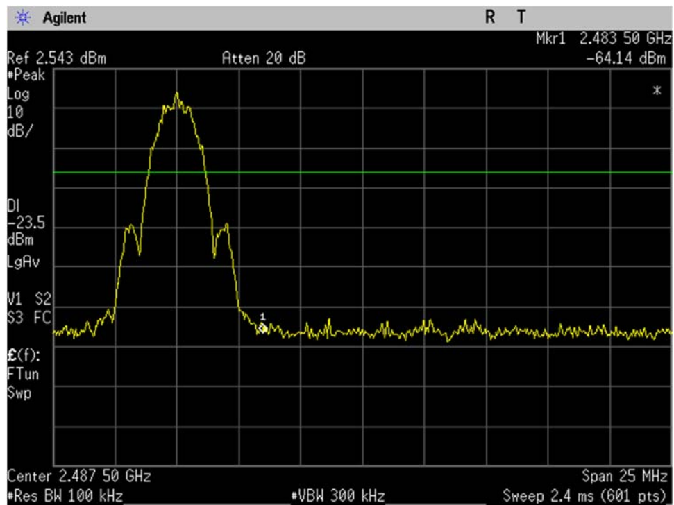
BLE_High Ch_2480MHz_2MBit_-20dBc_Upper Band Edge_Port 1
