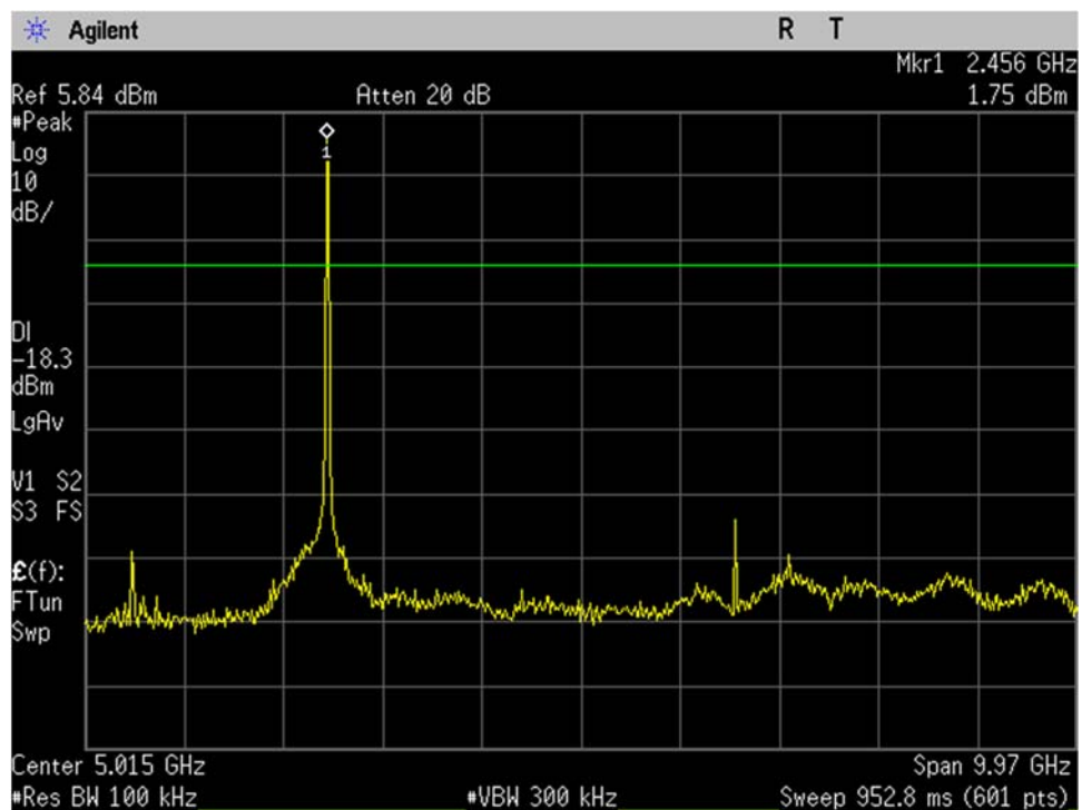
WIFI_High Ch_2462MHz_20MHz BW_g-mode_-20dBc_30MHz-10GHz_Port 1
