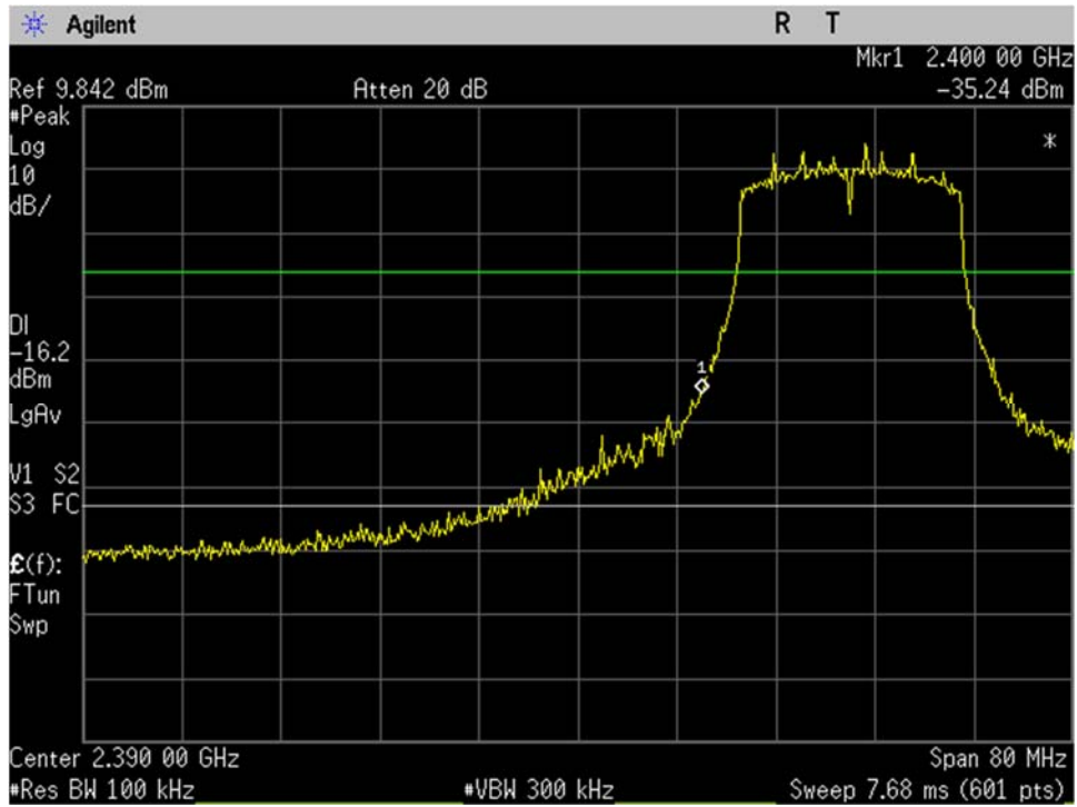
WIFI_Low Ch_2412MHz_20MHz BW_n-mode_-20dBc_Lower Band Edge_Port 1
