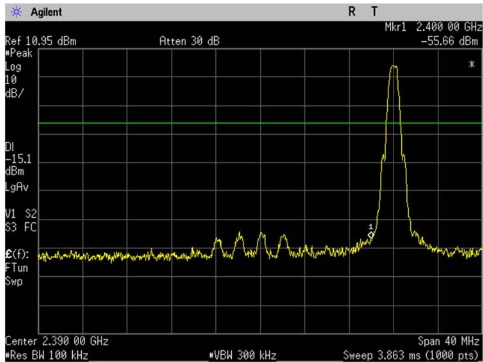
BLE_Low Ch_2402MHz_1MBit_-20dBc_Lower Band Edge_Port 1
