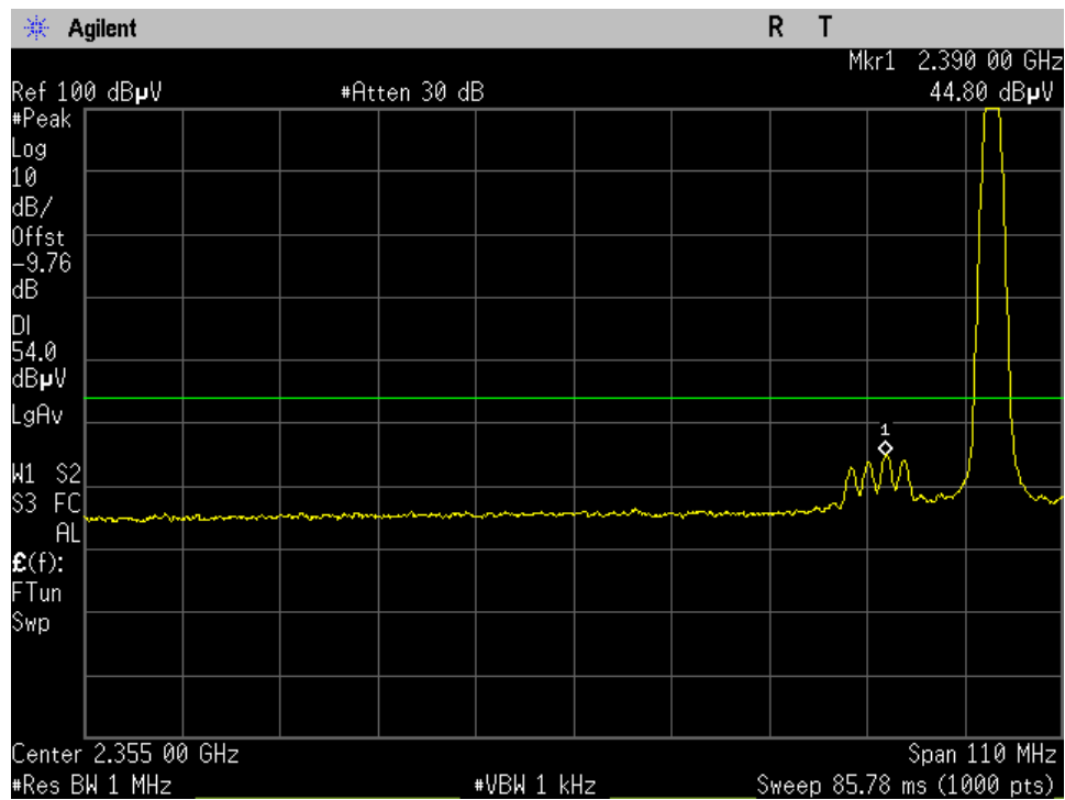
Low Ch_2402MHz_GFSK_15.209_Lower Band Edge Avg_Port 1
