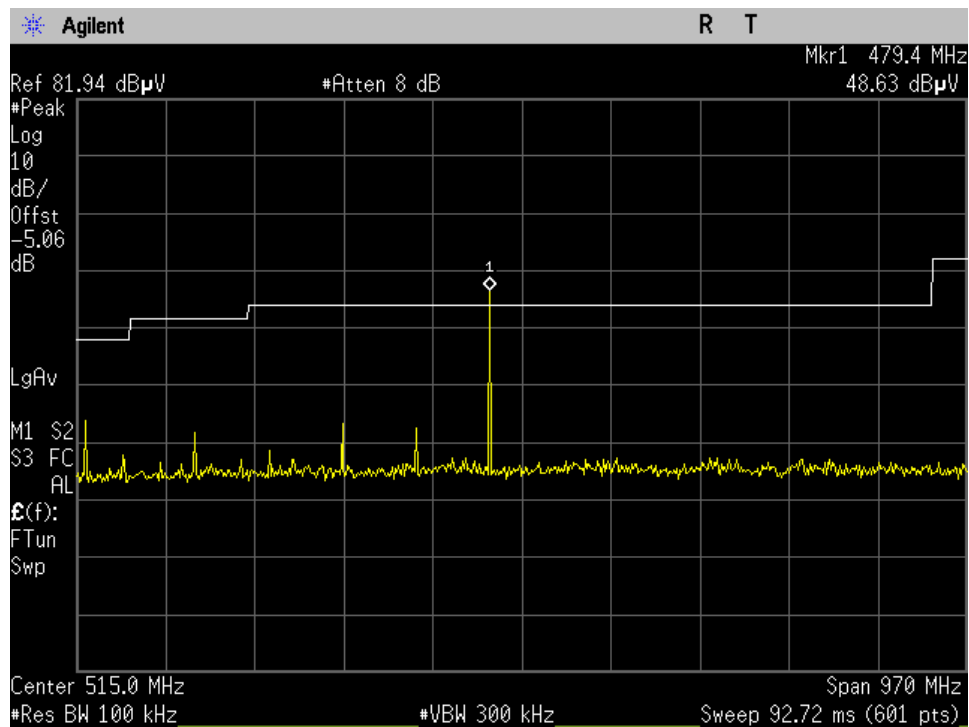
Mid Ch_2440MHz_GFSK_15.209_30-1000MHz_Peak_Port 1
