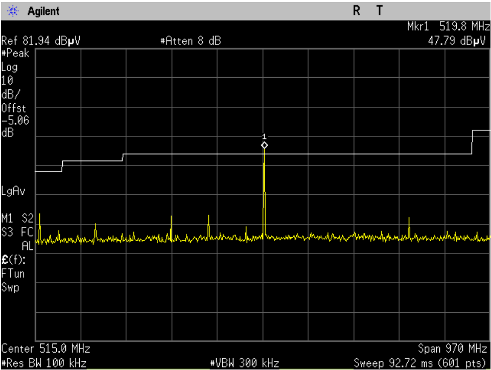
High Ch_2480MHz_GFSK_15.209_30-1000MHz_Peak_Port 1
