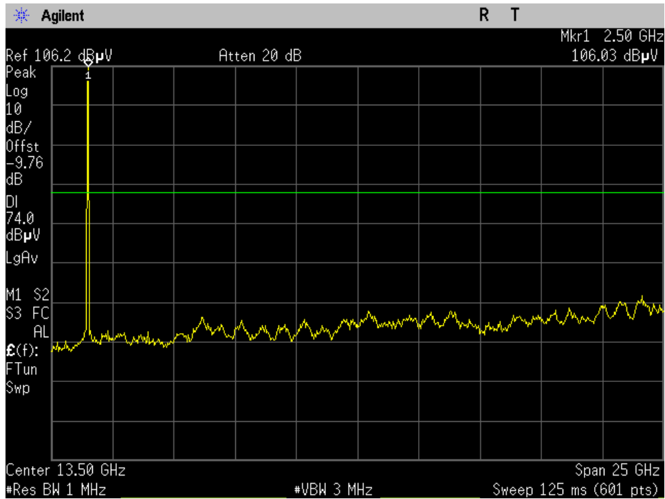
High Ch_2480MHz_Pi_4DQPSK_15.209_1-26GHz_Peak_Port 1
