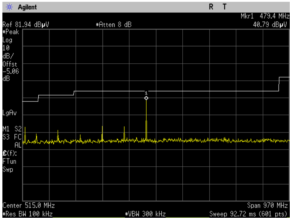
Mid Ch_2440MHz_Pi_4DQPSK_15.209_30-1000MHz_Peak_Port 1
