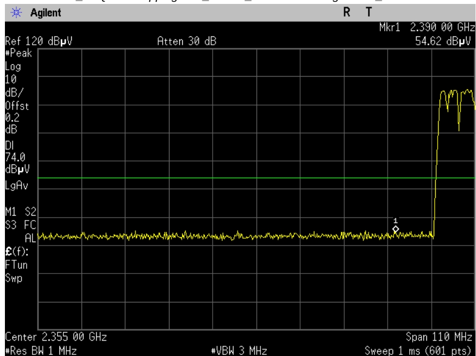
Pi_4DQPSK Hopping Low_15.209_Lower Band Edge Peak_Port 1
