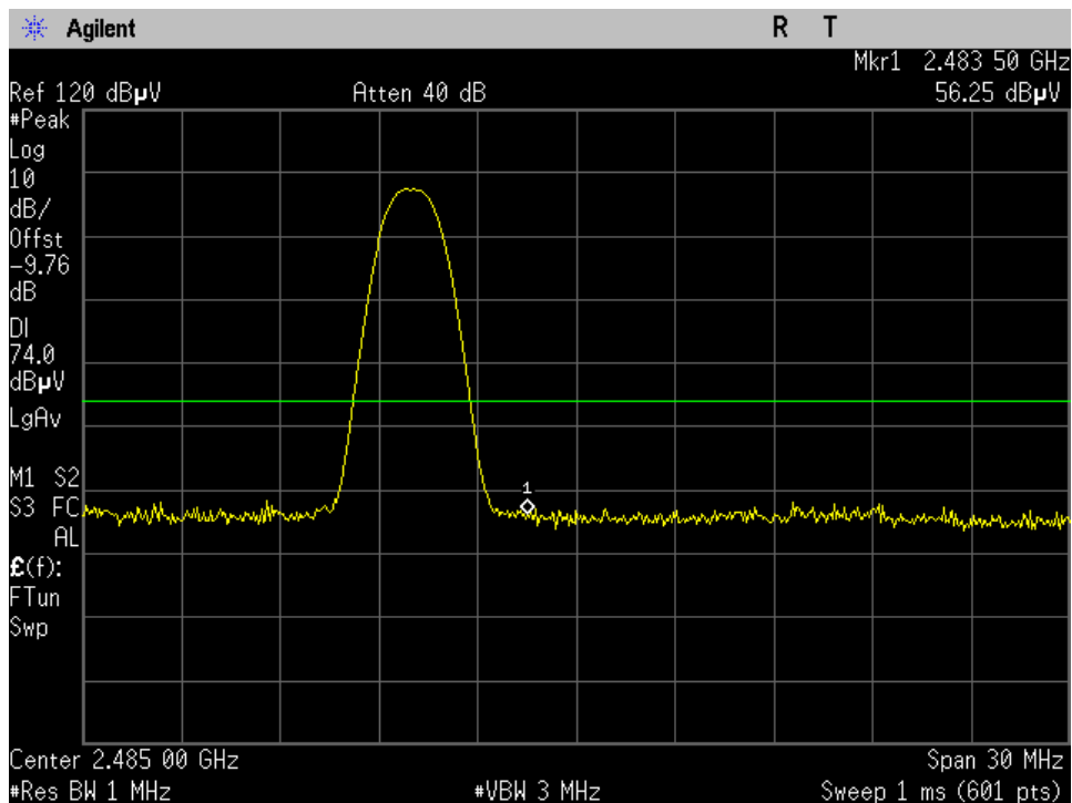
High Ch_2480MHz_GFSK_15.209_Upper Band Edge Peak_Port 1
