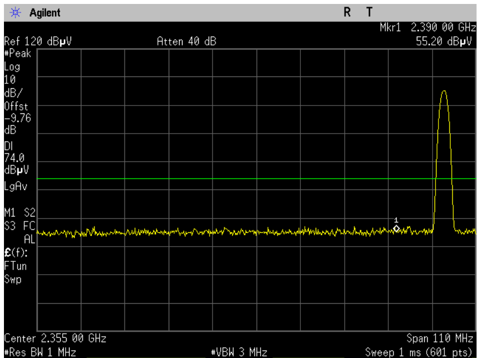
Low Ch_2402MHz_Pi_4DQPSK_15.209_Lower Band Edge Peak_Port 1
