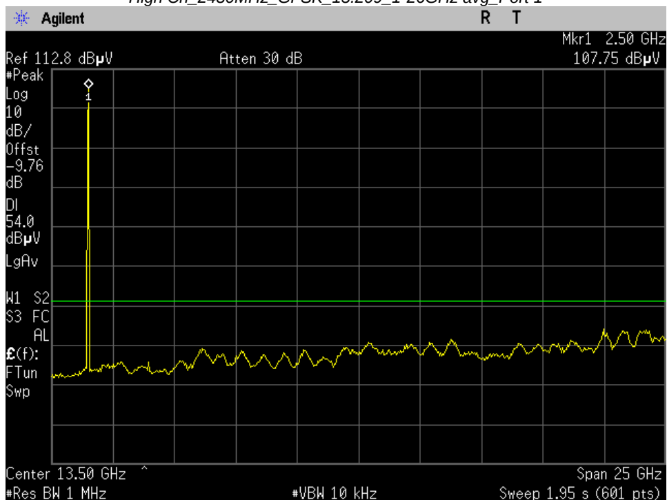
High Ch_2480MHz_GFSK_15.209_1-26GHz avg_Port 1
