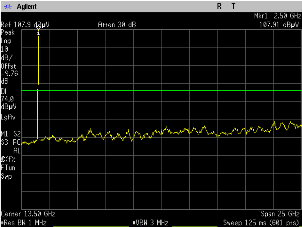
High Ch_2480MHz_GFSK_15.209_1-26GHz_Peak_Port 1
