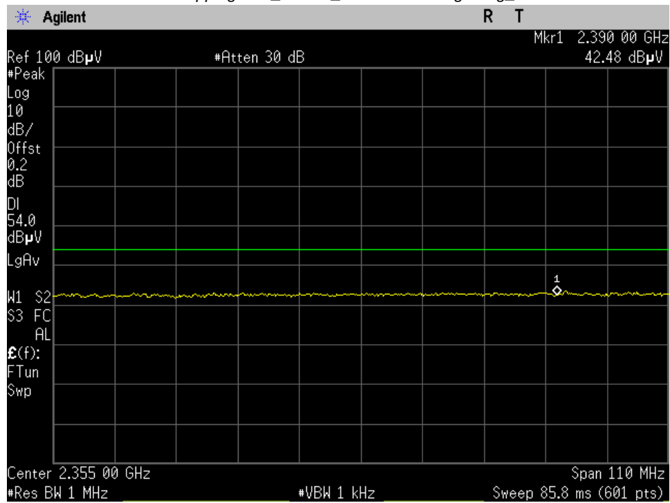
8DPSK Hopping Low_15.209_Lower Band Edge Avg_Port 1
