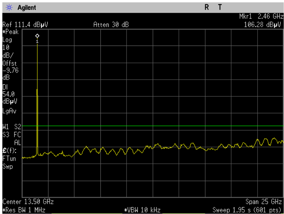
Mid Ch_2440MHz_GFSK_15.209_1-26GHz avg_Port 1
