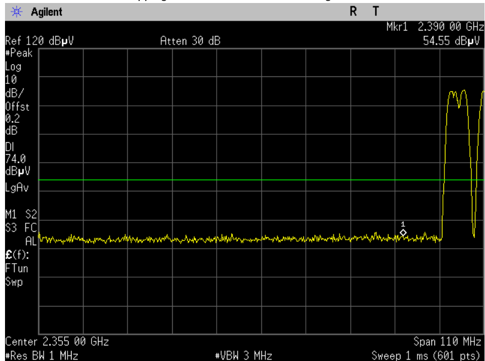
8DPSK Hopping Low_15.209_Lower Band Edge Peak_Port 1
