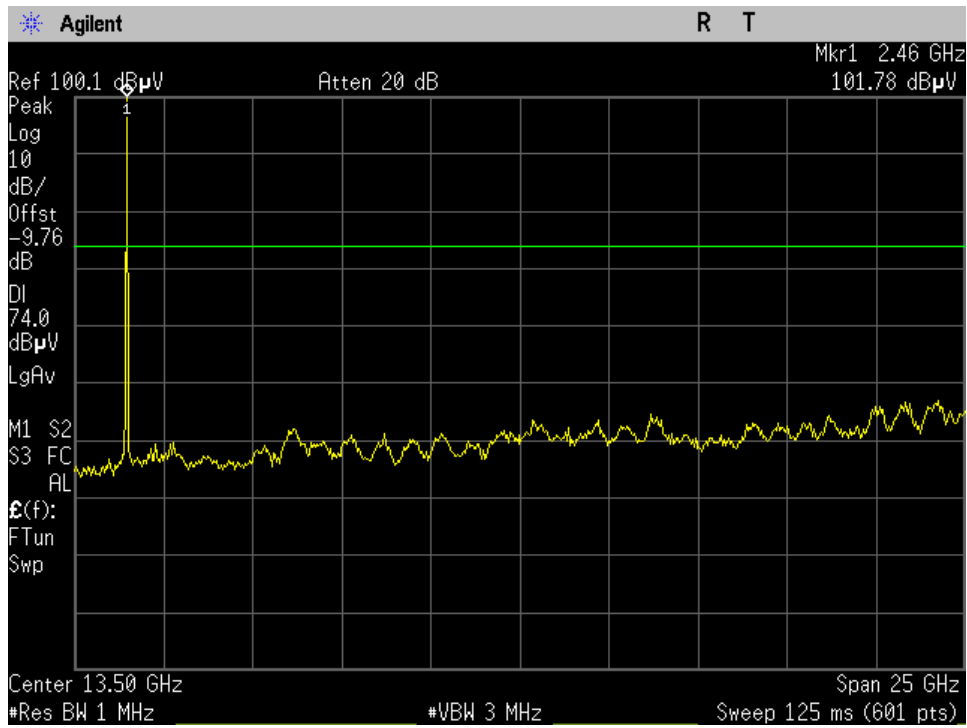
Mid Ch_2440MHz_8DPSK_15.209_1-26GHz _Peak_Port 1
