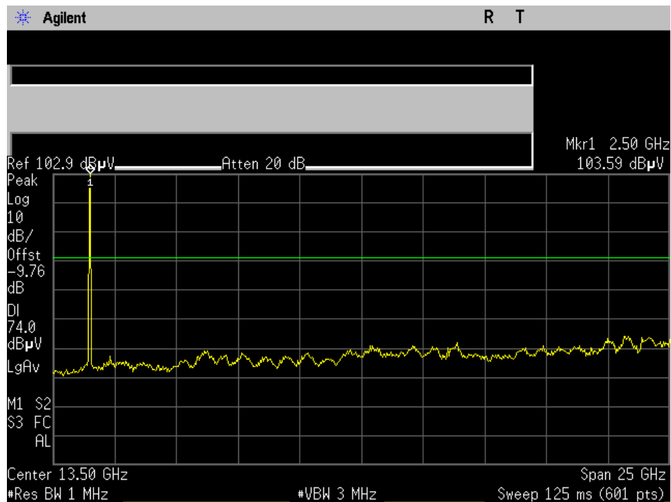
High Ch_2480MHz_8DPSK_15.209_1-26GHz_Peak_Port 1
