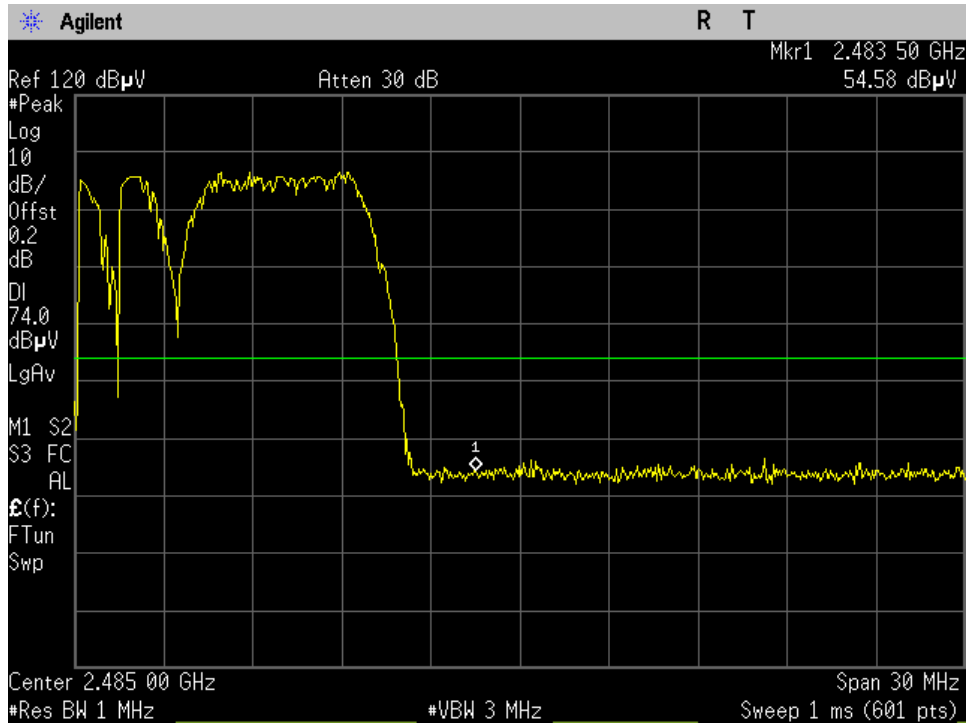
Pi_4DQPSK Hopping High_15.209_Upper Band Edge Peak_Port 1
