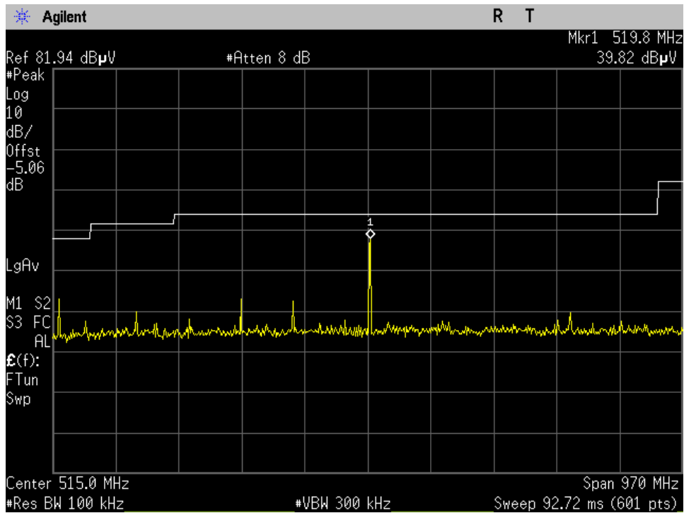
High Ch_2480MHz_Pi_4DQPSK_15.209_30-1000MHz_Peak_Port 1
