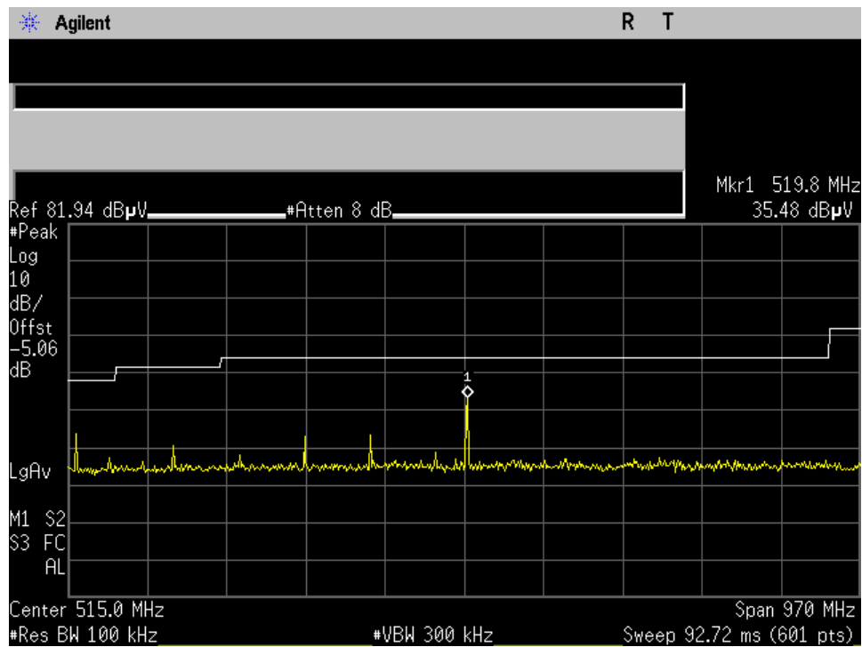
High Ch_2480MHz_8DPSK_15.209_30-1000MHz_Peak_Port 1
