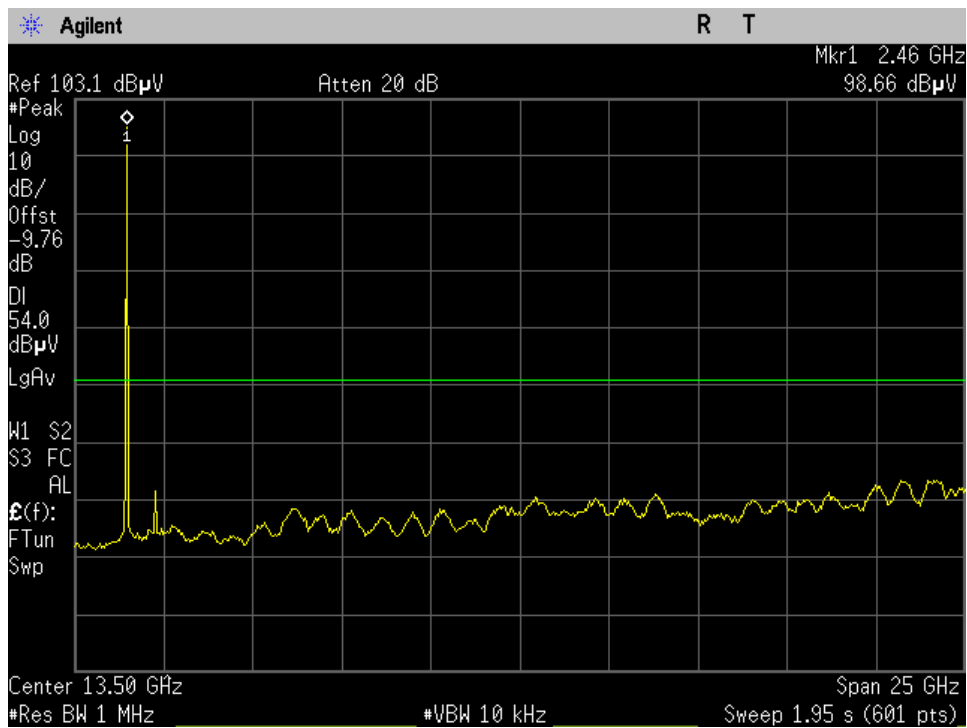
Mid Ch_2440MHz_8DPSK_15.209_1-26GHz avg_Port 1
