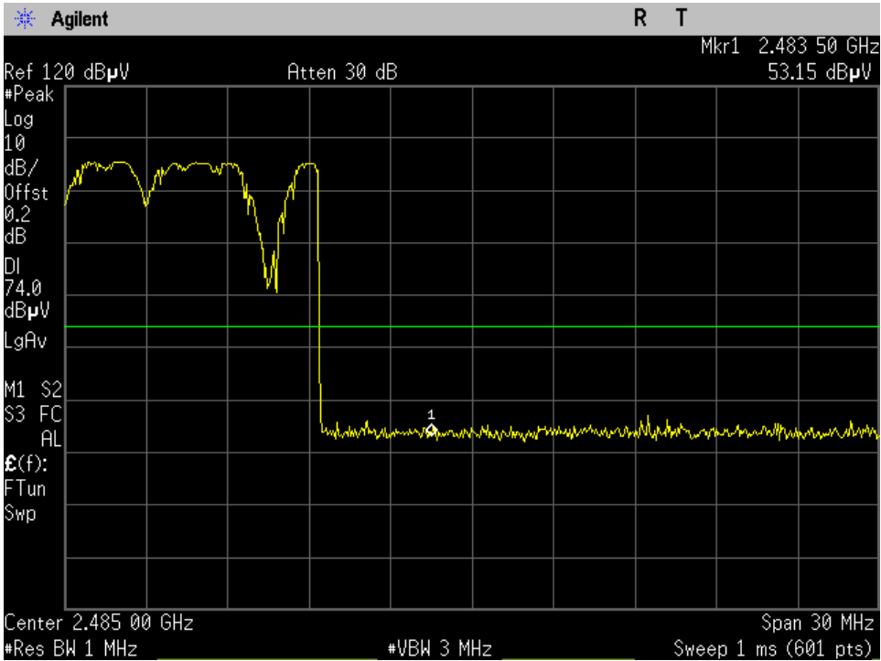
GFSK Hopping High_15.209_Upper Band Edge Peak_Port 1
