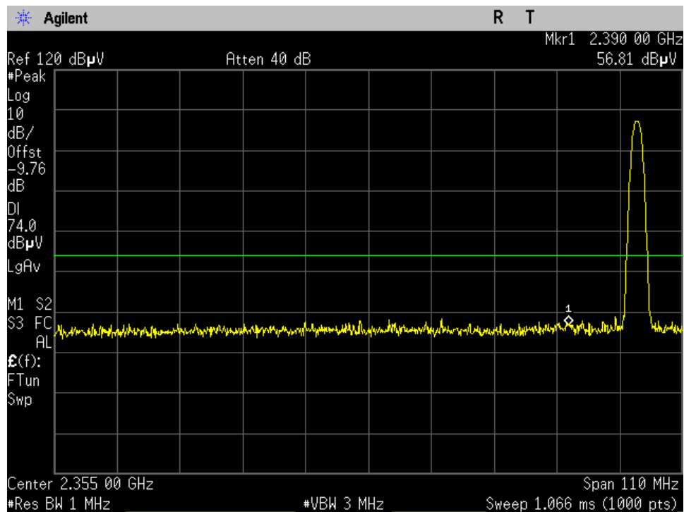
Low Ch_2402MHz_GFSK_15.209_Lower Band Edge Peak_Port 1
