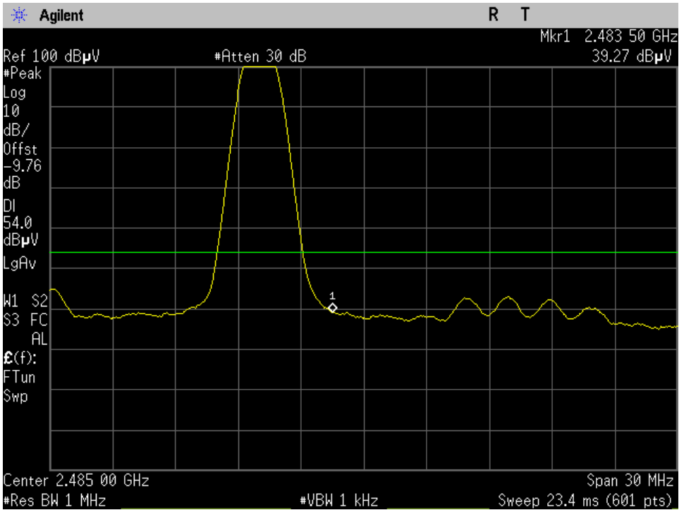
High Ch_2480MHz_GFSK_15.209_Upper Band Edge Avg_Port 1
