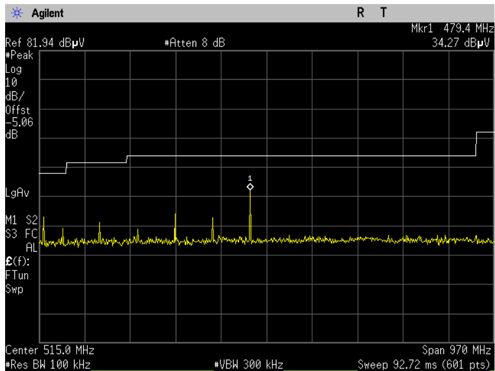
Mid Ch_2440MHz_8DPSK_15.209_30-1000MHz_Peak_Port 1
