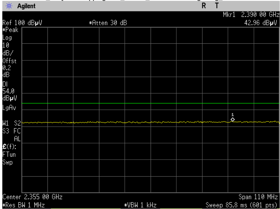
Pi_4DQPSK Hopping Low_15.209_Lower Band Edge Avg_Port 1
