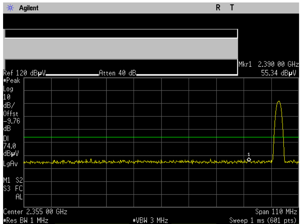
Low Ch_2402MHz_8DPSK_15.209_Lower Band Edge Peak_Port 1
