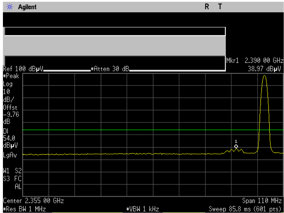
Low Ch_2402MHz_8DPSK_15.209_Lower Band Edge Avg_Port 1
