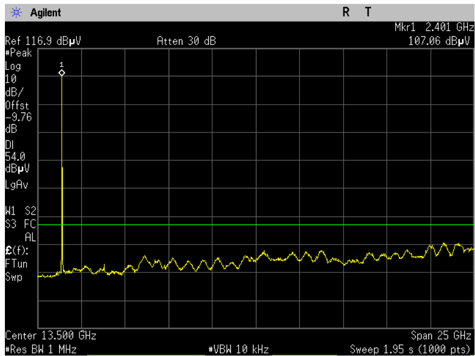
Low Ch_2402MHz_GFSK_15.209_1-26GHz avg_Port 1
