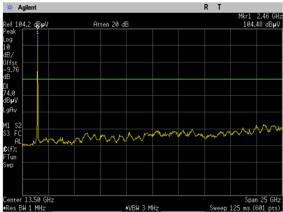
Mid Ch_2440MHz_Pi_4DQPSK_15.209_1-26GHz_Peak_Port 1
