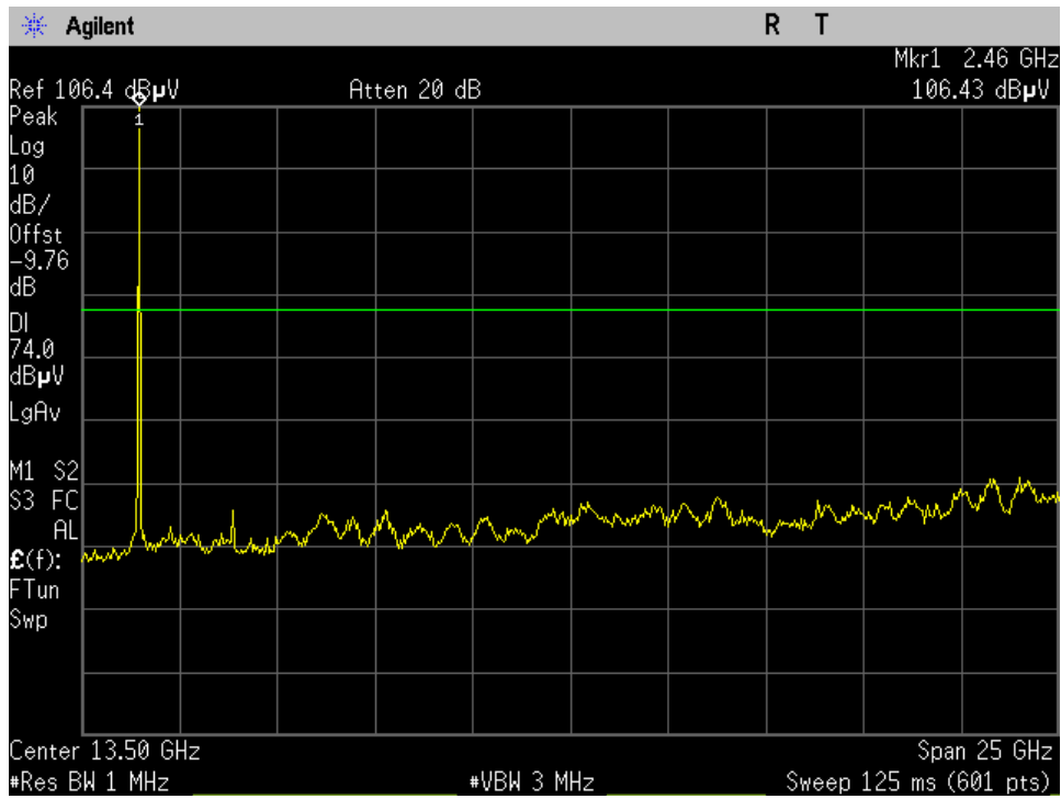
Mid Ch_2440MHz_GFSK_15.209_1-26GHz_Peak_Port 1
