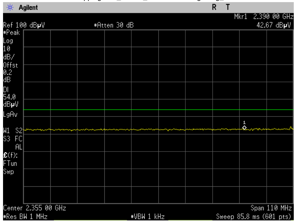
GFSK Hopping Low_15.209_Lower Band Edge Avg_Port 1
