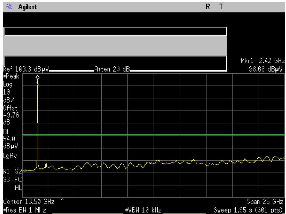
Low Ch_2402MHz_8DPSK_15.209_1-26GHz avg_Port 1
