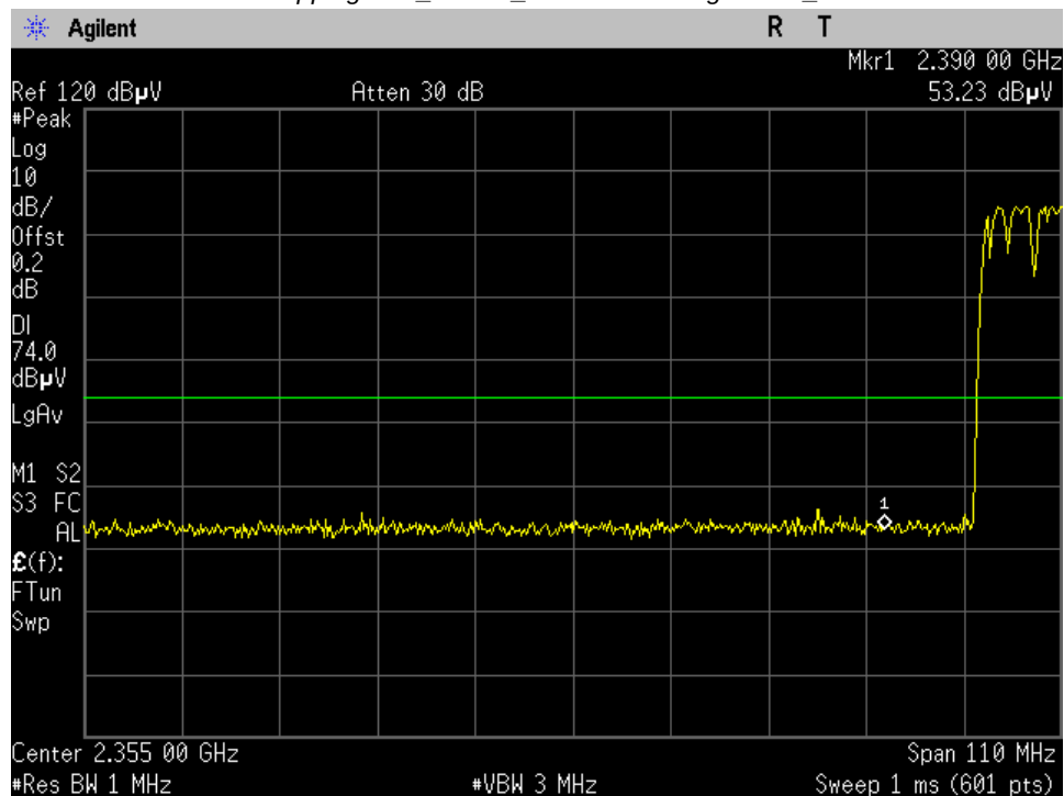
GFSK Hopping Low_15.209_Lower Band Edge Peak_Port 1
