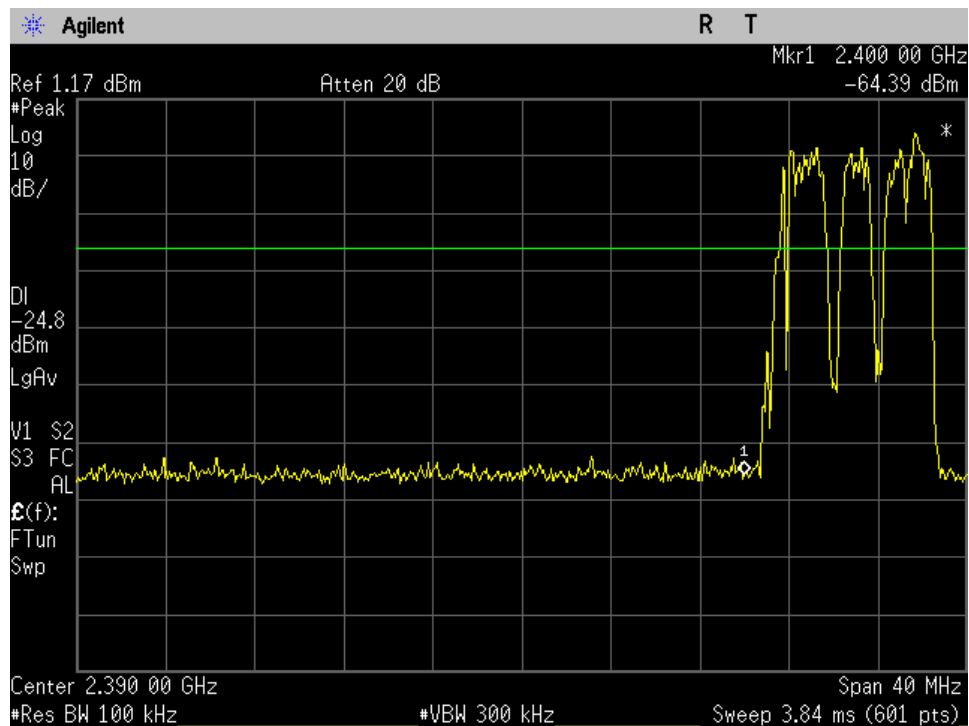
Pi_4DQPSK Hopping Low_-20dBc_Lower Band Edge_Port 1
