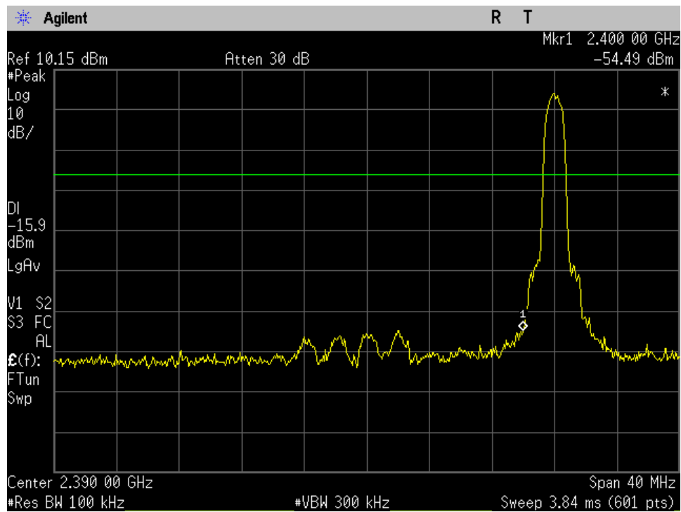
Low Ch_2402MHz_Pi_4DQPSK_-20dBc_Lower Band Edge_Port 1
