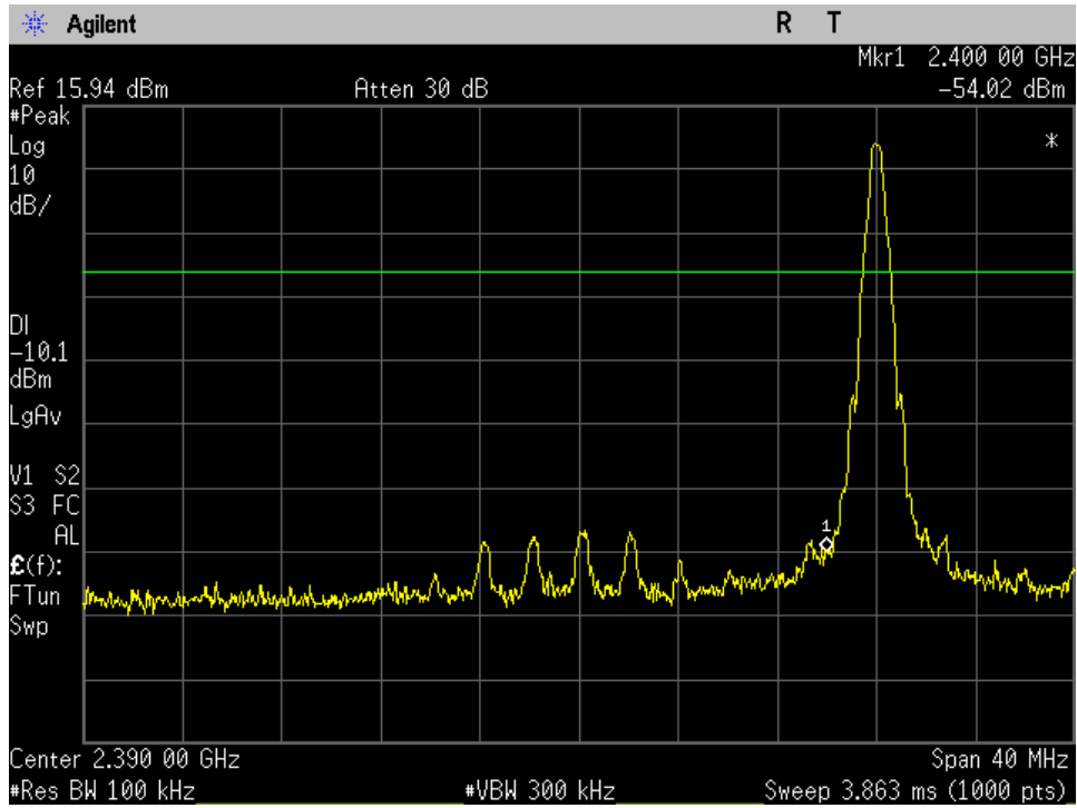
Low Ch_2402MHz_GFSK_-20dBc_Lower Band Edge_Port 1
