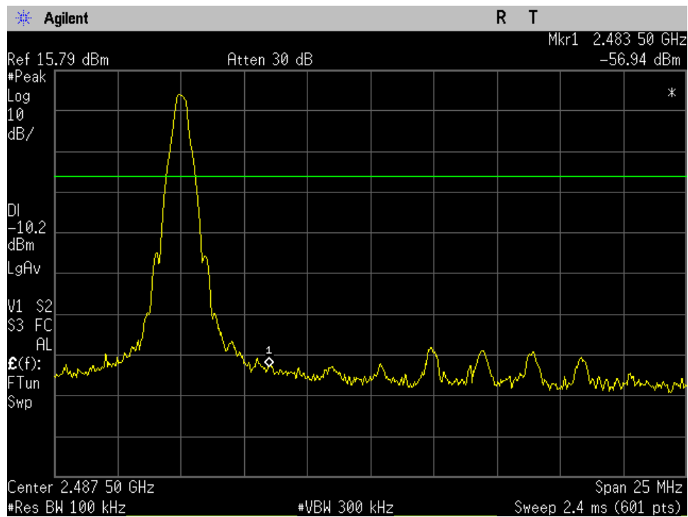
GFSK Hopping High_-20dBc_Upper Band Edge_Port 1
