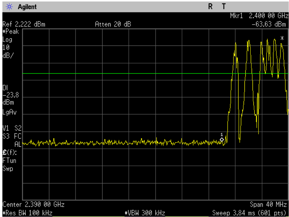
GFSK Hopping Low_-20dBc_Lower Band Edge_Port 1
