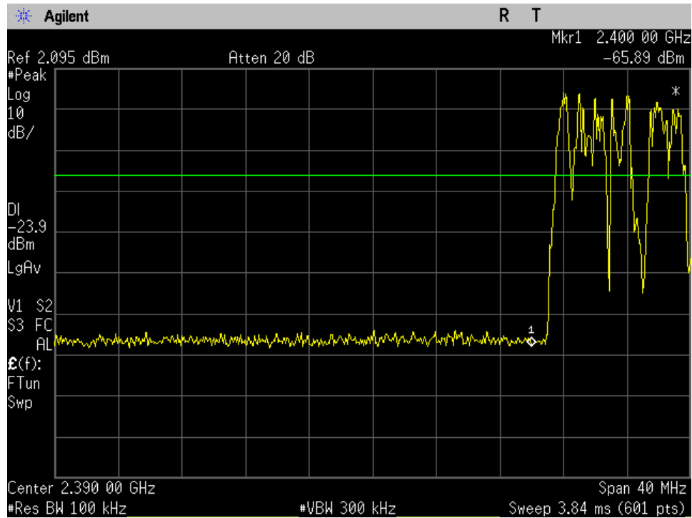
8DPSK Hopping Low_-20dBc_Lower Band Edge_Port 1
