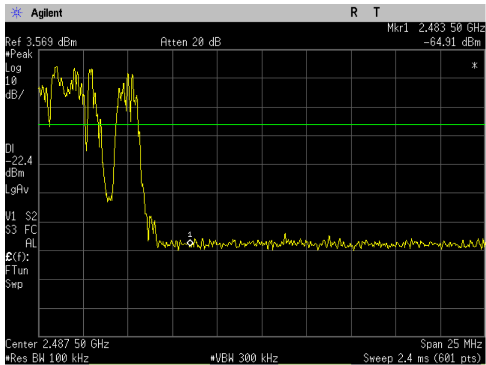
8DPSK Hopping High_-20dBc_Upper Band Edge_Port 1
