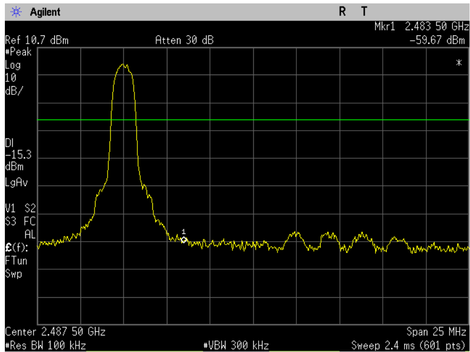
High Ch_2480MHz_Pi_4DQPSK_-20dBc_Upper Band Edge_Port 1
