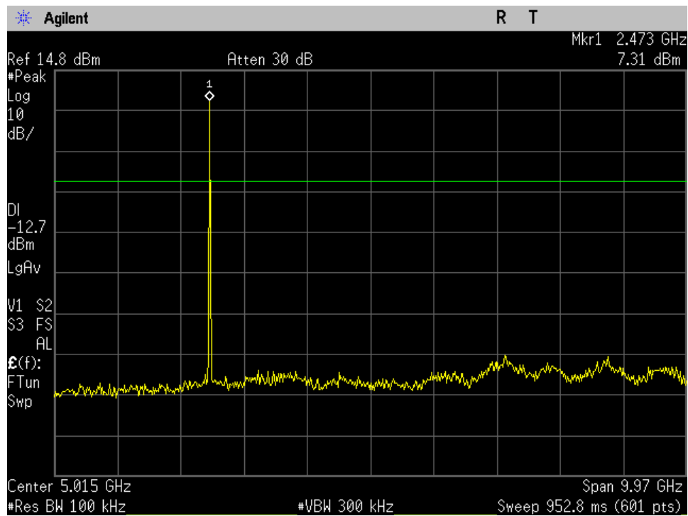
High Ch_2480MHz_GFSK_-20dBc_30MHz-10GHz_Port 1
