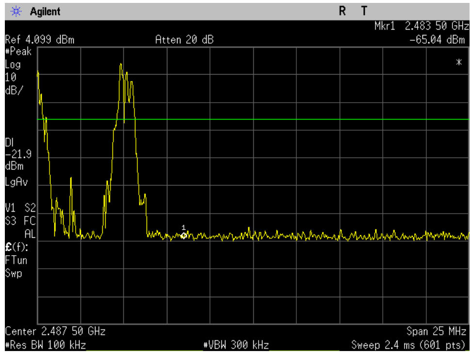
Pi_4DQPSK Hopping High_-20dBc_Upper Band Edge_Port 1
