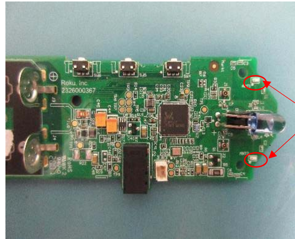
Main Board Antenna View
