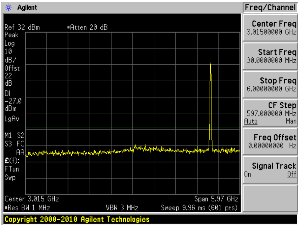
ANT A a Mode 5180 MHz Low Channel Spurious Emission_2
