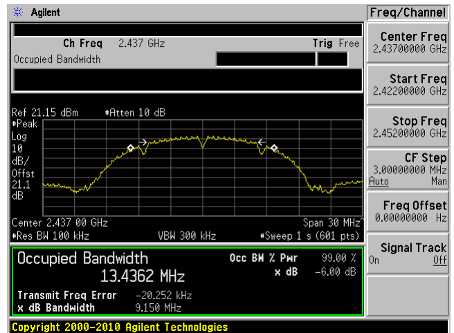
Mid Channel 6 dB OBW Antenna B
