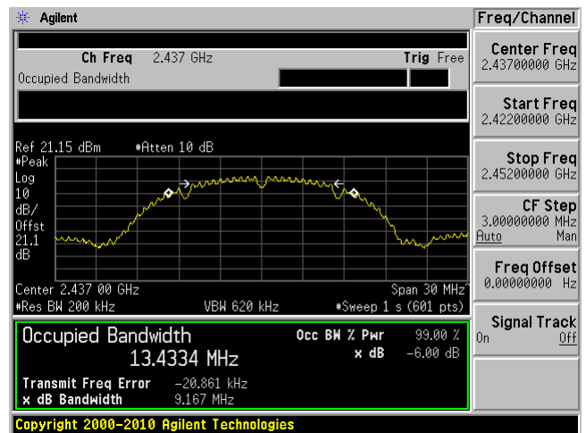
Mid Channel 99% OBW Antenna B
