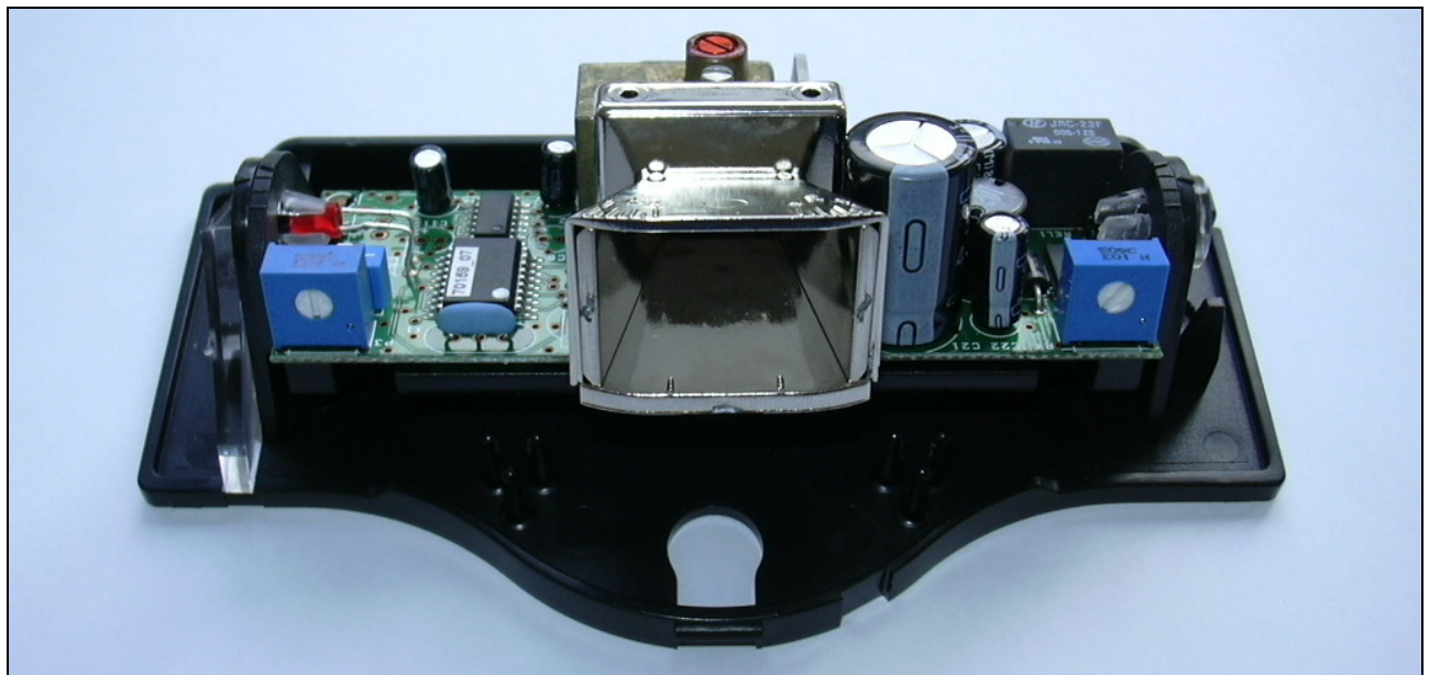
Photo 3: Component placement on the chassis
