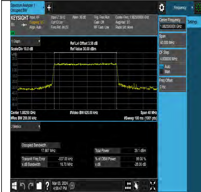
NTNV-N25-PC3-15-20-M-DFT-64QAM-Outer_Full-Ant0-PAS S
