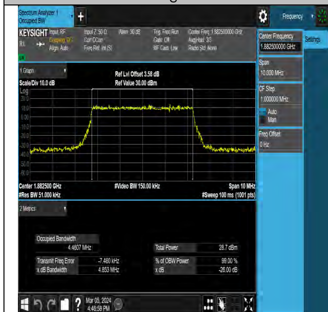
NTNV-N25-PC3-15-5-M-DFT-16QAM-Outet_Full-Ant0-PASS
