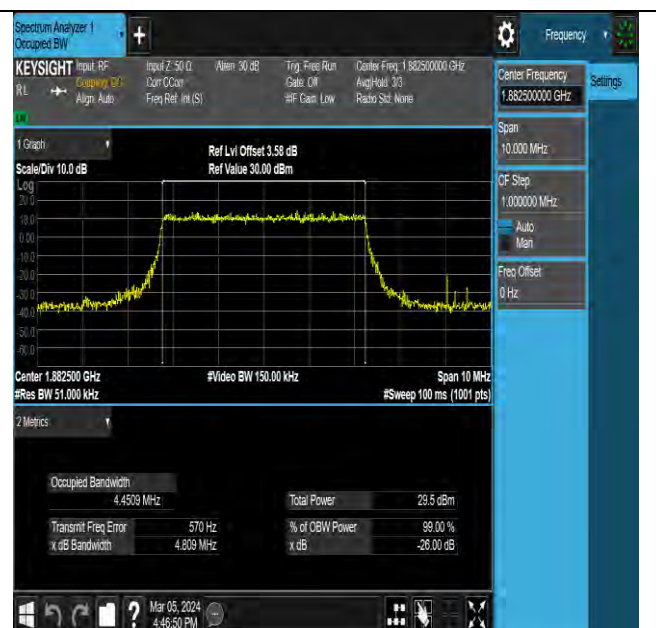
NTNV-N25-PC3-15-5-M-DFT-QPSK-Outet_Full-Ant0-PASS
