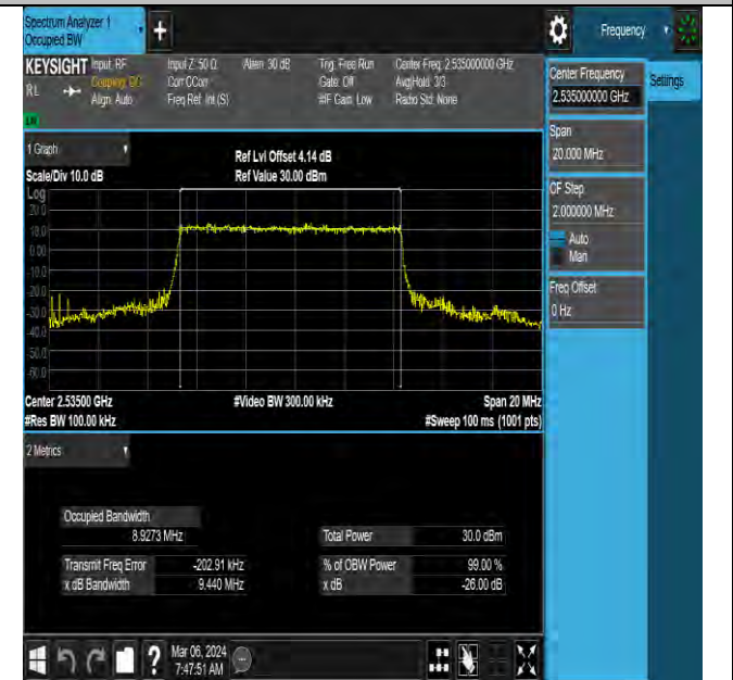
NTNV-N7-PC3-15-10-M-DFT-16QAM-Outer_Full-Ant0-PASS
