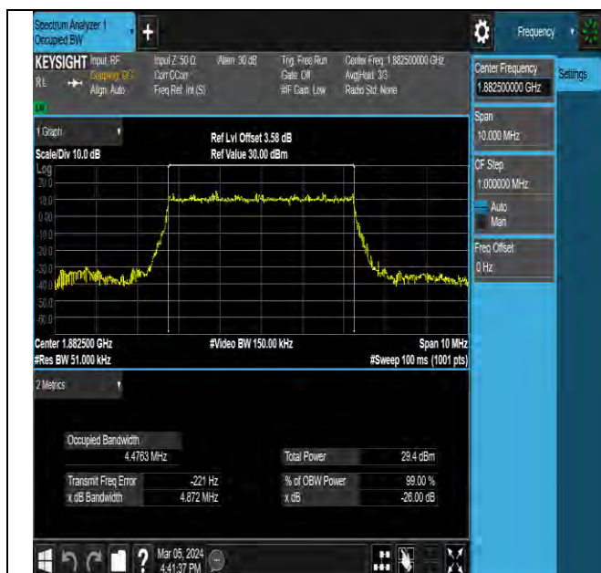
NTNV-N25-PC3-15-5-M-DFT-PI2BPSK-Outet_Full-Ant0-PASS S
