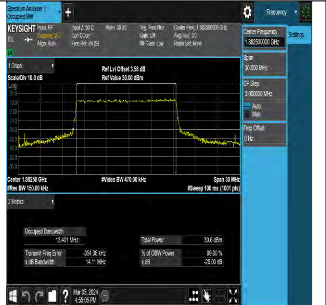
NTNV-N25-PC3-15-15-M-DFT-QPSK-Outer_Full-Ant0-PASS
