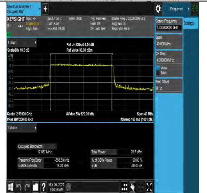
NTNV-N7-PC3-15-20-M-DFT-256QAM-Outter_Full-Ant0-PASS
