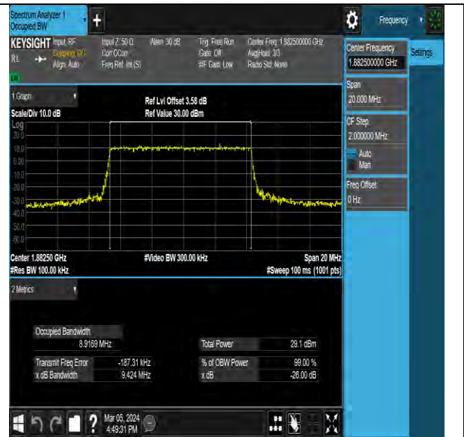
NTNV-N25-PC3-15-10-M-DFT-256QAM-Outer_Full-Ant0-PA SS
