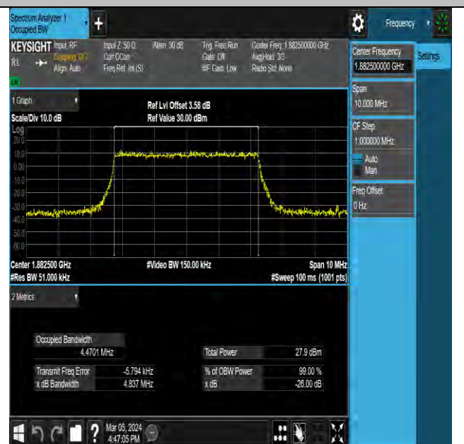
NTNV-N25-PC3-15-5-M-DFT-64QAM-Outet_Full-Ant0-PASS
