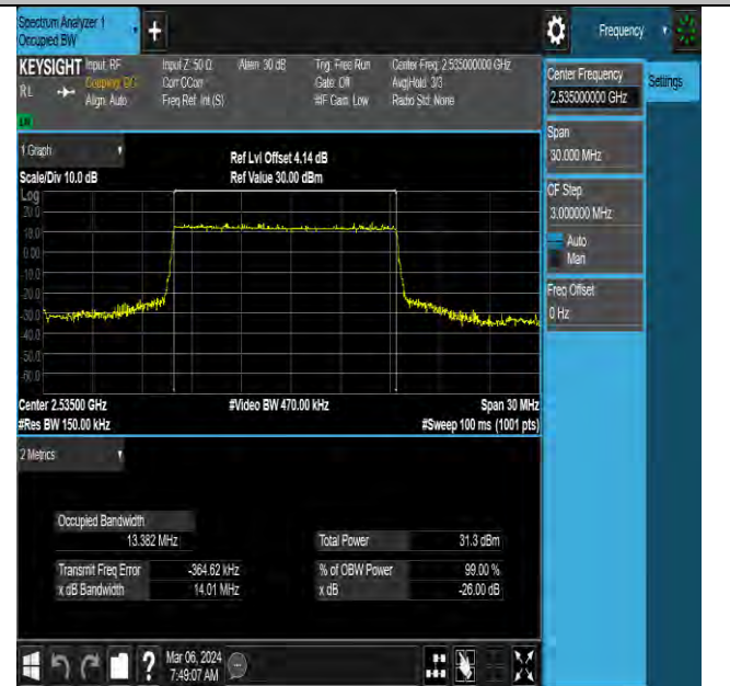
NTNV-N7-PC3-15-15-M-DFT-QPSK-Outer_Full-Ant0-PASS
