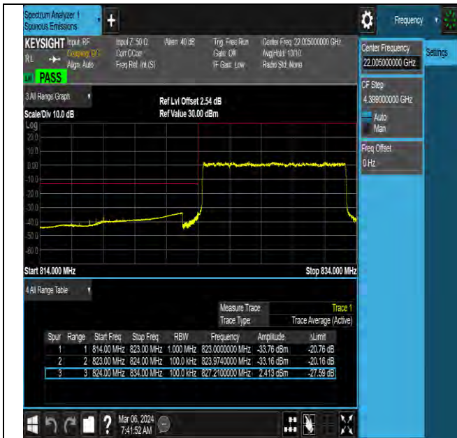
NTNV-N5-PC3-15-10-L-DFT-QPSK-Outer_Full-Ant0-PASS
