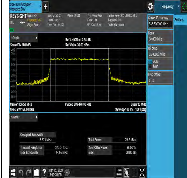
NTNV-N5-PC3-15-15-M-DFT-256QAM-Outer_Full-Ant0-PASS
