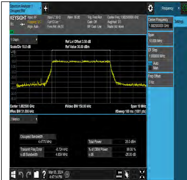
NTNV-N25-PC3-15-5-M-DFT-256QAM-Outet_Full-Ant0-PAS S
