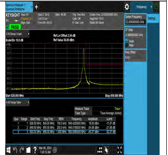
NTNV-N5-PC3-15-20-H-DFT-QPSK-Edge_1RB_Right-Ant0-PASS
