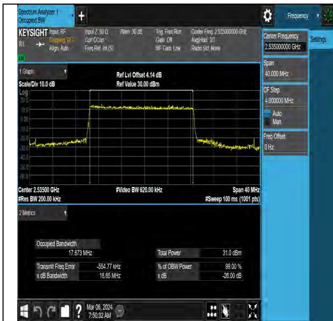
NTNV-N7-PC3-15-20-M-DFT-QPSK-Outter_Full-Ant0-PASS
