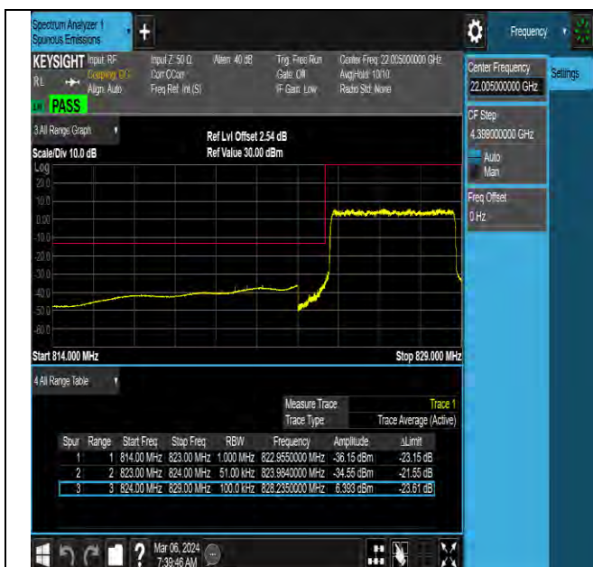
NTNV-N5-PC3-15-5-L-DFT-QPSK-Outer_Full-Ant0-PASS
