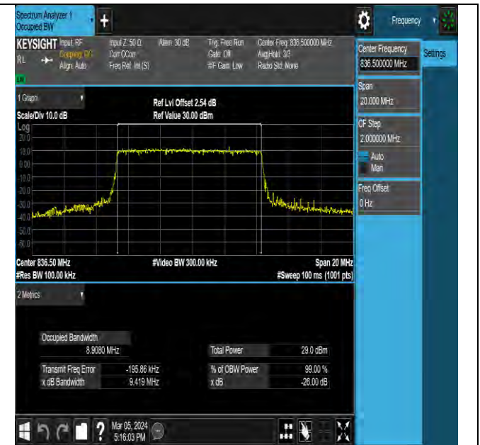
NTNV-N5-PC3-15-10-M-DFT-256QAM-Outer_Full-Ant0-PASS
