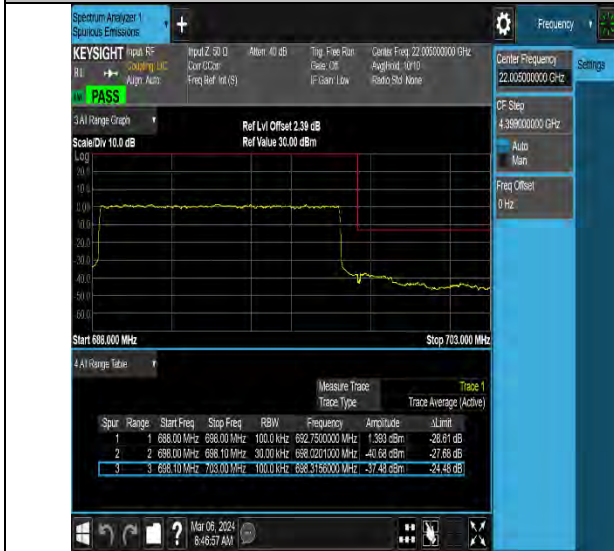
NTNV-N71-PC3-15-10-H-DFT-QPSK-Outer_Full-Ant0-PASS
