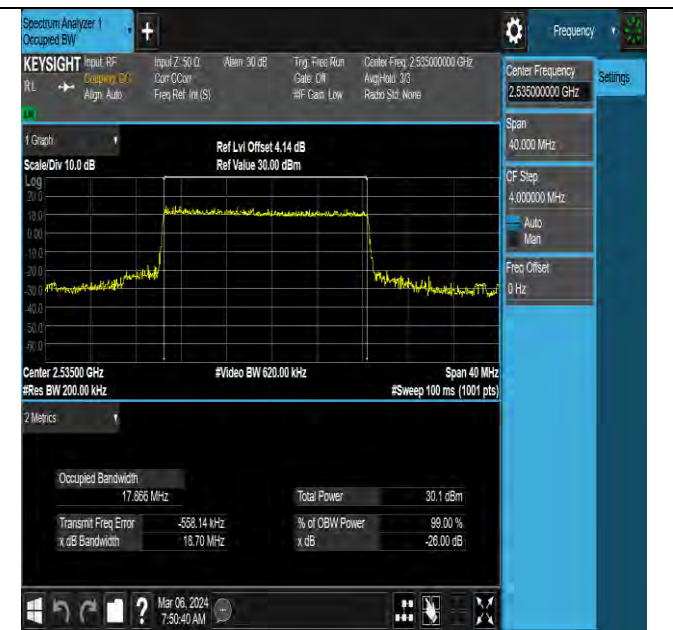
NTNV-N7-PC3-15-20-M-DFT-16QAM-Outter_Full-Ant0-PASS
