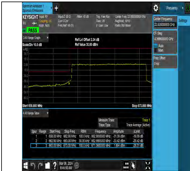
NTNV-N71-PC3-15-10-L-DFT-QPSK-Outer_Full-Ant0-PASS
