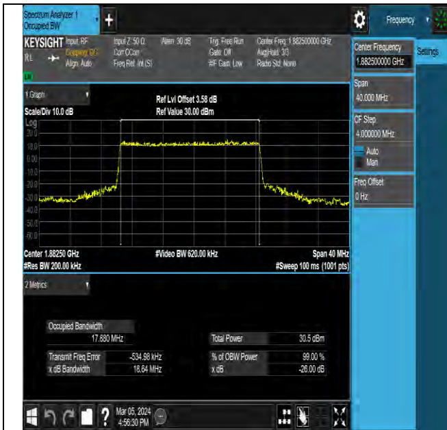
NTNV-N25-PC3-15-20-M-DFT-QPSK-Outer_Full-Ant0-PASS
