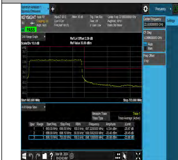
NTNV-N71-PC3-15-5-H-DFT-QPSK-Outer_Full-Ant0-PASS
