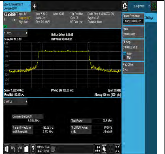
NTNV-N25-PC3-15-10-M-DFT-16QAM-Outet_Full-Ant0-PAS S
