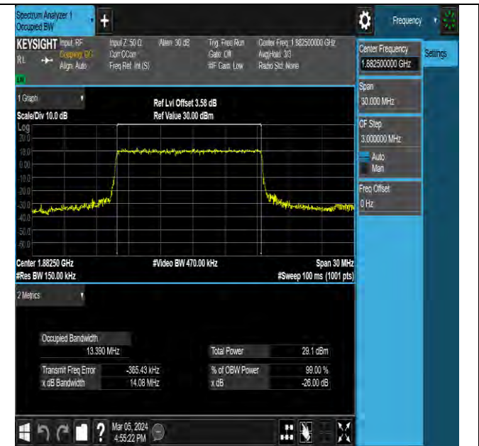
NTNV-N25-PC3-15-15-M-DFT-64QAM-Outer_Full-Ant0-PAS S
