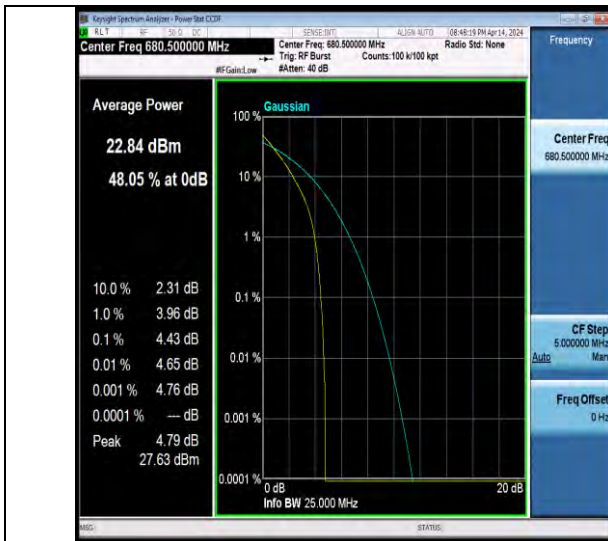
NTNV-N71-PC3-15-20-M-DFT-QPSK-Outer Full-PASS
