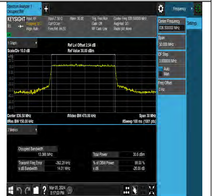
NTNV-N5-PC3-15-15-M-DFT-QPSK-Outer_Full-Ant0-PASS
