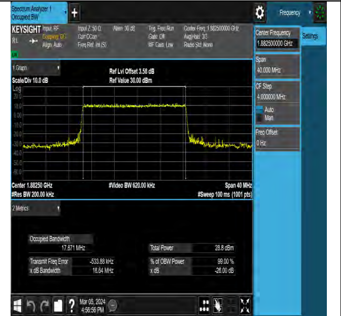
NTNV-N25-PC3-15-20-M-DFT-256QAM-Outer_Full-Ant0-PA SS
