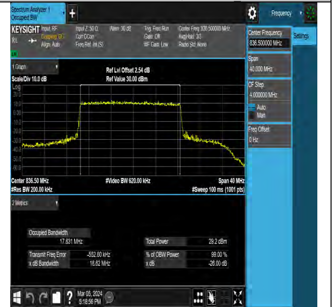
NTNV-N5-PC3-15-20-M-DFT-256QAM-Outter_Full-Ant0-PASS
