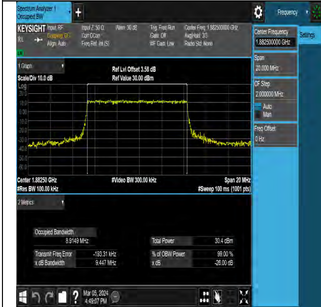
NTNV-N25-PC3-15-10-M-DFT-QPSK-Outet_Full-Ant0-PASS
