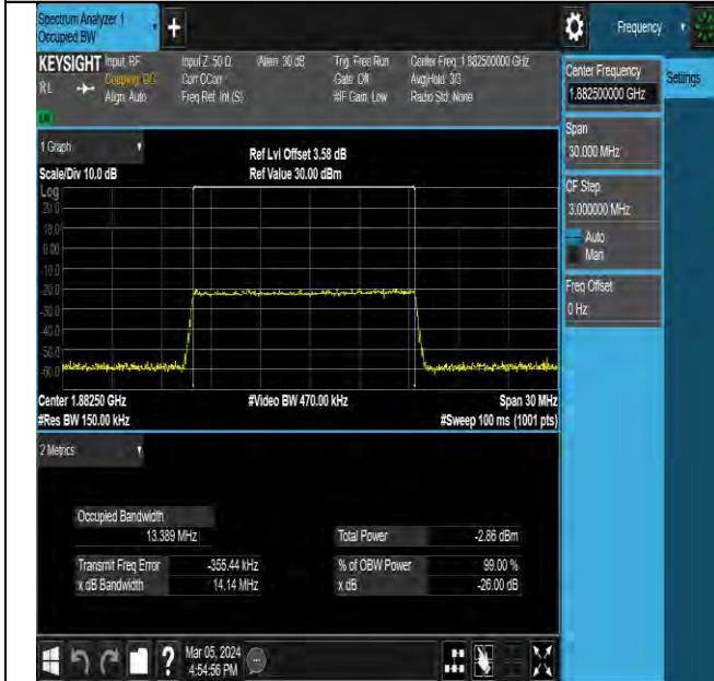
NTNV-N25-PC3-15-15-M-DFT-PI2BPSK-Outer_Full-Ant0-PA SS
