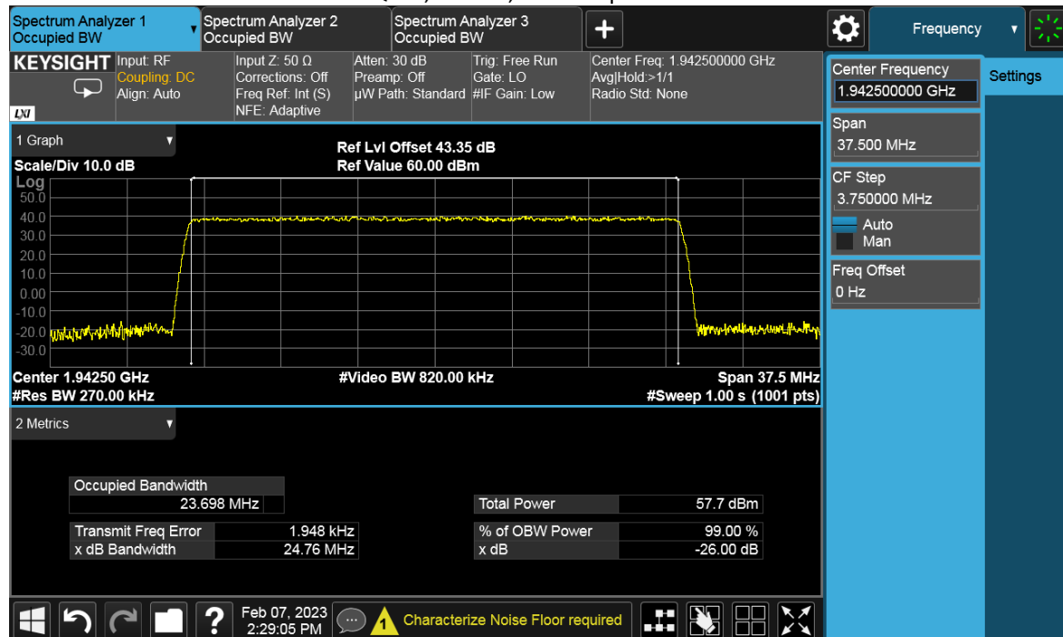
QPSK, 25MHz, Channel position B
