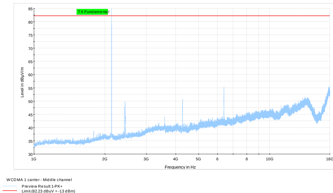
Figure 7.1-10: Radiated emissions spectral plot (1 to 18 GHz) – FCC §27.53 and RSS-139
