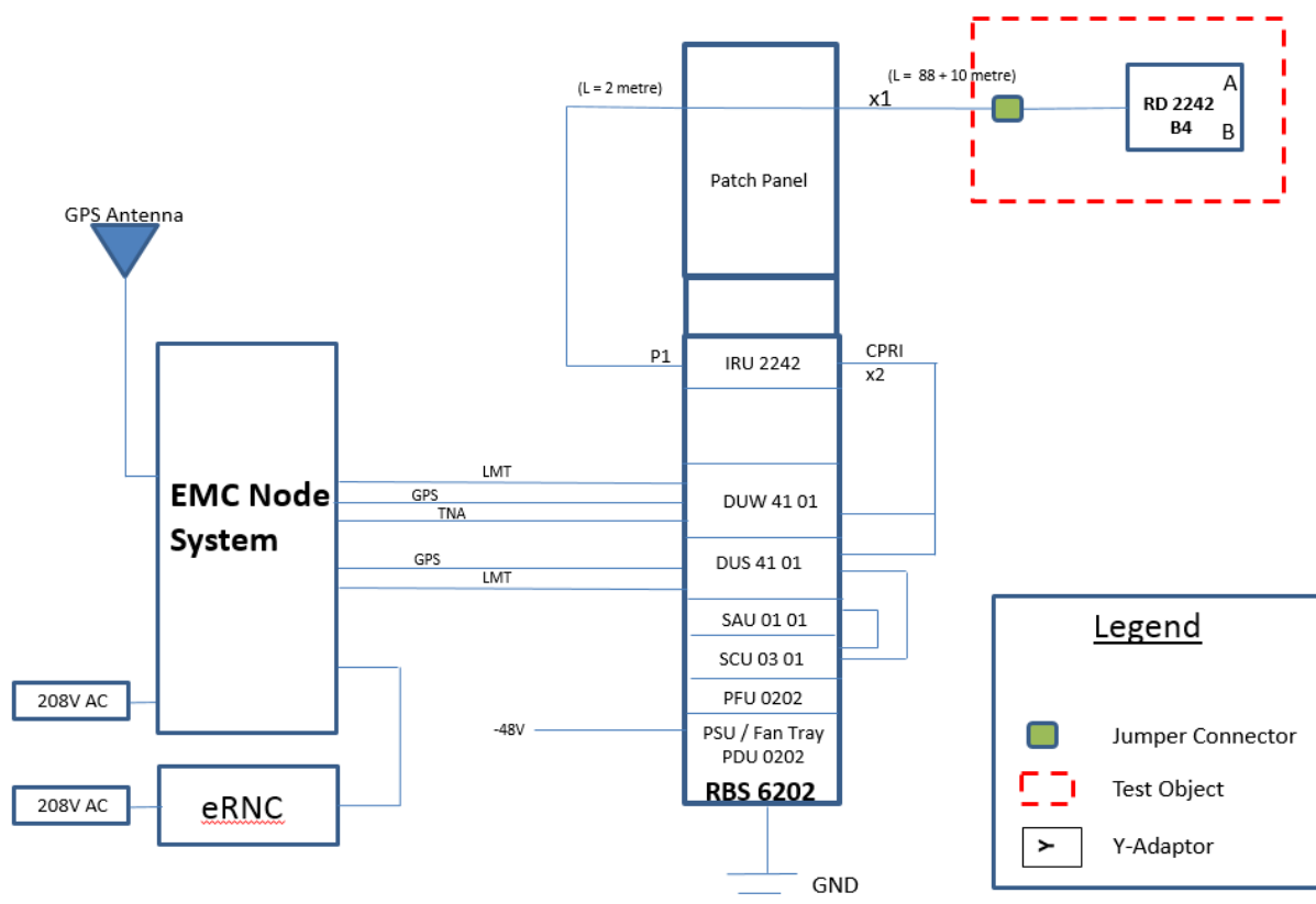
Figure 3.6-1: Setup diagram
