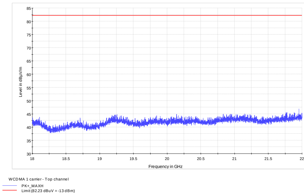
Figure 7.1-17: Radiated emissions spectral plot (18 to 22 GHz) – FCC §27.53 and RSS-139
