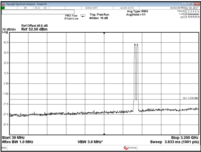
Figure 8.2-63: Conducted spurious emissions within 30–3200 MHz, Port A, 2 carriers: 20 MHz each at the top of the band, QPSK
