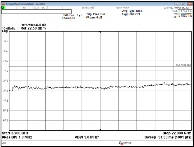
Figure 8.2-64: Conducted spurious emissions within 3200–22000 MHz, Port A, 2 carriers: 20 MHz each at the top of the band, QPSK
