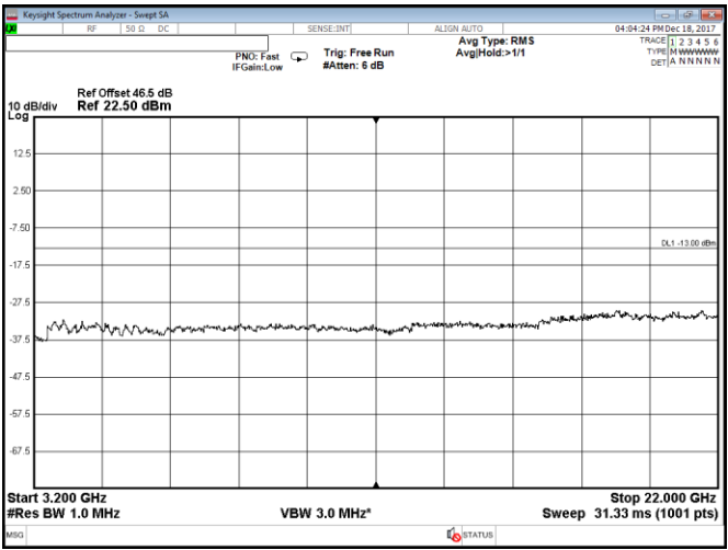
Figure 8.2-66: Conducted spurious emissions within 3200–22000 MHz, Port B, 2 carriers: 5 MHz each at the bottom of the band, QPSK
