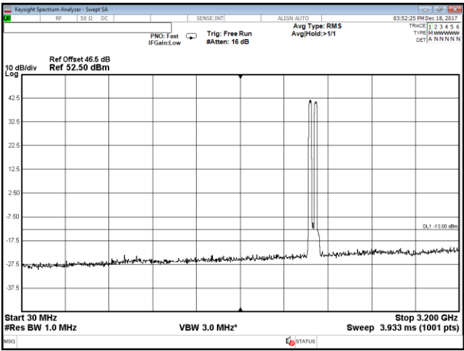
Figure 8.2-71: Conducted spurious emissions within 30–3200 MHz, Port B, 2 carriers: 20 MHz each at the bottom of the band, QPSK
