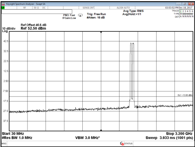
Figure 8.2-79: Conducted spurious emissions within 30–3200 MHz, Port B, 2 carriers: 20 MHz each at the top of the band, QPSK
