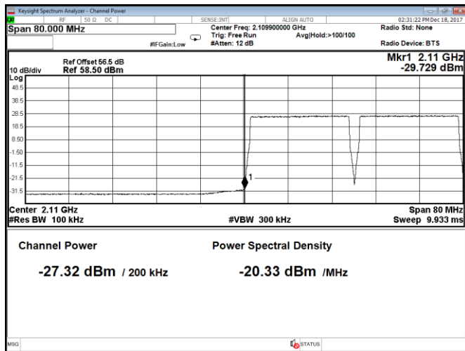
Figure 8.2-111: Conducted band edge emission at 2110 MHz, Port B, 20 MHz channel, QPSK (RBW = 1% of EBW)
