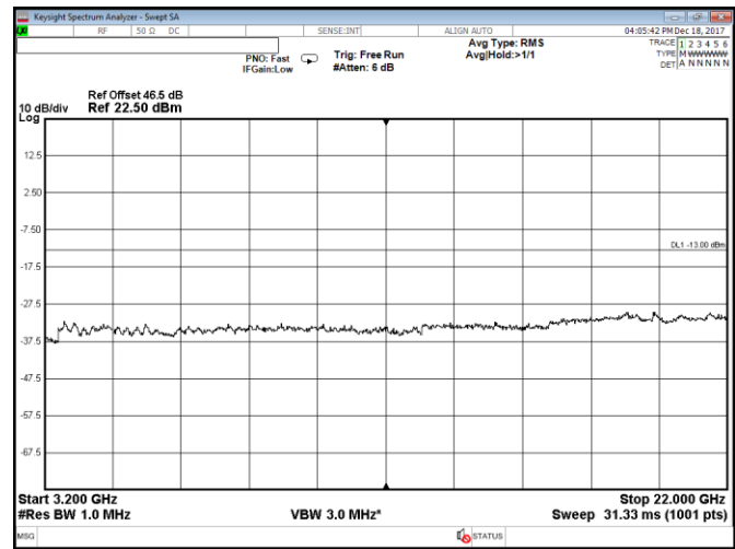
Figure 8.2-58: Conducted spurious emissions within 3200–22000 MHz, Port A, 2 carriers: 5 MHz each at the top of the band, QPSK
