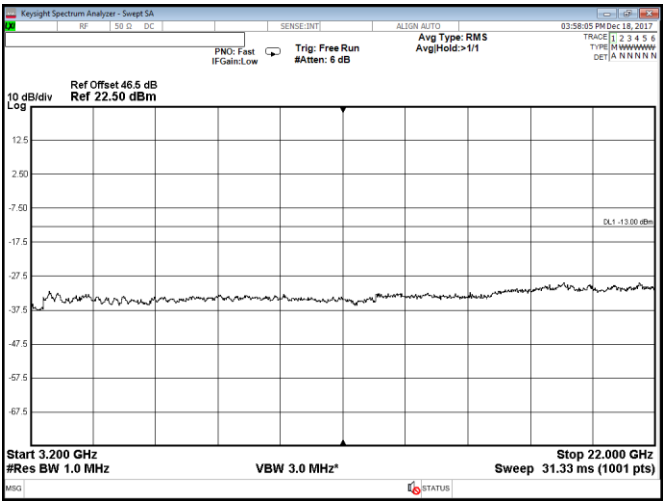
Figure 8.2-56: Conducted spurious emissions within 3200–22000 MHz, Port A, 2 carriers: 20 MHz each at the bottom of the band, QPSK
