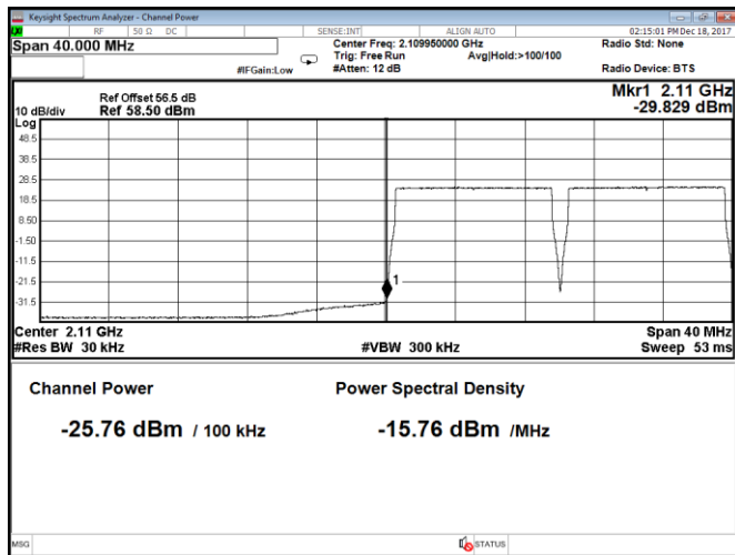
Figure 8.2-99: Conducted band edge emission at 2110 MHz, Port A, 10 MHz channel, 2 carriers, QPSK (RBW = 1% of EBW)
