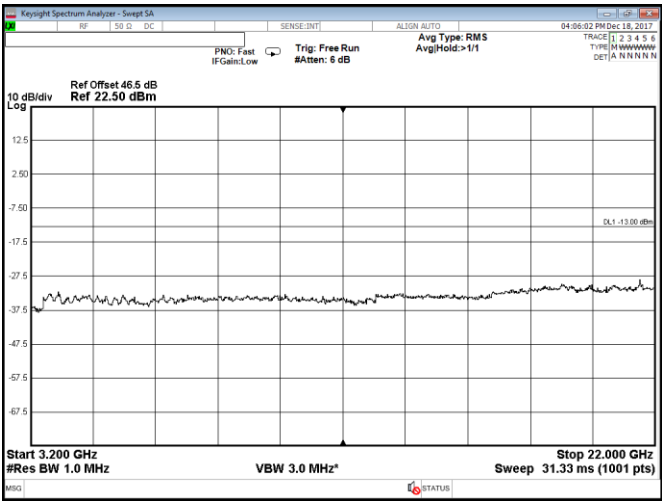
Figure 8.2-74: Conducted spurious emissions within 3200–22000 MHz, Port B, 2 carriers: 5 MHz each at the top of the band, QPSK
