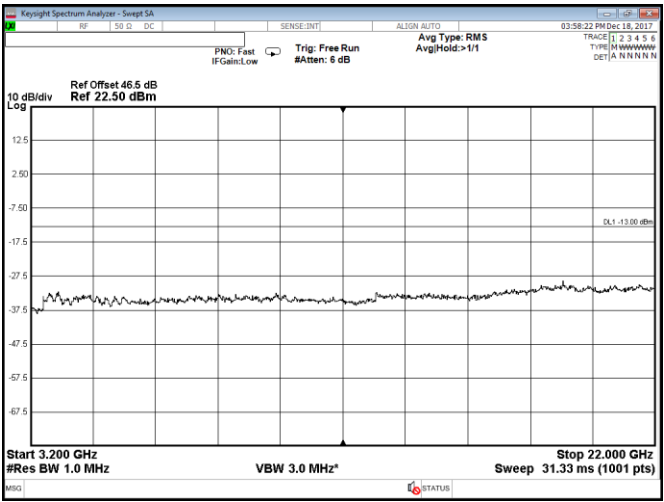
Figure 8.2-72: Conducted spurious emissions within 3200–22000 MHz, Port B, 2 carriers: 20 MHz each at the bottom of the band, QPSK
