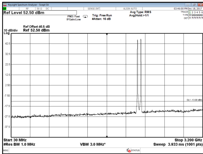
Figure 8.2-57: Conducted spurious emissions within 30–3200 MHz, Port A, 2 carriers: 5 MHz each at the top of the band, QPSK
