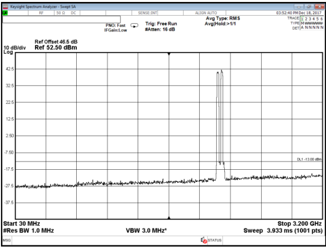
Figure 8.2-55: Conducted spurious emissions within 30–3200 MHz, Port A, 2 carriers: 20 MHz each at the bottom of the band, QPSK
