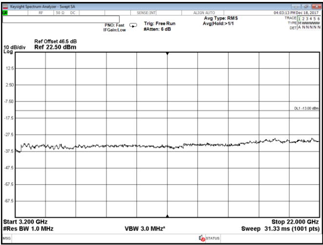
Figure 8.2-52: Conducted spurious emissions within 3200–22000 MHz, Port A, 2 carriers: 10 MHz each at the bottom of the band, QPSK
