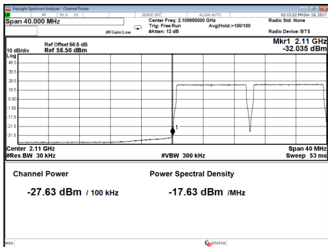
Figure 8.2-107: Conducted band edge emission at 2110 MHz, Port B, 10 MHz channel, QPSK (RBW = 1% of EBW)
