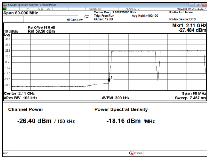
Figure 8.2-101: Conducted band edge emission at 2110 MHz, Port A, 15 MHz channel, 2 carriers, QPSK (RBW = 1% of EBW)
