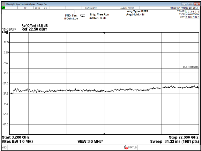
Figure 8.2-78: Conducted spurious emissions within 3200–22000 MHz, Port B, 2 carriers: 15 MHz each at the top of the band, QPSK
