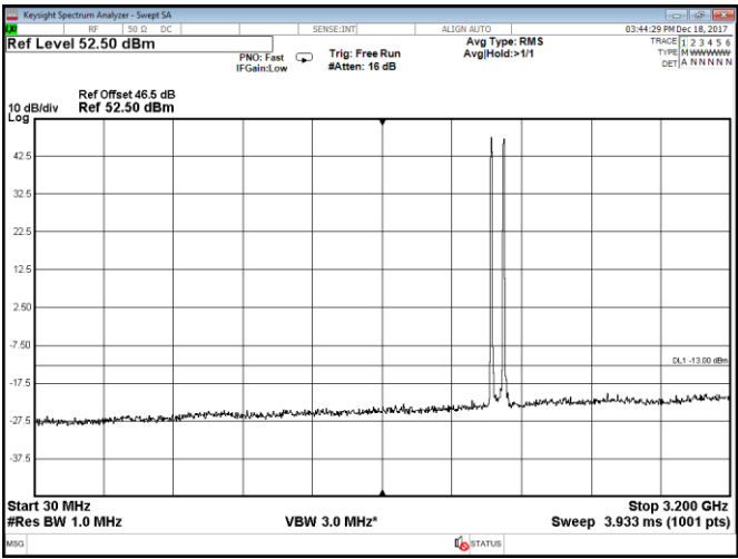
Figure 8.2-65: Conducted spurious emissions within 30–3200 MHz, Port B, 2 carriers: 5 MHz each at the bottom of the band, QPSK
