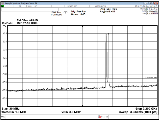
Figure 8.2-69: Conducted spurious emissions within 30–3200 MHz, Port B, 2 carriers: 15 MHz each at the bottom of the band, QPSK
