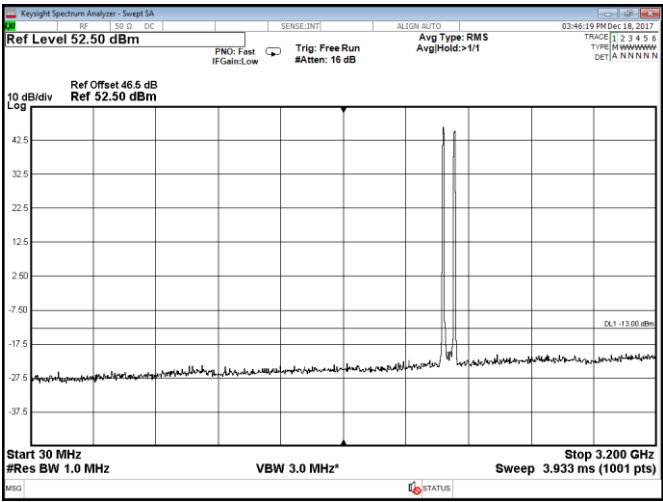
Figure 8.2-73: Conducted spurious emissions within 30–3200 MHz, Port B, 2 carriers: 5 MHz each at the top of the band, QPSK
