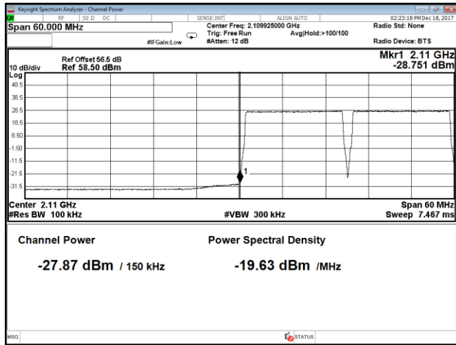
Figure 8.2-109: Conducted band edge emission at 2110 MHz, Port B, 15 MHz channel, QPSK (RBW = 1% of EBW)
