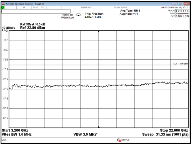
Figure 8.2-62: Conducted spurious emissions within 3200–22000 MHz, Port A, 2 carriers: 15 MHz each at the top of the band, QPSK
