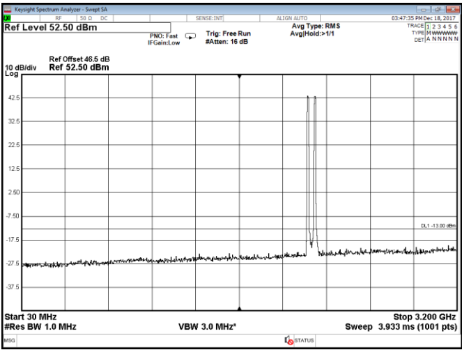
Figure 8.2-51: Conducted spurious emissions within 30–3200 MHz, Port A, 2 carriers: 10 MHz each at the bottom of the band, QPSK
