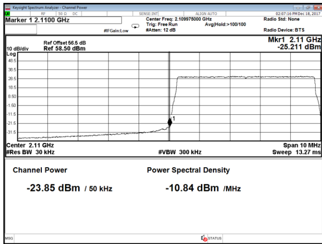
Figure 8.2-81: Conducted band edge emission at 2110 MHz, Port A, 5 MHz channel, QPSK (RBW = 1% of EBW)
