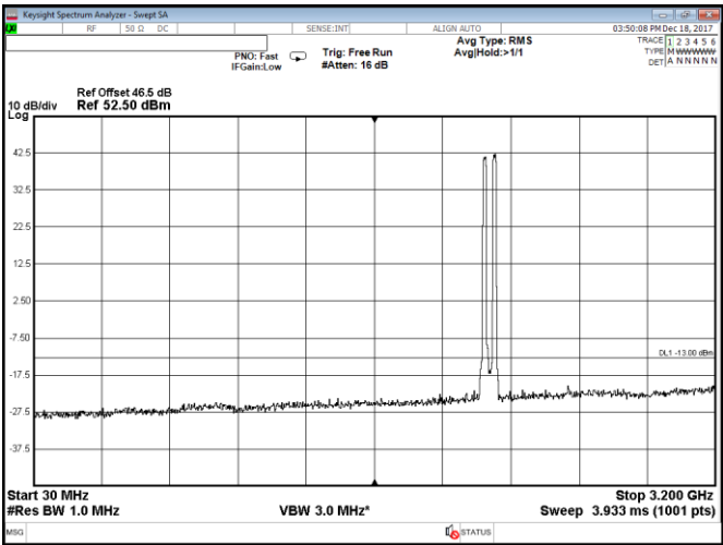
Figure 8.2-77: Conducted spurious emissions within 30–3200 MHz, Port B, 2 carriers: 15 MHz each at the top of the band, QPSK
