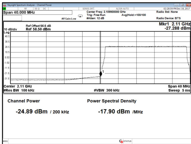
Figure 8.2-87: Conducted band edge emission at 2110 MHz, Port A, 20 MHz channel, QPSK (RBW = 1% of EBW)
