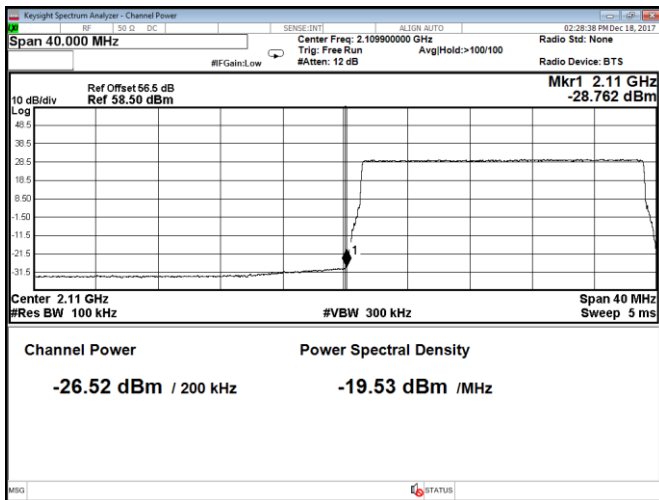
Figure 8.2-95: Conducted band edge emission at 2110 MHz, Port B, 20 MHz channel, QPSK (RBW = 1% of EBW)
