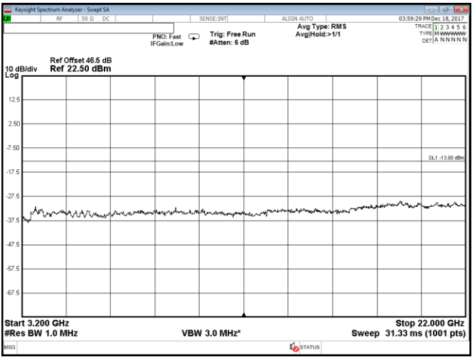
Figure 8.2-70: Conducted spurious emissions within 3200–22000 MHz, Port B, 2 carriers: 15 MHz each at the bottom of the band, QPSK
