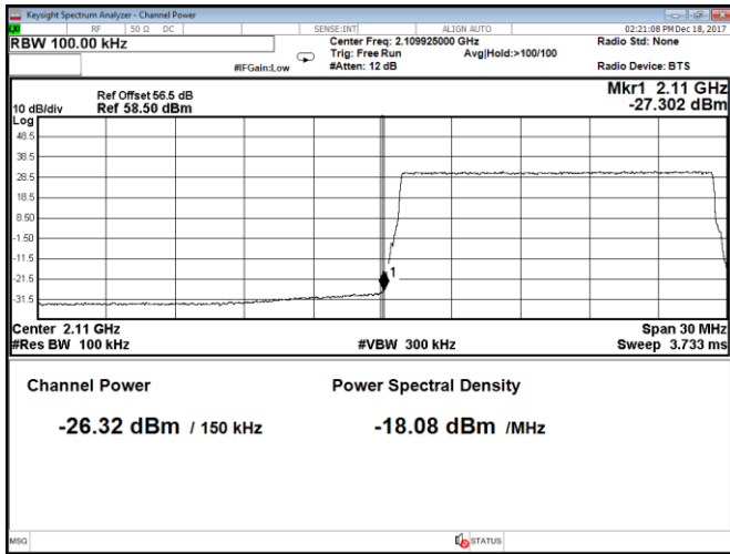
Figure 8.2-93: Conducted band edge emission at 2110 MHz, Port B, 15 MHz channel, QPSK (RBW = 1% of EBW)
