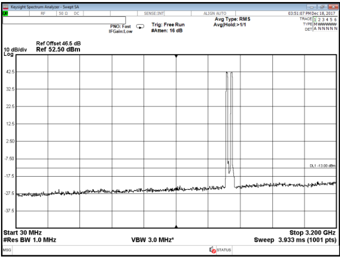
Figure 8.2-53: Conducted spurious emissions within 30–3200 MHz, Port A, 2 carriers: 15 MHz each at the bottom of the band, QPSK
