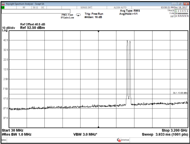
Figure 8.2-61: Conducted spurious emissions within 30–3200 MHz, Port A, 2 carriers: 15 MHz each at the top of the band, QPSK
