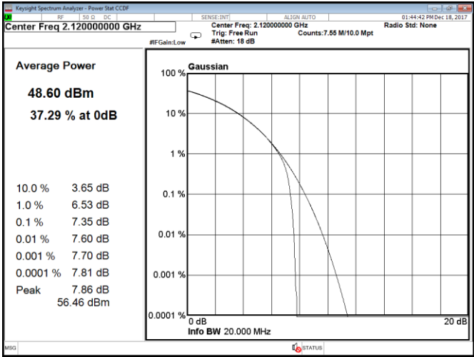
Figure 8.1-102: CCDF, QPSK, 20 MHz, Port B, Low channel
