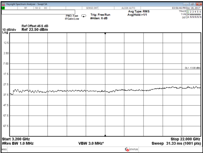
Figure 8.2-80: Conducted spurious emissions within 3200–22000 MHz, Port B, 2 carriers: 20 MHz each at the top of the band, QPSK
