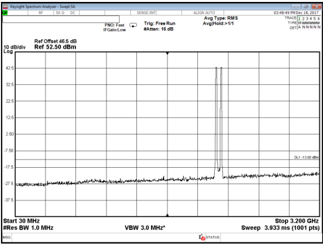
Figure 8.2-75: Conducted spurious emissions within 30–3200 MHz, Port B, 2 carriers: 10 MHz each at the top of the band, QPSK
