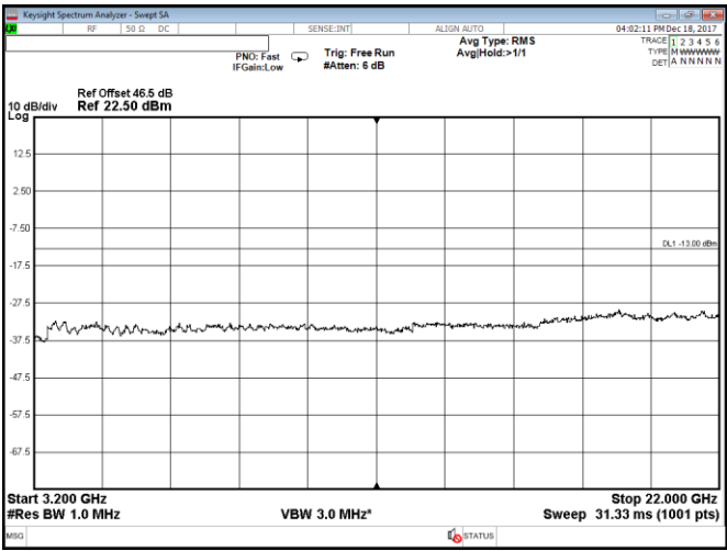
Figure 8.2-76: Conducted spurious emissions within 3200–22000 MHz, Port B, 2 carriers: 10 MHz each at the top of the band, QPSK
