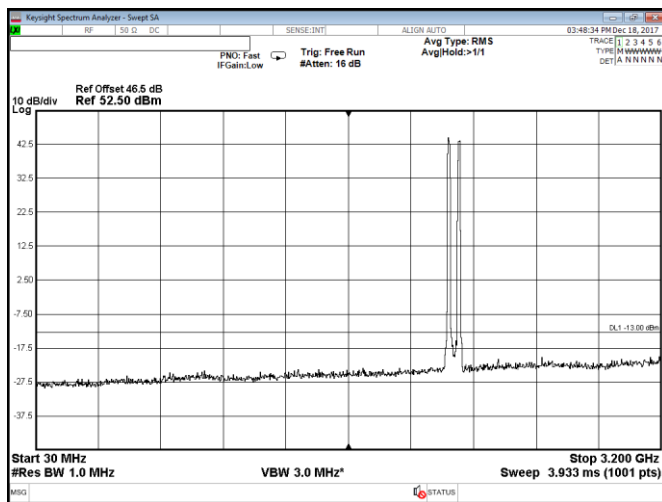
Figure 8.2-59: Conducted spurious emissions within 30–3200 MHz, Port A, 2 carriers: 10 MHz each at the top of the band, QPSK
