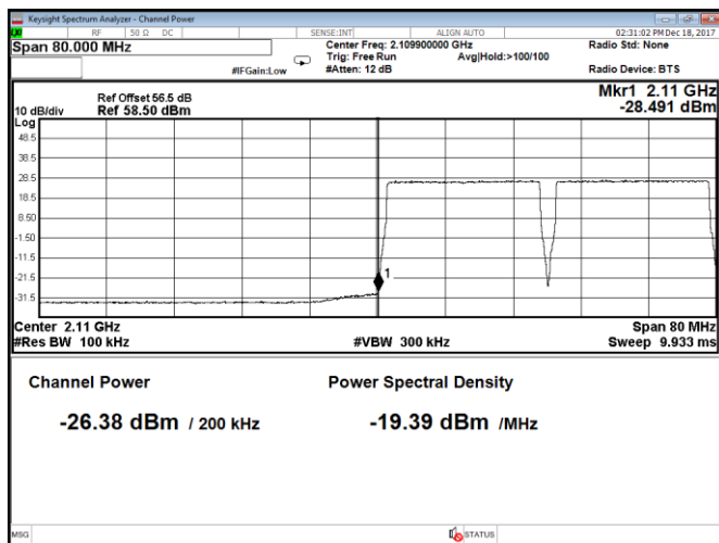
Figure 8.2-103: Conducted band edge emission at 2110 MHz, Port A, 20 MHz channel, 2 carriers, QPSK (RBW = 1% of EBW)
