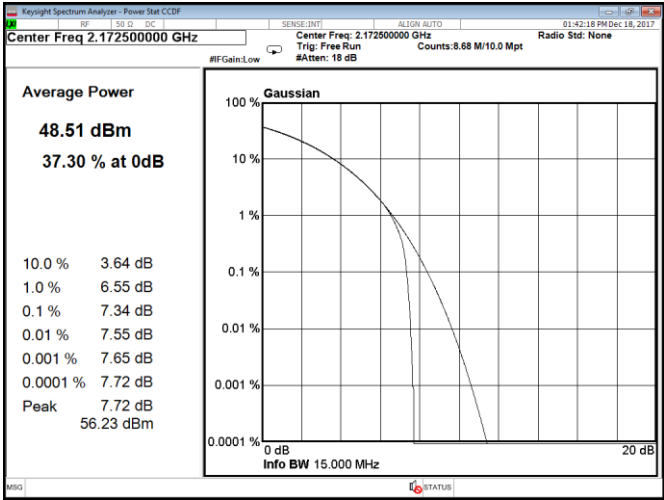
Figure 8.1-98: CCDF, QPSK, 15 MHz, Port B, High channel
