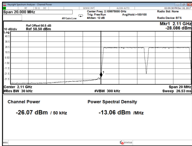
Figure 8.2-105: Conducted band edge emission at 2110 MHz, Port B, 5 MHz channel, QPSK (RBW = 1% of EBW)
