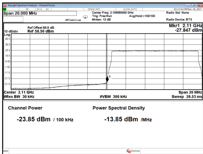
Figure 8.2-83: Conducted band edge emission at 2110 MHz, Port A, 10 MHz channel, QPSK (RBW = 1% of EBW)
