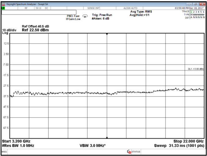
Figure 8.2-54: Conducted spurious emissions within 3200–22000 MHz, Port A, 2 carriers: 15 MHz each at the bottom of the band, QPSK
