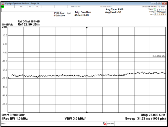
Figure 8.2-68: Conducted spurious emissions within 3200–22000 MHz, Port B, 2 carriers: 10 MHz each at the bottom of the band, QPSK
