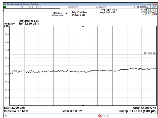
Figure 8.2-60: Conducted spurious emissions within 3200–22000 MHz, Port A, 2 carriers: 10 MHz each at the top of the band, QPSK
