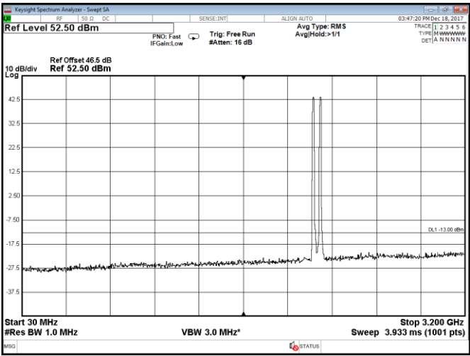
Figure 8.2-67: Conducted spurious emissions within 30–3200 MHz, Port B, 2 carriers: 10 MHz each at the bottom of the band, QPSK
