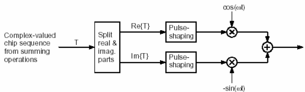
Figure 11: Downlink modulation
