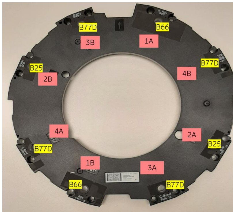
Figure C.2 Top view of the EUT without the radome with the active antenna elements labeled where '1A','1B','2A','2B','3A','3B','4A','4B' correspond to 'A','B','C','D','E','F','G','H' listed in the document.
