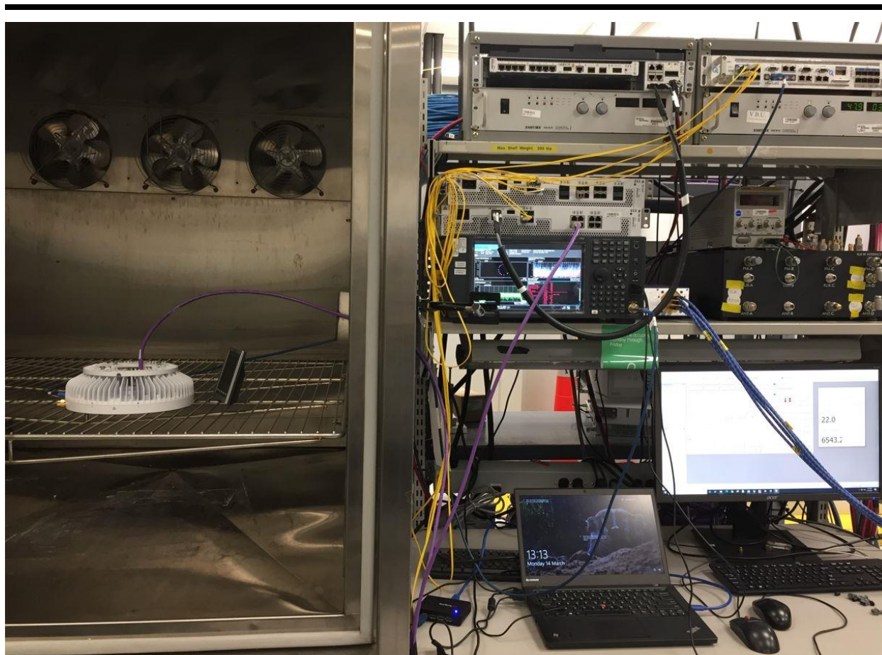
Figure 3: Frequency stability test setup
