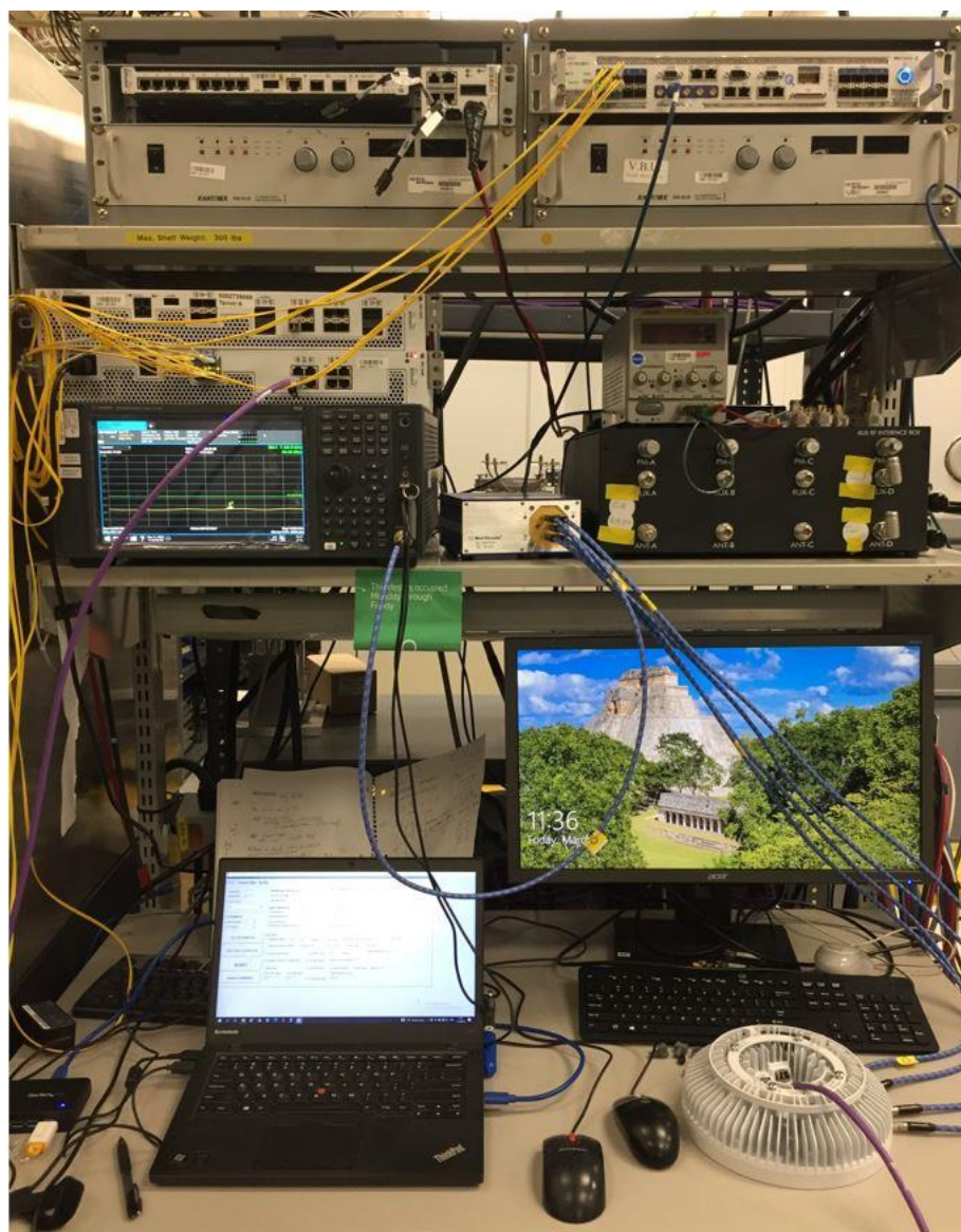
Figure 2: Conducted test setup
