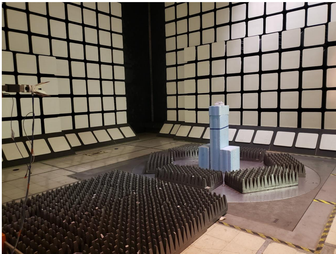
Figure 4: Radiated PSD test setup
