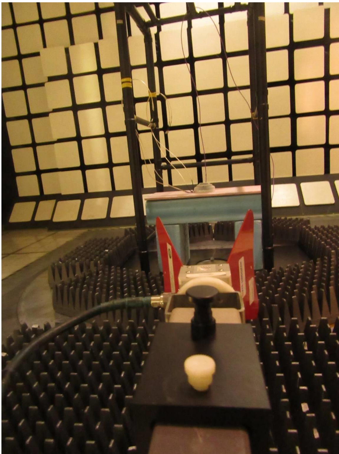
Figure 1: Radiated Test setup
