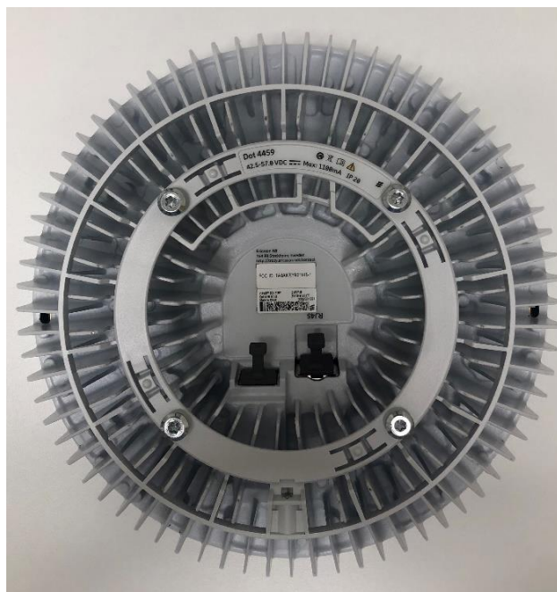
Figure 2: Dot 4459 B77D Bottom View
