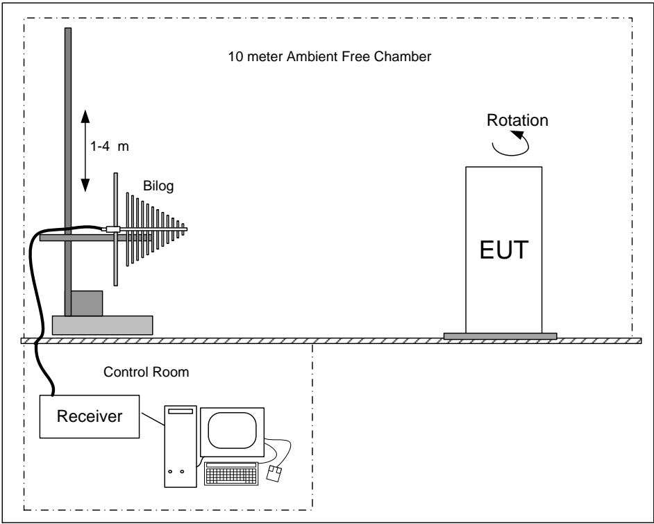
Figure 3: Setup of Radiated Emissions
