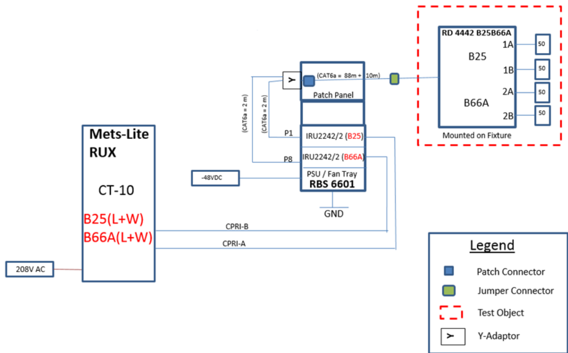
Figure 3.6-1: Setup diagram
