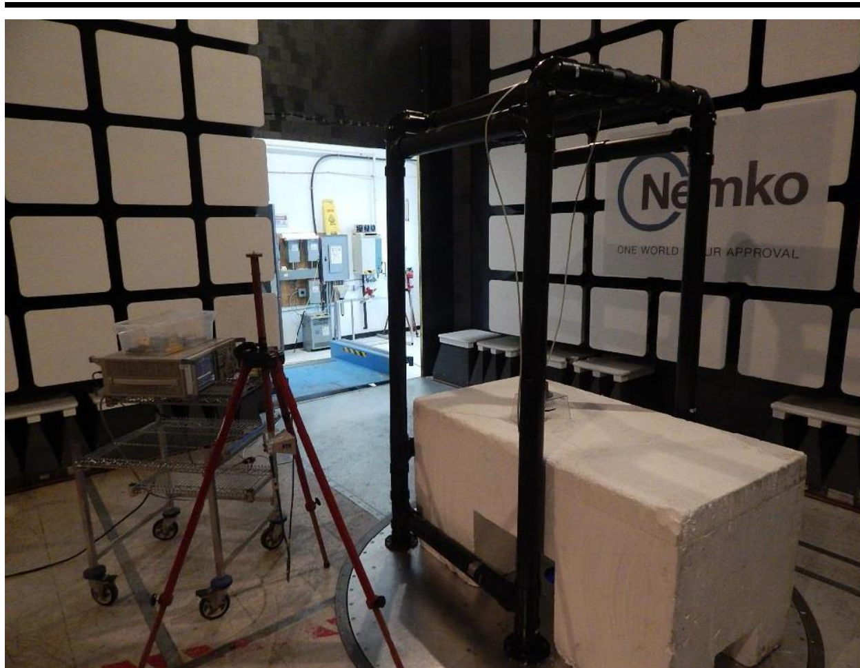
Figure 3: Radiated Test setup (frequency 18 – 37 GHz)
