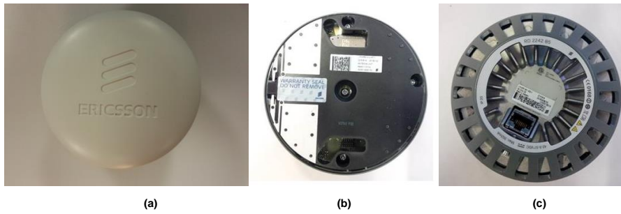
Figure C.1 The EUT. (a) Front view with radome. (b) Front view without radome. (c) Back view.
