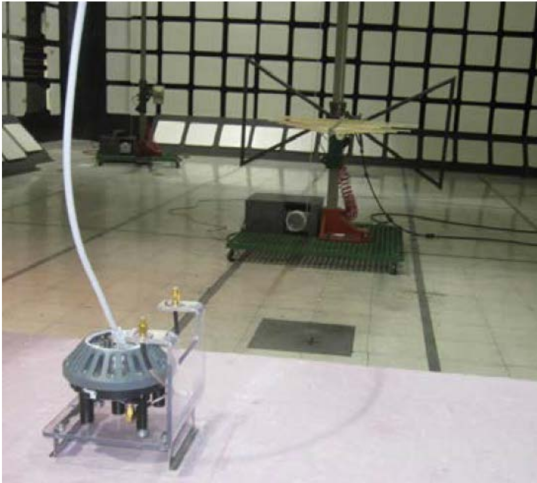
Figure 4 Test Antenna (30 MHz to 1 GHz)
