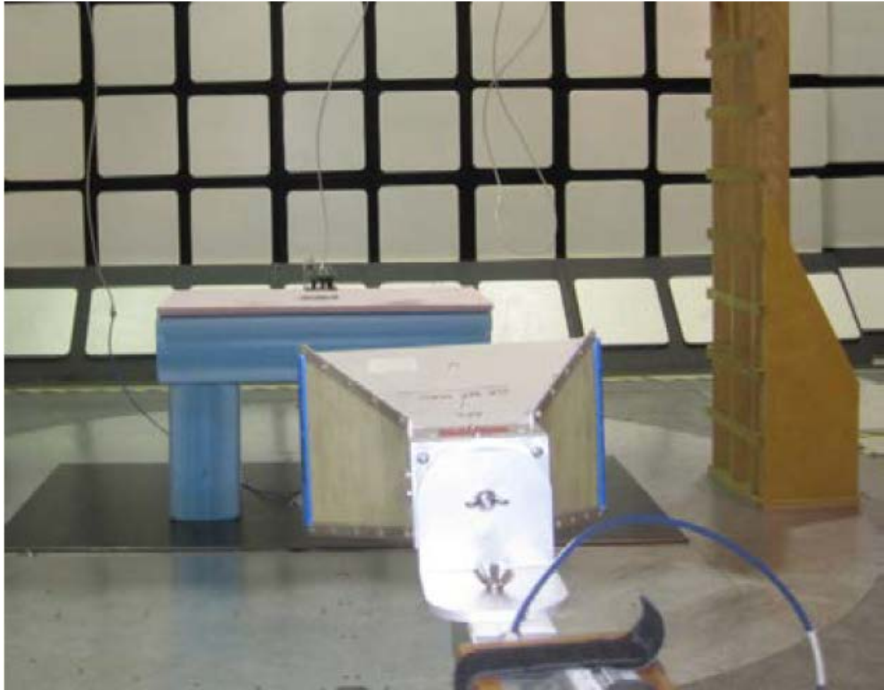
Figure 3 Test Antenna (1 to 10 GHz)
