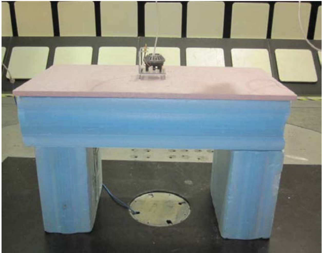
Figure 1 Radiated Emissions Test Setup
