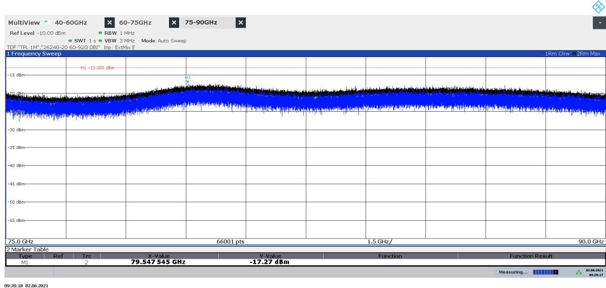
Diagram 2.36a: 75 – 90 GHz, QPSK, BMT8 50 , EIRP Horizontal polarization
