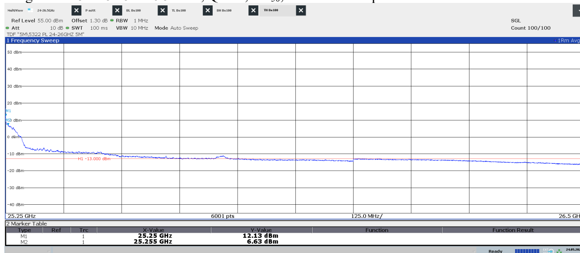
Diagram 2.18d: 25.25 – 26.5 GHz, QPSK, TH 50 , EIRP Vertical polarization
