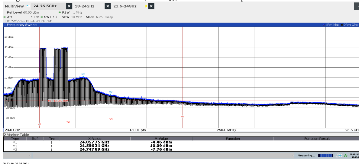
Diagram 2.15a: Pre scan 24 – 26.5 GHz, TimL 50 , EIRP Horizontal polarization
