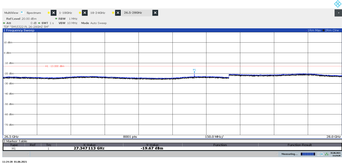
Diagram 2.22a: 26.5 – 28 GHz, QPSK, BL 50 , EIRP Horizontal polarization
