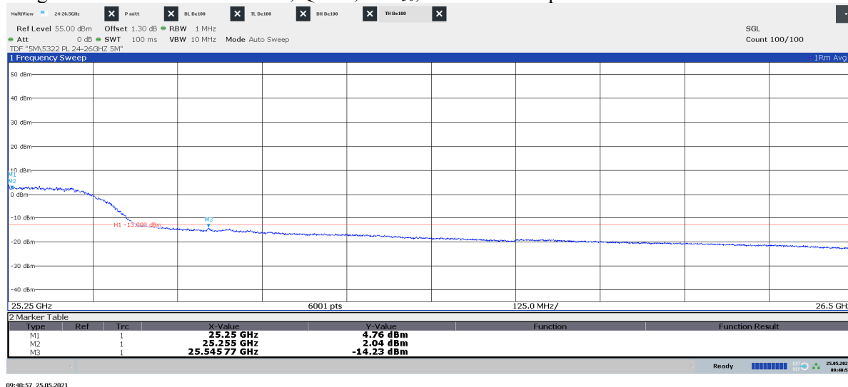
Diagram 2.20f: 25.25 – 26.5 GHz, QPSK, BT8 50 , EIRP Vertical polarization
