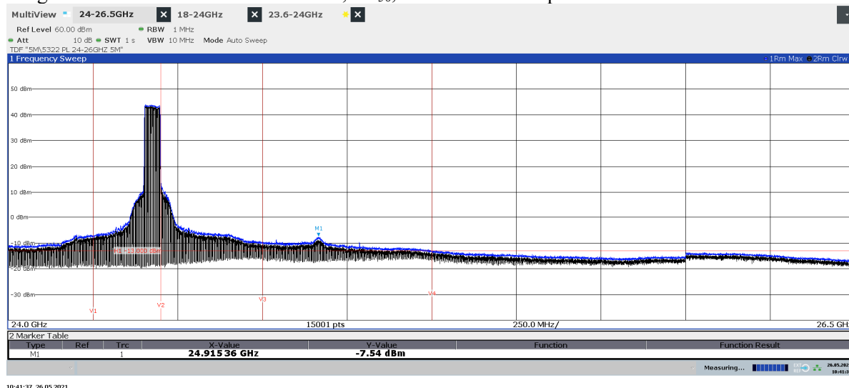
Diagram 2.14a: Pre scan 24 – 26.5 GHz, TL 50 , EIRP Horizontal polarization
