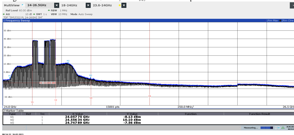
Diagram 2.15b: Pre scan 24 – 26.5 GHz, TimL 50 , EIRP Vertical polarization
