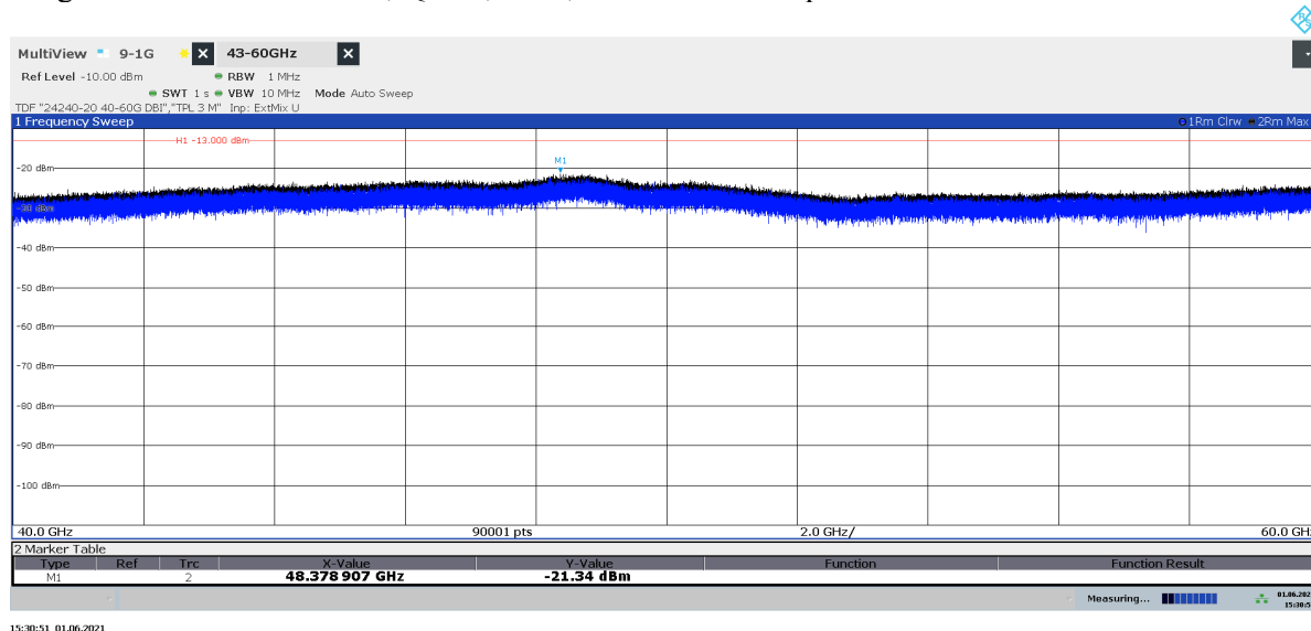
Diagram 2.28a: 40 – 60 GHz, QPSK, BH 50 , EIRP Horizontal polarization
