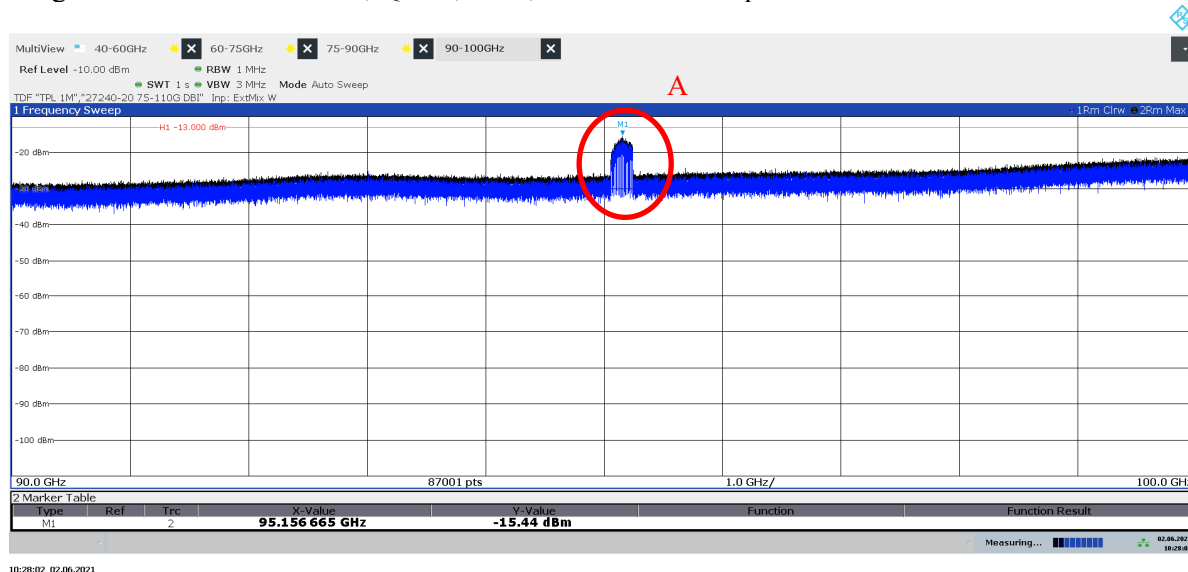
Diagram 2.37a: 90 – 100 GHz, QPSK, BH 50 , EIRP Horizontal polarization
