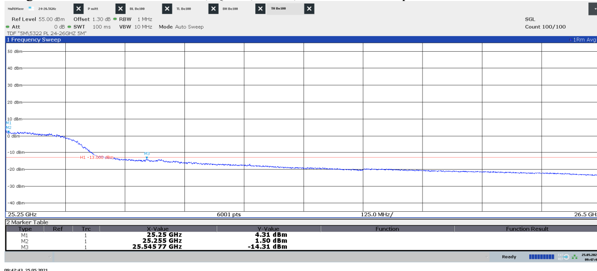
Diagram 2.20e: 25.25 – 26.5 GHz, QPSK, BT8 50 , EIRP Horizontal polarization
