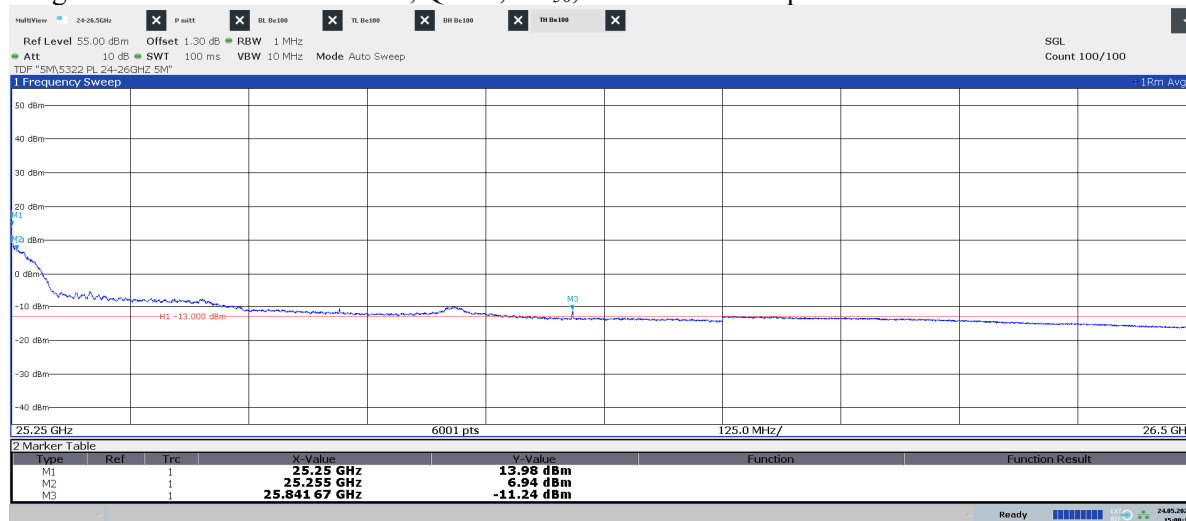
Diagram 2.18c: 25.25 – 26.5 GHz, QPSK, TH 50 , EIRP Horizontal polarization
