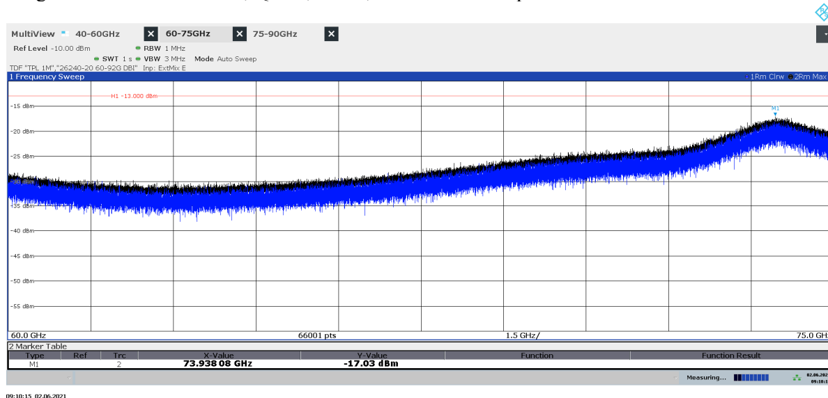
Diagram 2.32a: 60 – 75 GHz, QPSK, BT8 50 , EIRP Horizontal polarization
