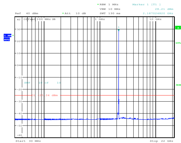
Figure 8.3-1: Conducted spurious emissions of 3× 5 MHz bottom channels
