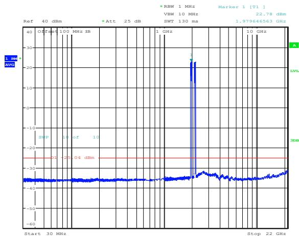
Figure 8.4-9: Conducted spurious emissions of 3x 5 MHz top B66 channels and 3x 15 MHz top B2/25 channels
