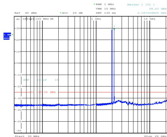
Figure 8.4-1: Conducted spurious emissions of 3x5 MHz bottom B66 channels and 3x5 MHz bottom B2/25 channels
