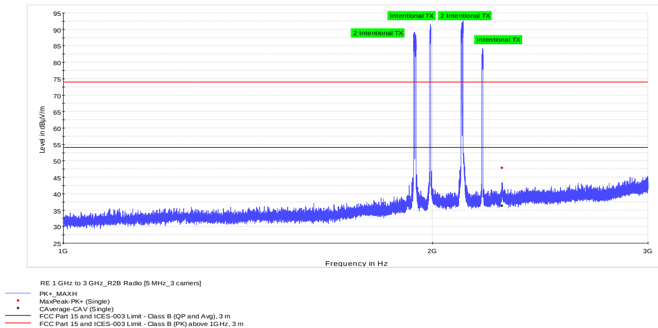
Figure 8.4-2: Radiated spurious emissions spectral plot (1 to 3 GHz)
