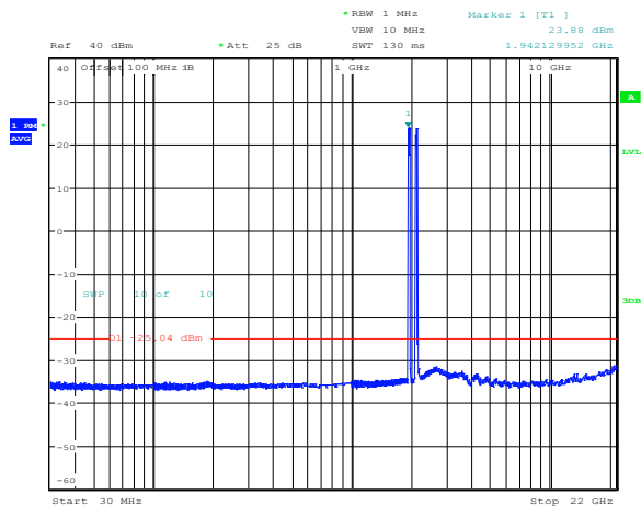
Figure 8.4-5: Conducted spurious emissions of 3x 10 MHz mid B66 channels and 3x 10 MHz mid B2/25 channels
