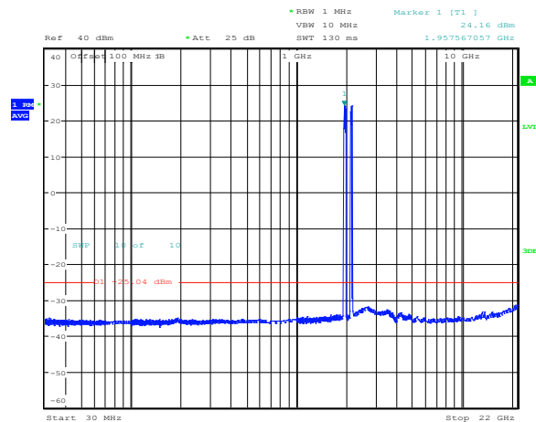
Figure 8.4-6: Conducted spurious emissions of 3x 10 MHz top B66 channels and 3x 10 MHz top B2/25 channels
