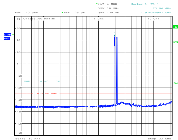
Figure 8.4-10: Conducted spurious emissions of 3x 10 MHz bottom B66 channels and 3x 20 MHz bottom B2/25 channels
