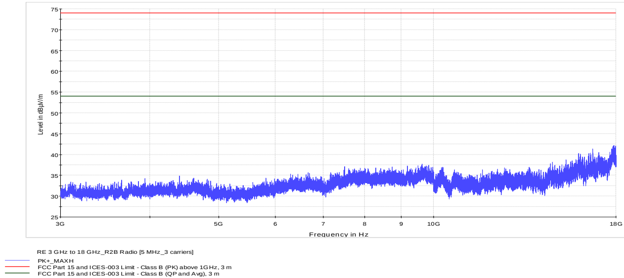
Figure 8.4-3: Radiated spurious emissions spectral plot (3 to 18 GHz)
