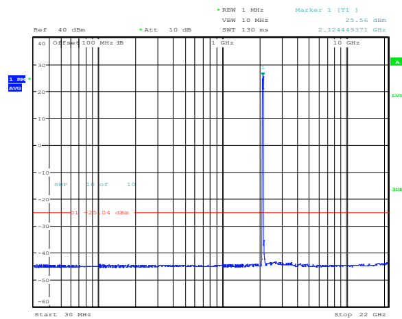
Figure 8.3-2: Conducted spurious emissions of 3× 5 MHz mid channels
