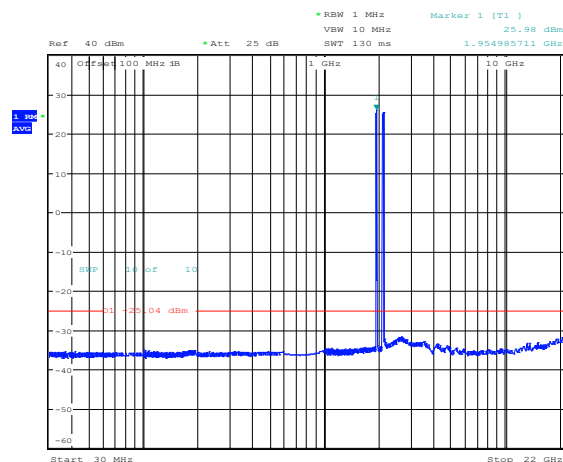
Figure 8.4-2: Conducted spurious emissions of 3x5 MHz mid B66 channels and 3x5 MHz mid B2/25 channels
