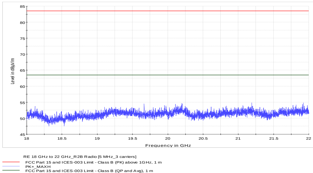
Figure 8.4-4: Radiated spurious emissions spectral plot (18 to 22 GHz)
