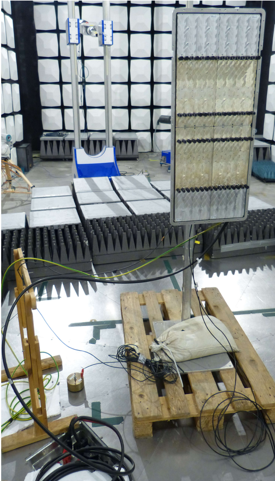
Photo of the test set-up for radiated emission above 18 – 26,5 GHz
