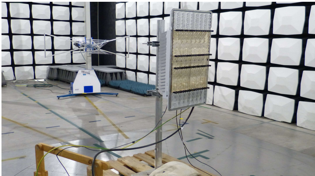
Photo of the test set-up for radiated emission 30 – 1000 MHz
