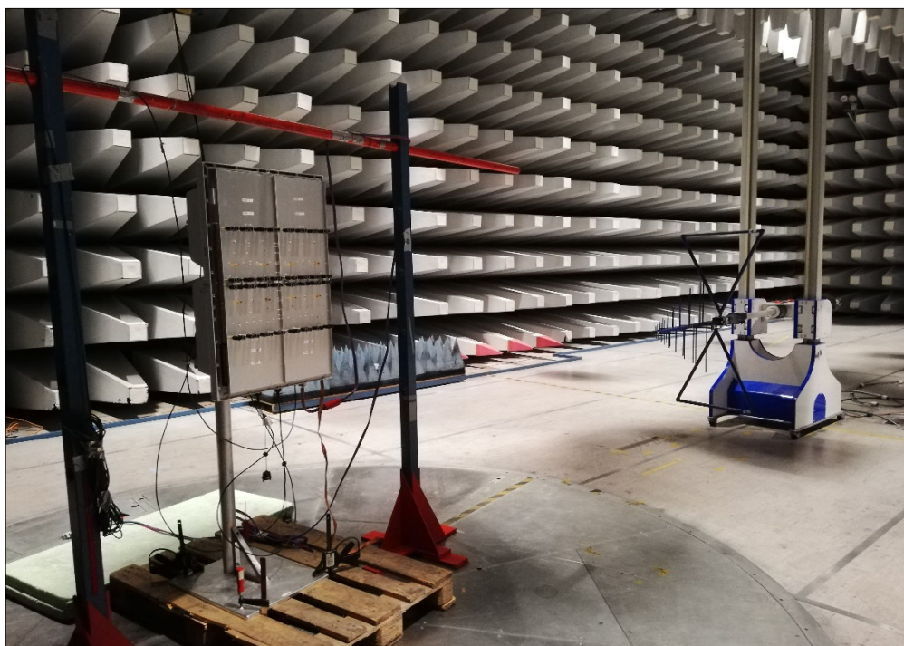
Figure 19 - Test Setup - 30 MHz to 1 GHz
