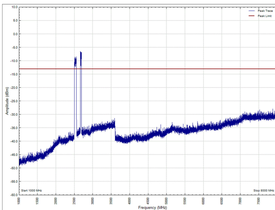
Figure 61 - 2526 MHz + 2665 MHz + 2675 MHz + 2685 MHz, 1 GHz to 8 GHz, Vertical
