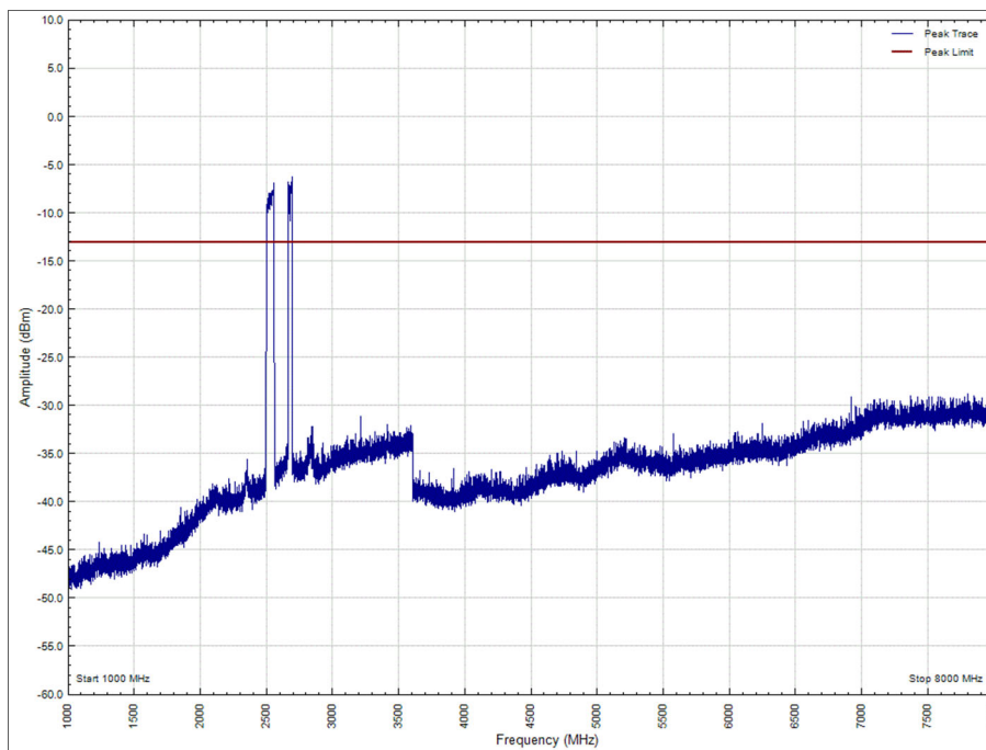
Figure 60 - 2526 MHz + 2665 MHz + 2675 MHz + 2685 MHz, 1 GHz to 8 GHz, Horizontal
