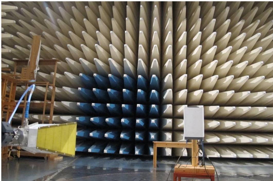
Radiated Emissions
