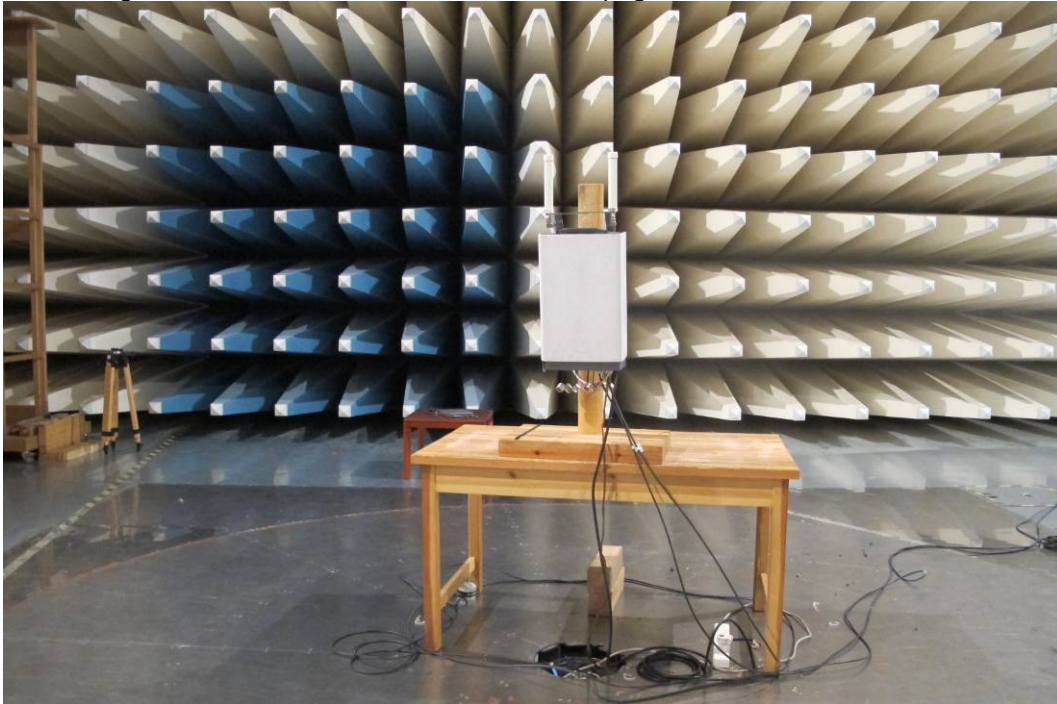
Semi-integrated Omni antenna KRE 101 2245/1, side mounted
