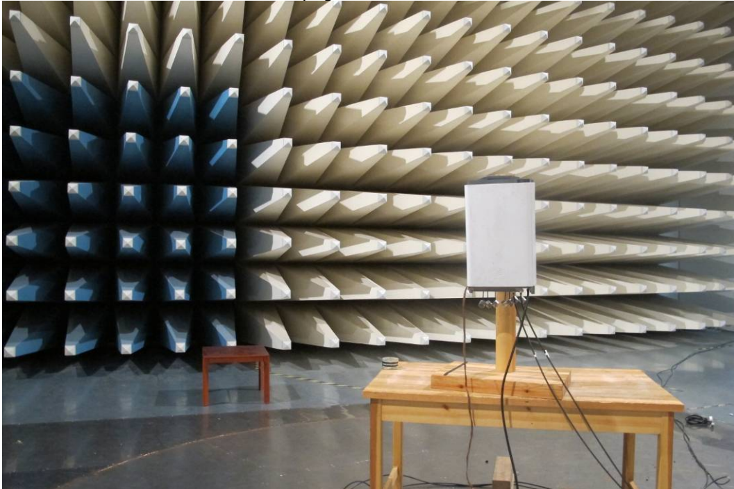
Internal antenna KRE 101 2135/1, side mounted
