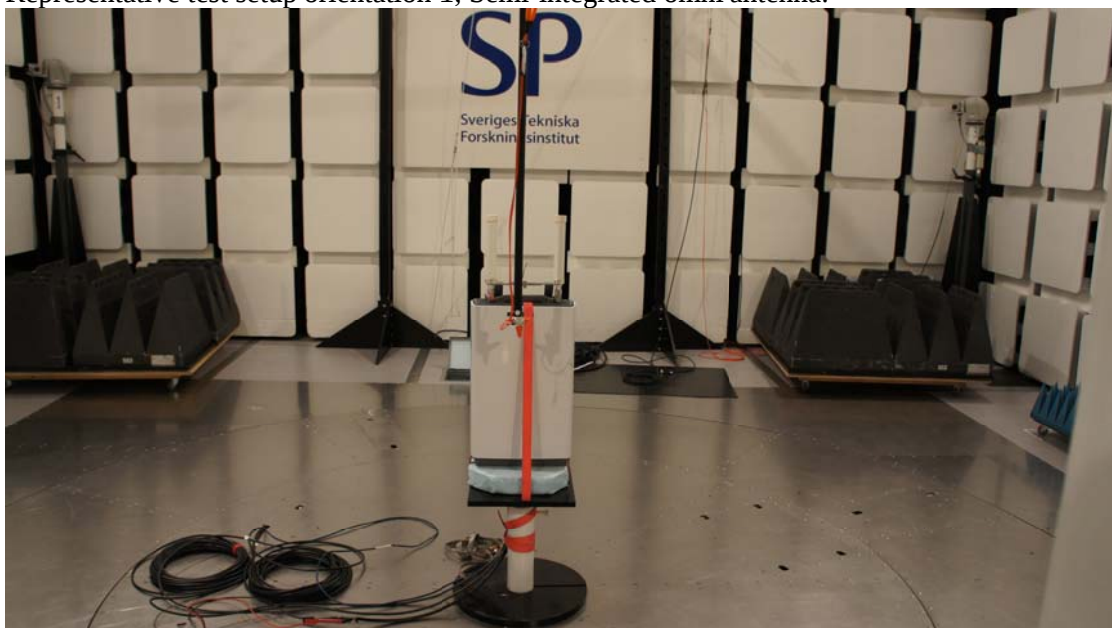
Representative test setup orientation 1, Semi-integrated omni antenna:
