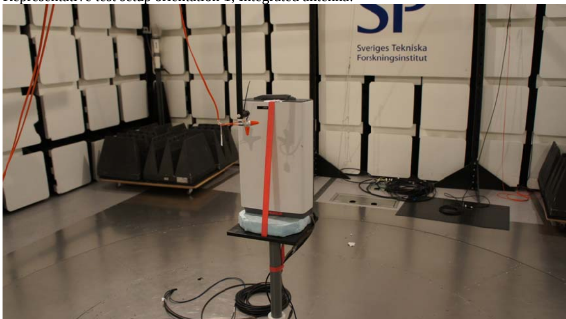
Representative test setup orientation 1, Integrated antenna:
