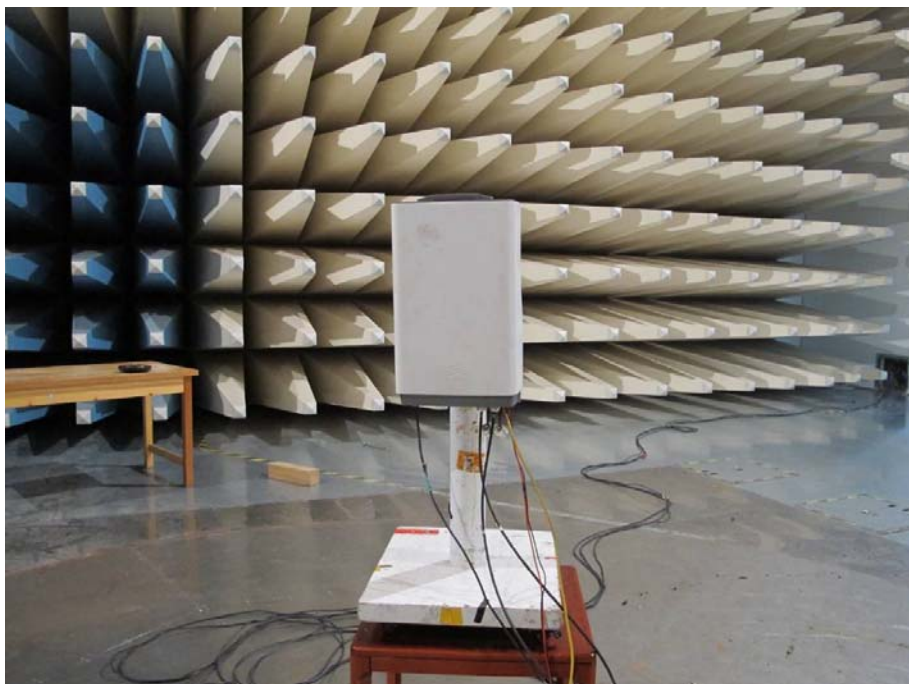
Maximum PEAK Output Power – Radiated (EIRP) Internal antenna KRE 101 2141/1, upright mounted
