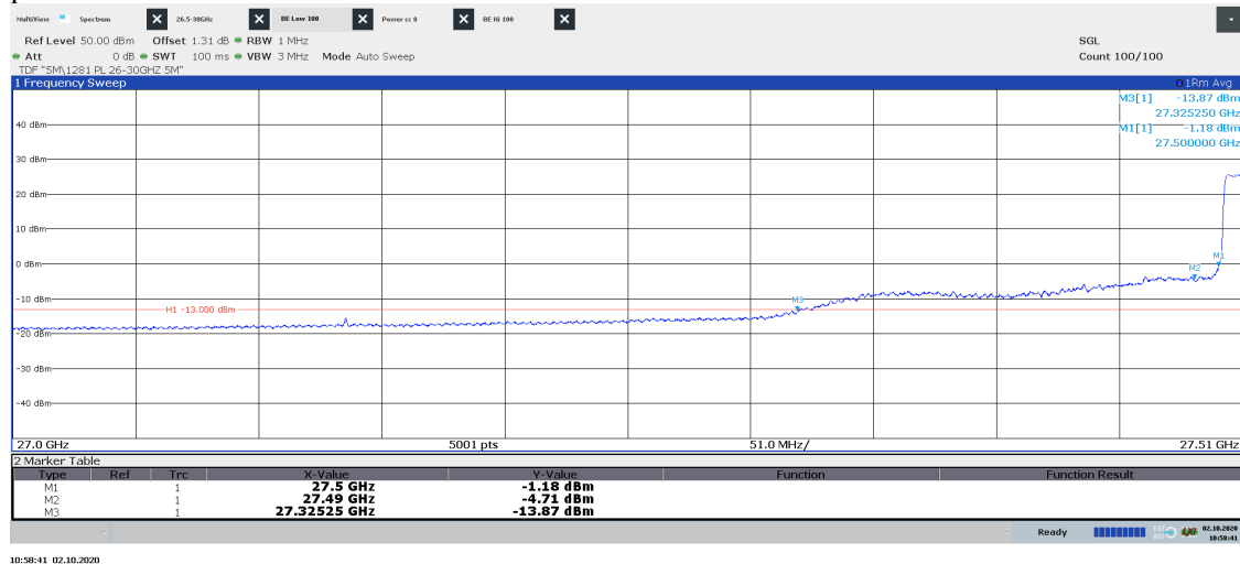
Diagram 2.12c: Pre scan 27.00 – 27.51 GHz, Symbolic name: BMT8 100 , EIRP Horizontal polarization
