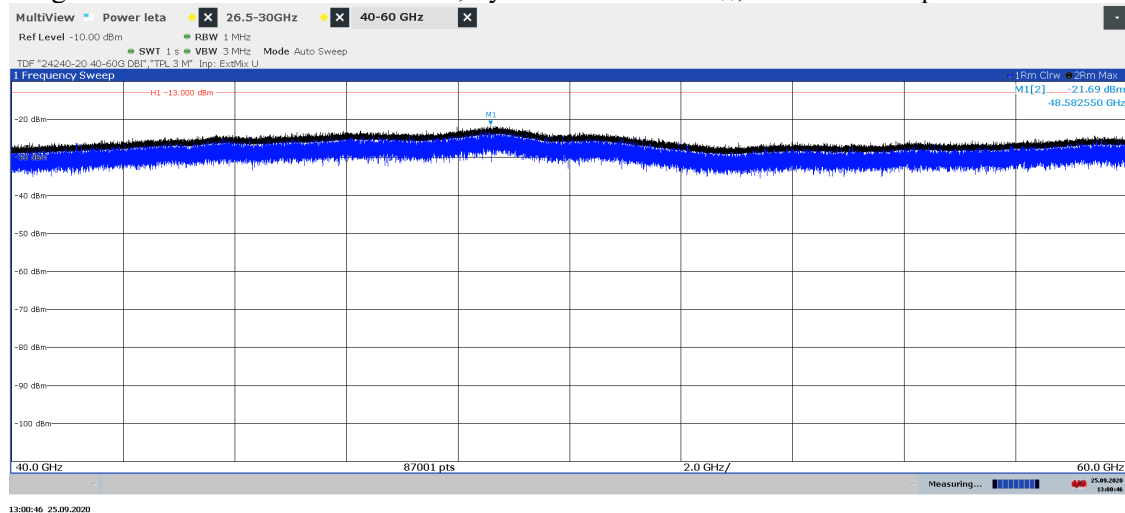
Diagram 2.14b: Pre scan 40 – 60 GHz, Symbolic name: BL 100 , EIRP Vertical polarization
