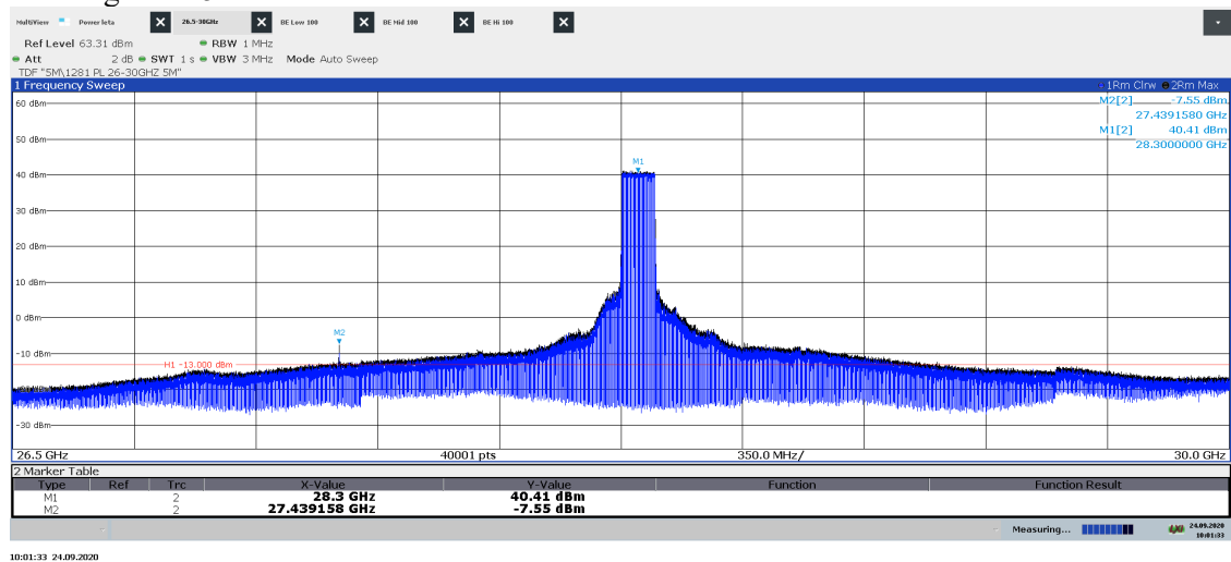
Diagram 2.5b: Pre scan 26.5 – 30.0 GHz, Symbolic name: TH 100 , EIRP Vertical polarization See diagram 2.5e for TRP result
