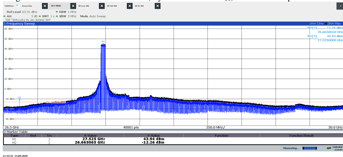
Diagram 2.4b: Pre scan 26.5 – 30.0 GHz, Symbolic name: BL 50 , EIRP Vertical polarization
