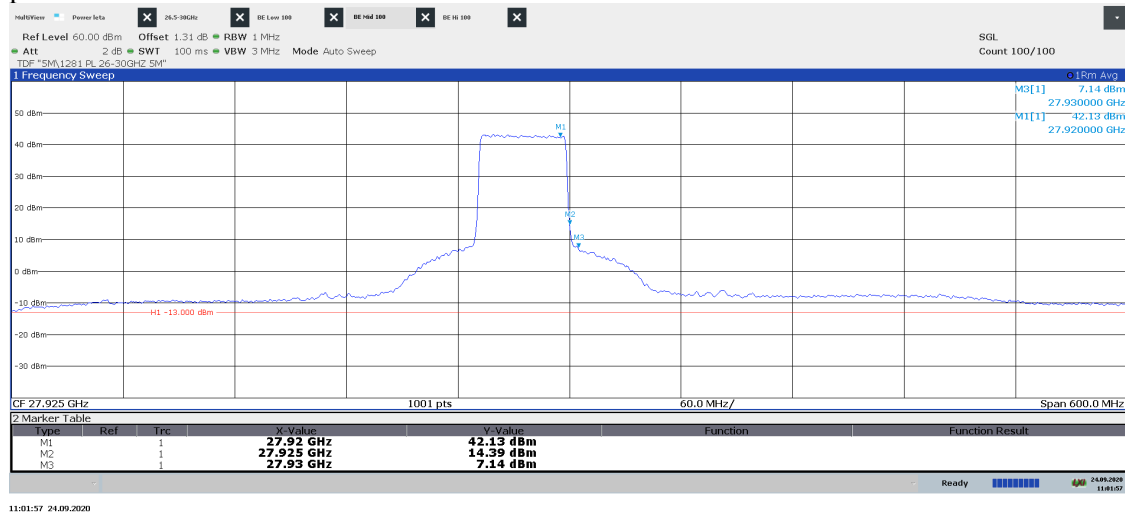
Diagram 2.7a: Pre scan 27.625 – 28.225 GHz, Symbolic name: TL 50 , EIRP Horizontal polarization
