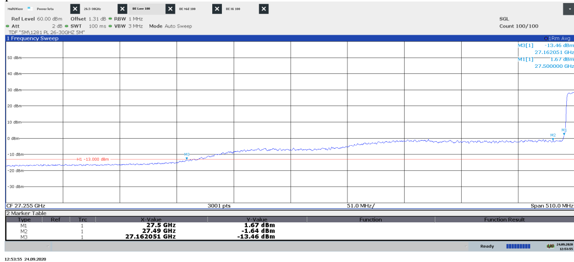
Diagram 2.11c: Pre scan 27.00 – 27.51 GHz, Symbolic name: BT8 100 , EIRP Horizontal polarization
