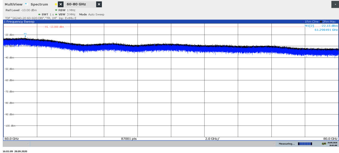
Diagram 2.15a: Pre scan 60 – 80 GHz, Symbolic name: BL 100 , EIRP Horizontal polarization
