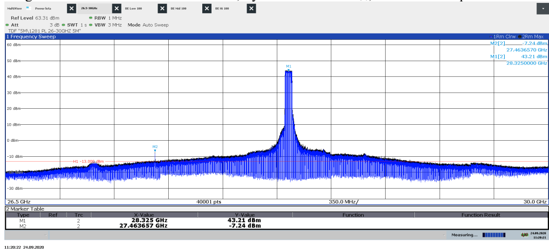
Diagram 2.9b: Pre scan 26.5 – 30.0 GHz, Symbolic name: TH 50 , EIRP Vertical polarization
