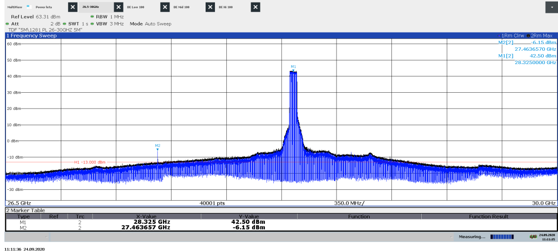
Diagram 2.9a: Pre scan 26.5 – 30.0 GHz, Symbolic name: TH 50 , EIRP Horizontal polarization
