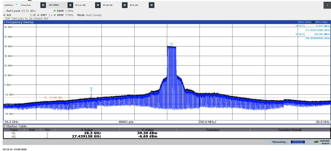
Diagram 2.5a: Pre scan 26.5 – 30.0 GHz, Symbolic name: TH 100 , EIRP Horizontal polarization See diagram 2.5e for TRP result
