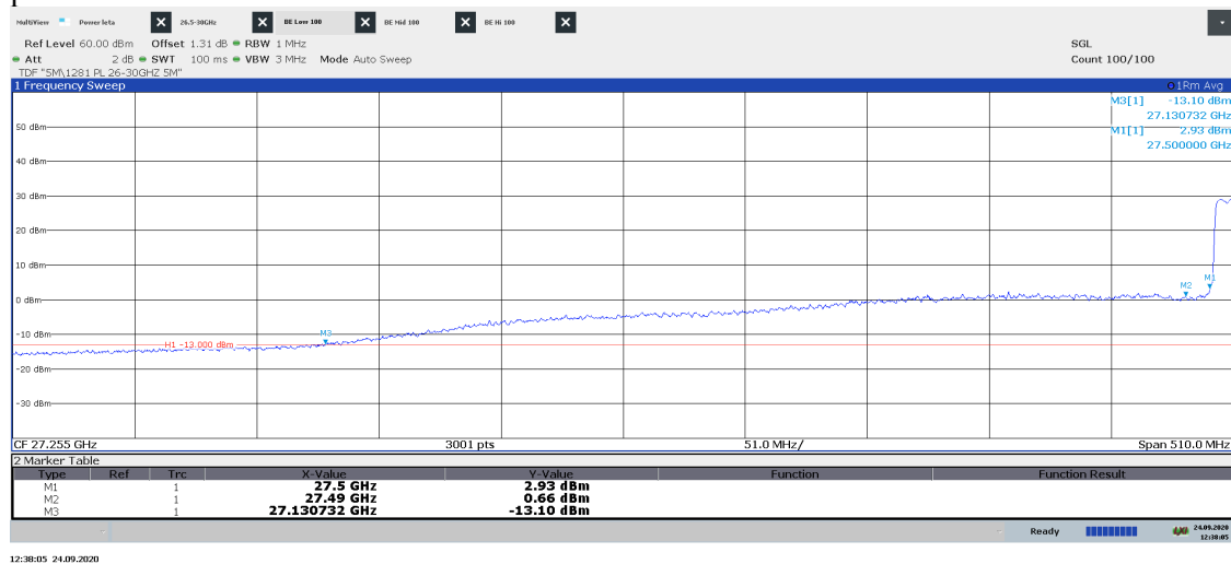
Diagram 2.11d: Pre scan 27.00 – 27.51 GHz, Symbolic name: BT8 100 , EIRP Vertical polarization
