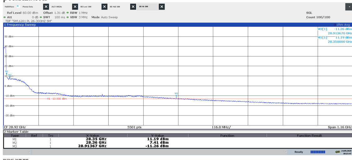
Diagram 2.5c: Pre scan 28.34 – 29.5GHz, Symbolic name: TH 100 , EIRP Horizontal polarization
