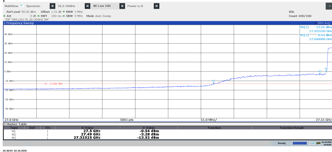
Diagram 2.12d: Pre scan 27.00 – 27.51 GHz, Symbolic name: BMT8 100 , EIRP Vertical polarization
