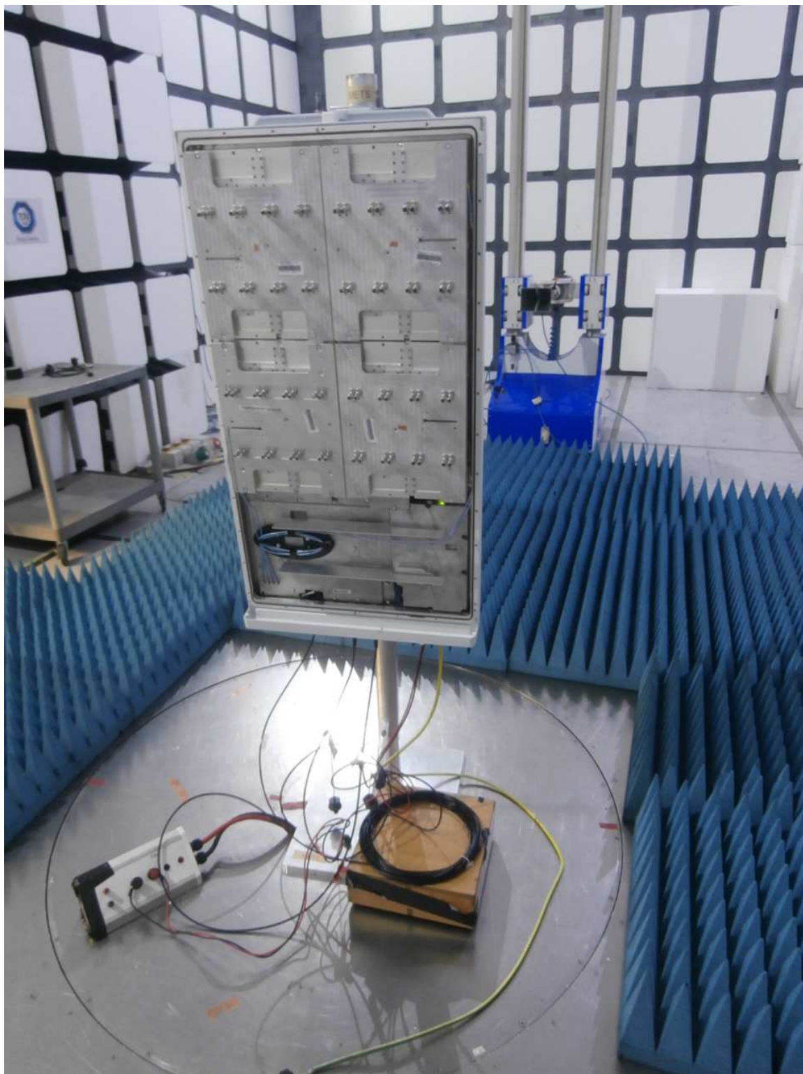
1GHz-8GHz – Radiated Emissions
