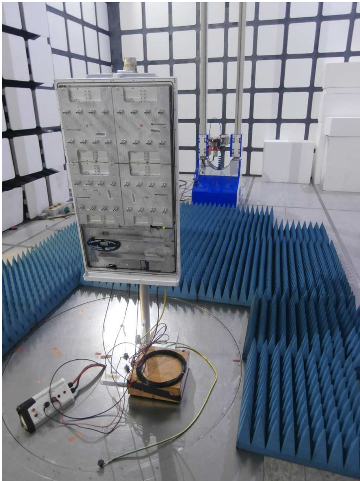
8GHz-18GHz – Radiated Emissions
