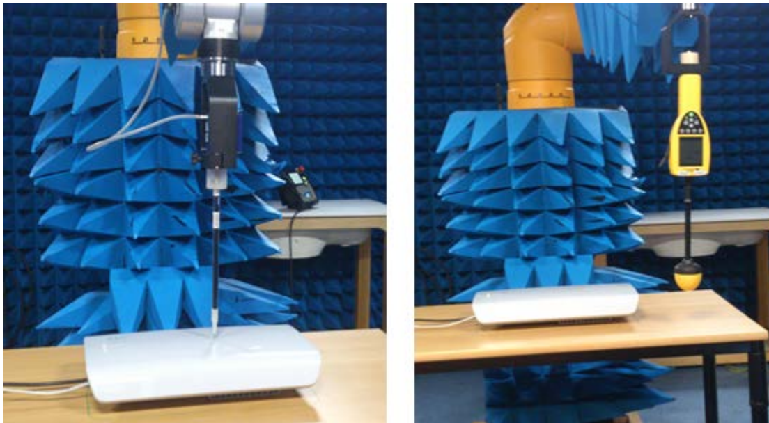
Figure C.1 (left) EUT positioned for field strength measurements using the DASY5 near-field scanner. (right) EUT positioned for field strength measurements using the Narda broadband meter.
