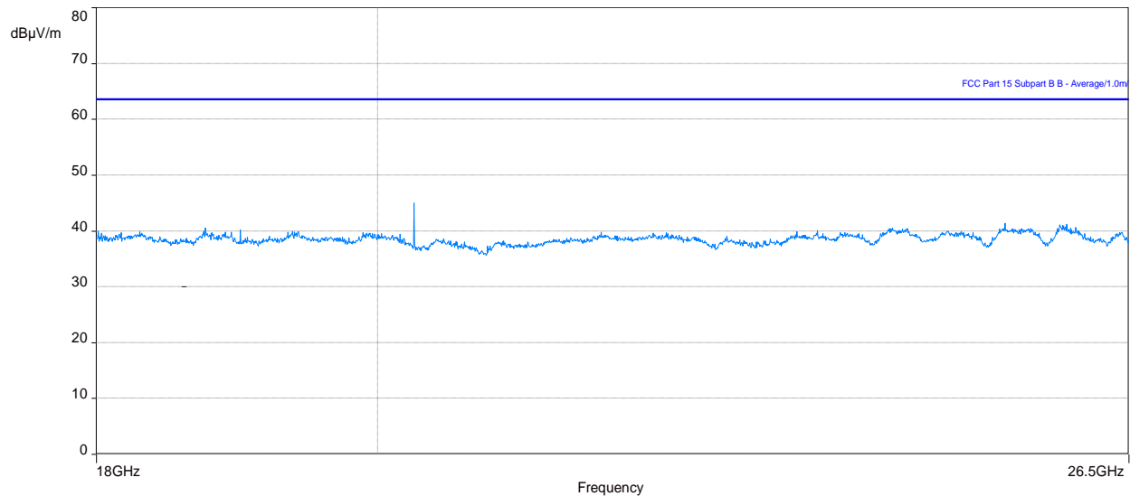
Figure 13: Plot of RE at 1m from 18 to 26.5 GHz (LTE – Middle chanel)
