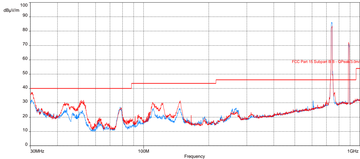
Figure 17: Plot of RE at 3 m – 30 to 1000 MHz (LTE – Top channel)
