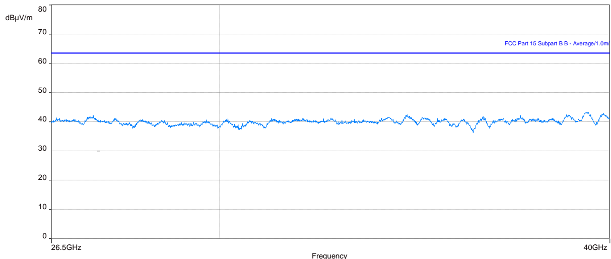
Figure 14: Plot of RE at 1m from 26.5 to 40 GHz (LTE – Middle chanel)
