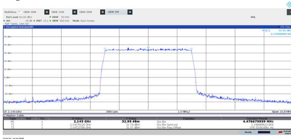
Diagram 1.16, E-TM1.1, M 5 , Port B:
