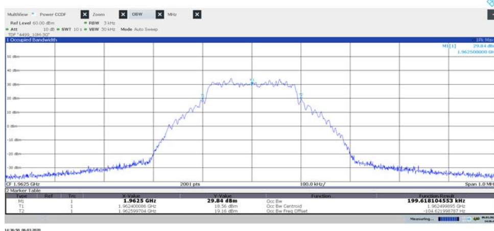
Diagram 1.39, NB IoT SA: N-TM, LTE: E-TM1.1, M_{IoT+L} , Port D:
