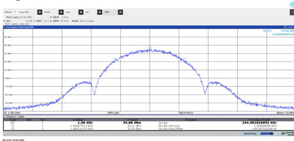
Diagram 1.34, GSM: 8PSK, LTE: E-TM1.1, M_{G+L} , Port C:
