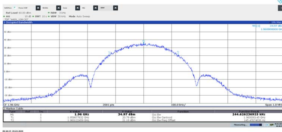
Diagram 1.33, GSM: 8PSK, LTE: E-TM1.1, M_{G+L} , Port B:
