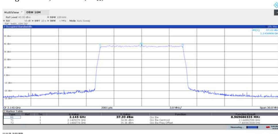
Diagram 1.17, E-TM1.1, M 10 , Port B:
