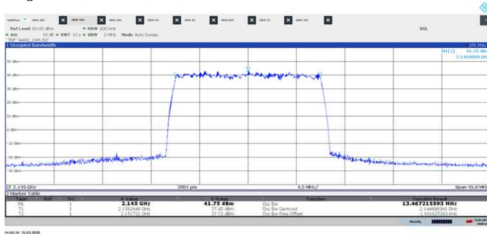
Diagram 1.22, E-TM3.2, M 15 , Port B:
