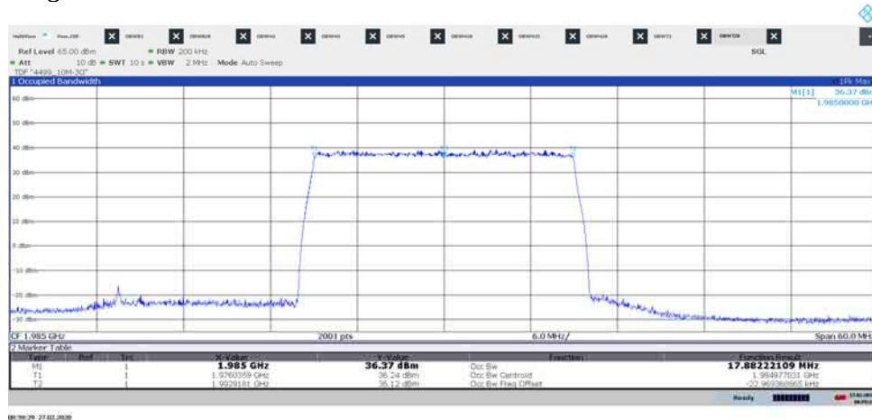
Diagram 1.7, E-TM3.1, T 20 , Port C:
