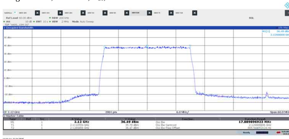
Diagram 1.24, E-TM3.1, B 20 , Port D:
