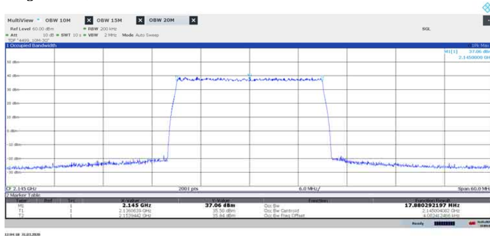
Diagram 1.19, E-TM1.1, M 20 , Port B:
