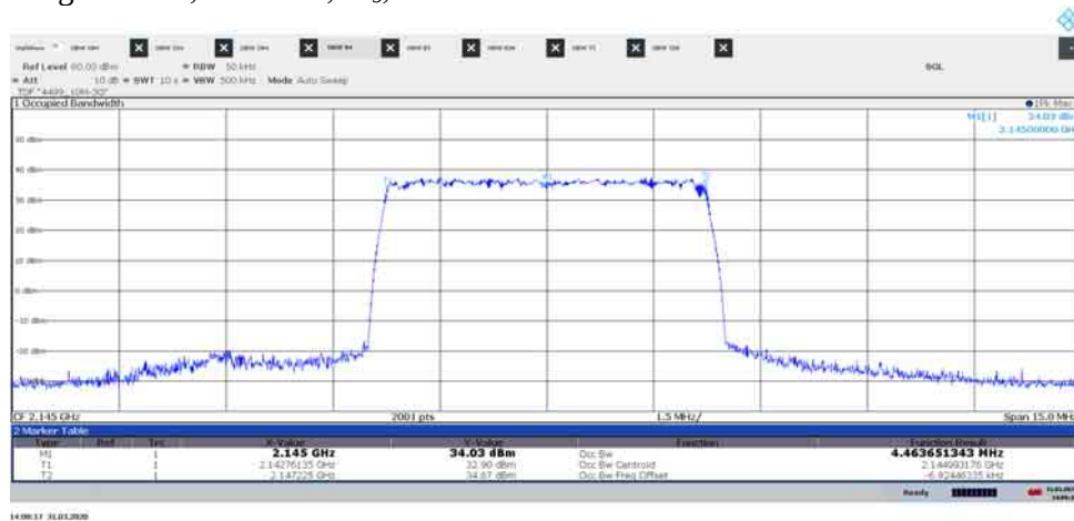
Diagram 1.20, E-TM3.2, M 5 , Port B:
