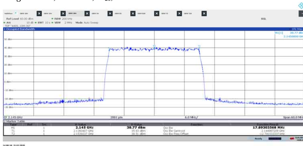
Diagram 1.23, E-TM3.2, M 20 , Port B:
