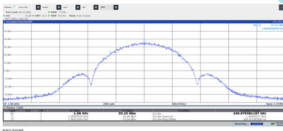
Diagram 1.32, GSM: 8PSK, LTE: E-TM1.1, M_{G+L} , Port A:
