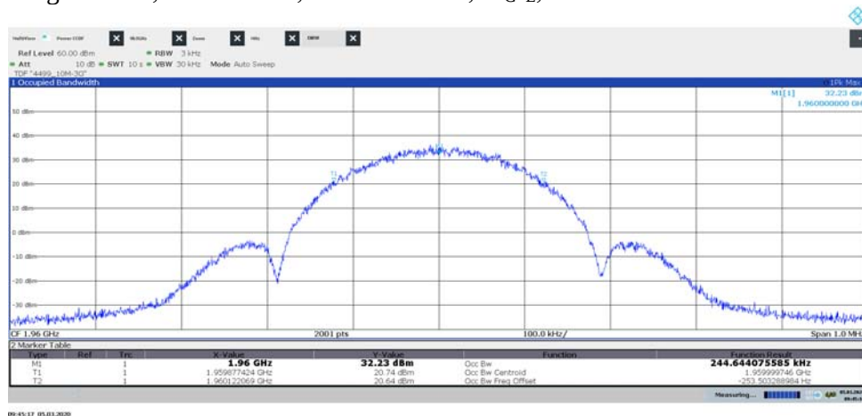
Diagram 1.35, GSM: 8PSK, LTE: E-TM1.1, M_{G+L} , Port D:
