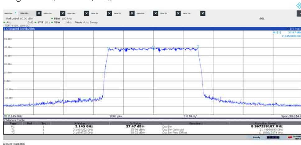
Diagram 1.21, E-TM3.2, M 10 , Port B:
