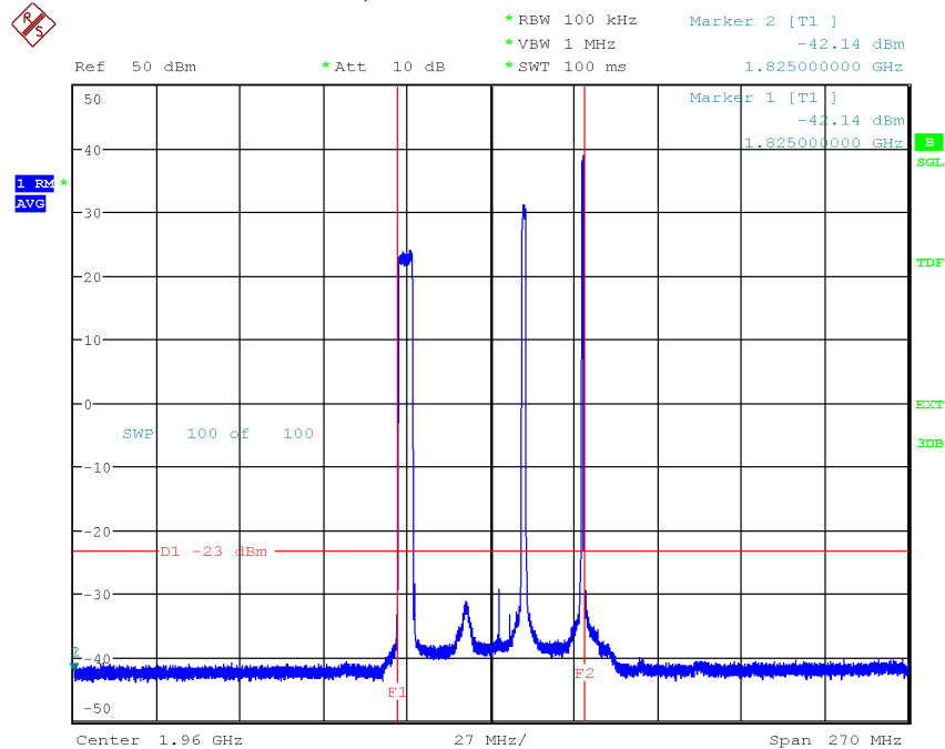
Diagram 3.20b, NR: NR-FR1-TM1.1, LTE: E-TM1.1, GSM: GMSK, \text{Tim}_{\text{NR}+\text{L}+\text{G}} , 1.8275 GHz – 2.0975 GHz, Port D:
