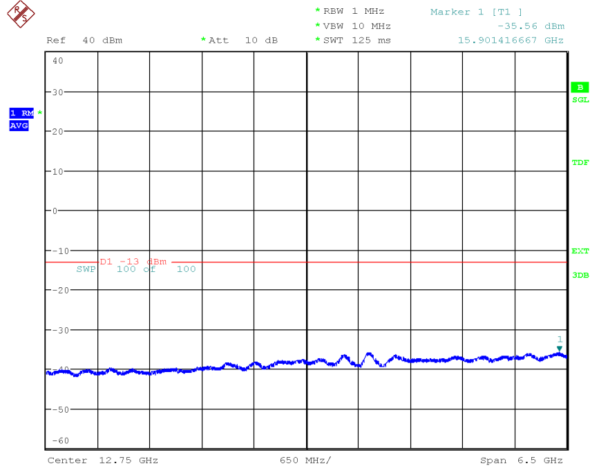
Diagram 3.31d, NR: NR-FR1-TM1.1, LTE: E-TM1.1, WCDMA: TM1, Bim NR+L+W , 9.5 GHz – 16 GHz, Port A:
