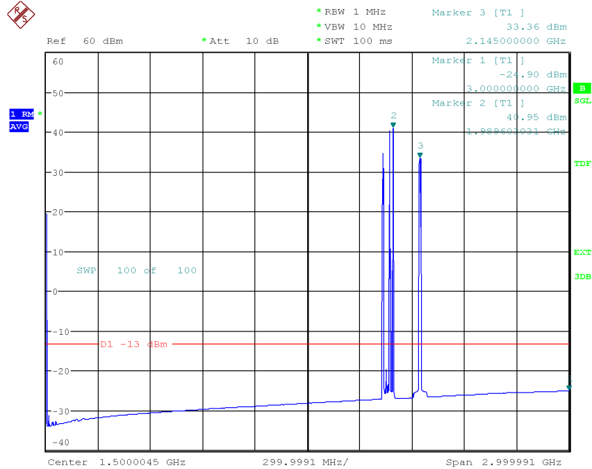
Diagram 3.20a, NR: NR-FR1-TM1.1, LTE: E-TM1.1, GSM: GMSK, \text{Tim}_{\text{NR}+\text{L}+\text{G}} , 9 kHz – 3 GHz, Port D:
