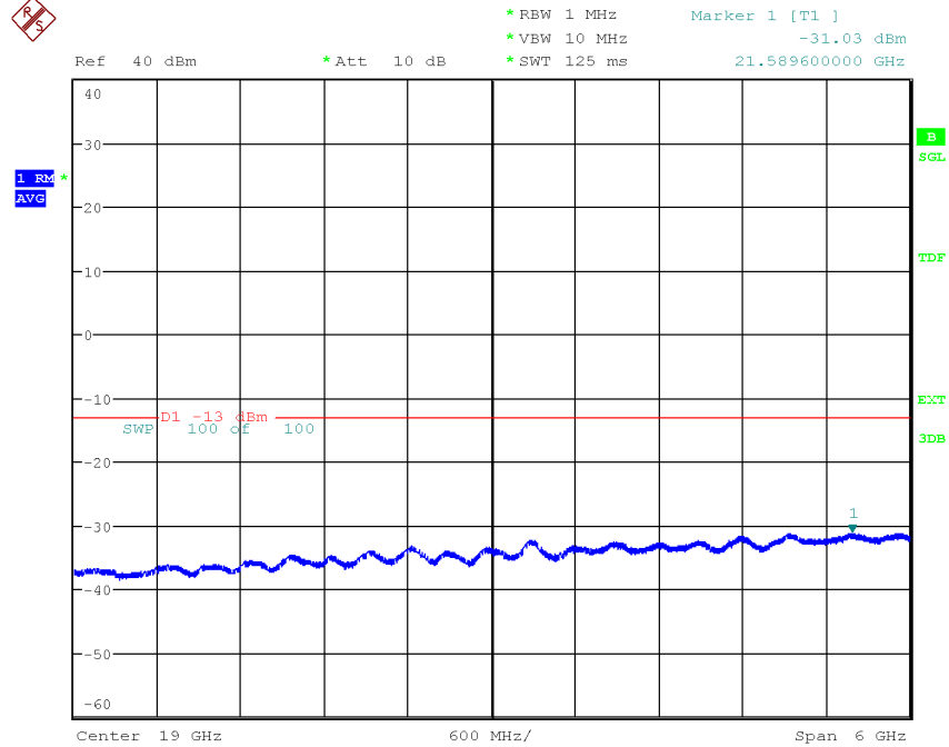
Diagram 3.20e, NR: NR-FR1-TM1.1, LTE: E-TM1.1, GSM: GMSK, \text{Tim}_{\text{NR}+\text{L}+\text{G}} , 16 GHz – 22 GHz, Port D:
