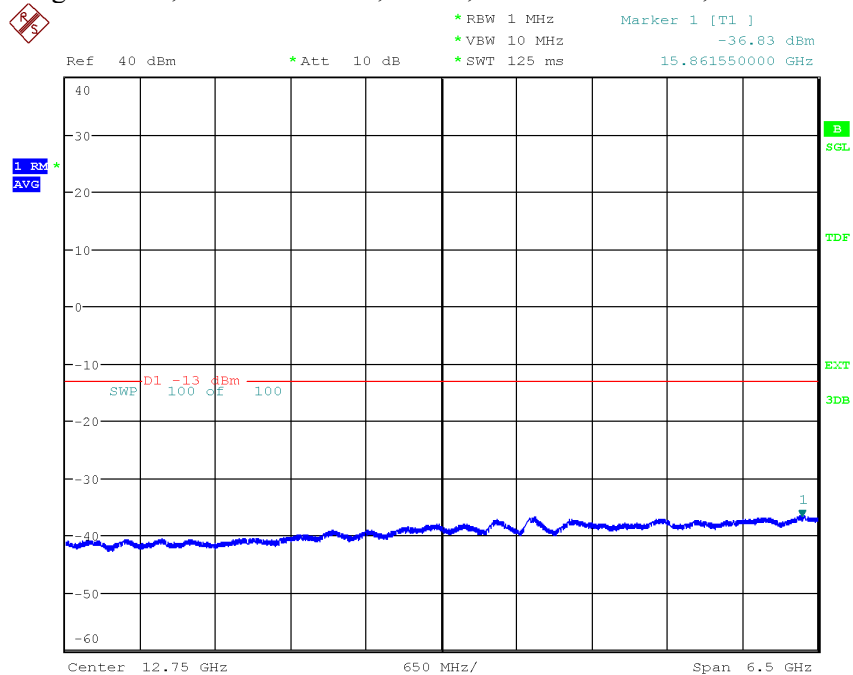
Diagram 3.8d, NR-FR1-TM1.1, \text{Tim}_{\text{NR}} , 9.5 GHz – 16 GHz, Port D:
