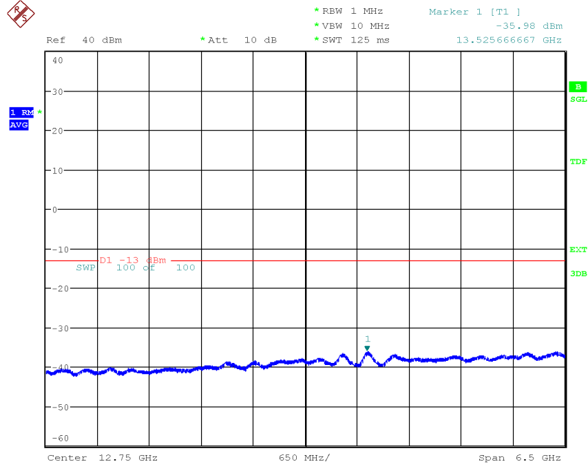
Diagram 3.25d, NR: NR-FR1-TM1.1, LTE: E-TM1.1, NB IoT SA: N-TM, Bim NR+L+IoT , 9.5 GHz – 16 GHz, Port A:
