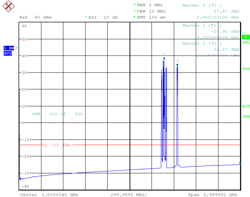
Diagram 3.24a, NR: NR-FR1-TM1.1, LTE: E-TM1.1, NB IoT SA: N-TM, Max NR+L+IoT , 9 kHz – 3 GHz, Port D:
