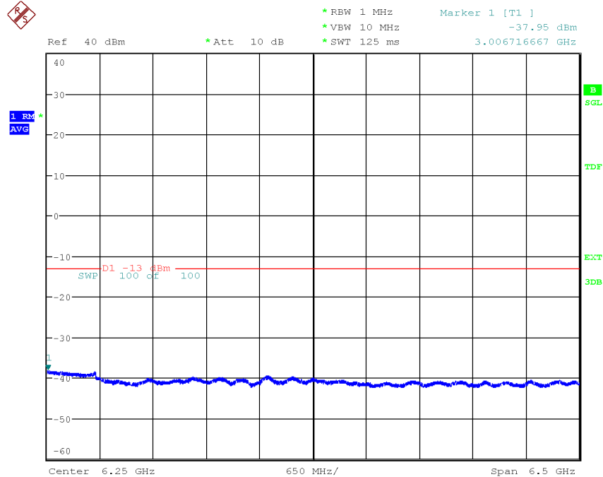
Diagram 3.25c, NR: NR-FR1-TM1.1, LTE: E-TM1.1, NB IoT SA: N-TM, Bim NR+L+IoT , 3 GHz – 9.5 GHz, Port A:
