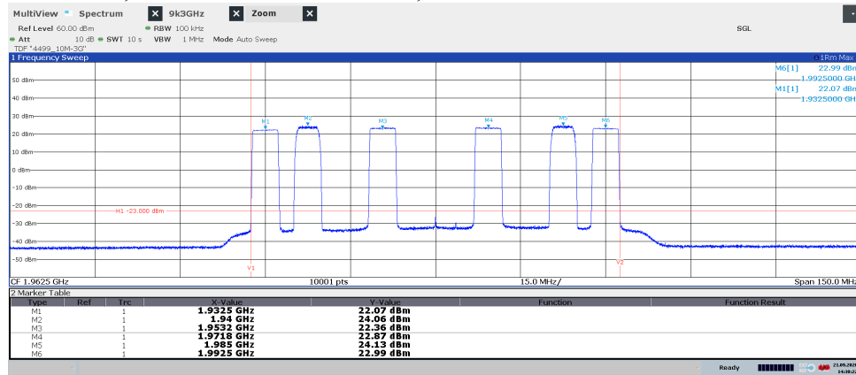
Diagram 3.30b, NR: NR-FR1-TM1.1, LTE: E-TM1.1, WCDMA: TM1, Max NR+L+W , 1.8275 GHz – 2.0975 GHz, Port D:
