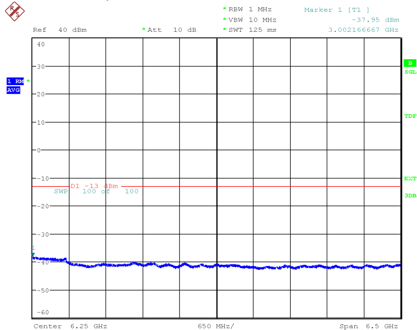
Diagram 3.20c, NR: NR-FR1-TM1.1, LTE: E-TM1.1, GSM: GMSK, \text{Tim}_{\text{NR}+\text{L}+\text{G}} , 3 GHz – 9.5 GHz, Port D:
