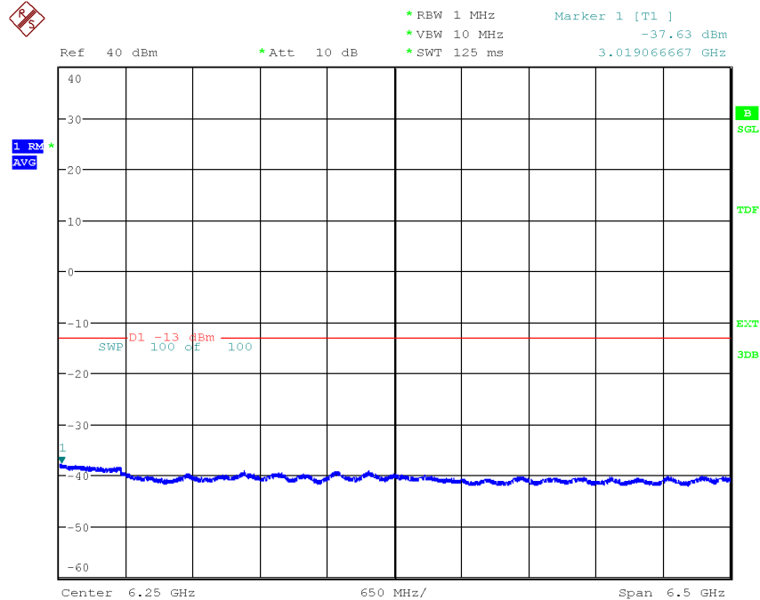
Diagram 3.31c, NR: NR-FR1-TM1.1, LTE: E-TM1.1, WCDMA: TM1, Bim NR+L+W , 3 GHz – 9.5 GHz, Port A:
