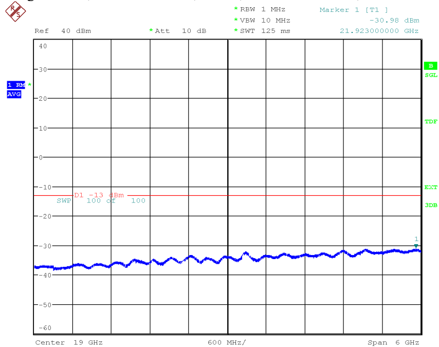
Diagram 3.8e, NR-FR1-TM1.1, \text{Tim}_{\text{NR}} , 16 GHz – 22 GHz, Port D:
