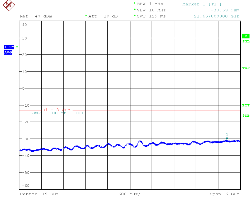
Diagram 3.31e, NR: NR-FR1-TM1.1, LTE: E-TM1.1, WCDMA: TM1, Bim NR+L+W , 16 GHz – 22 GHz, Port A:
