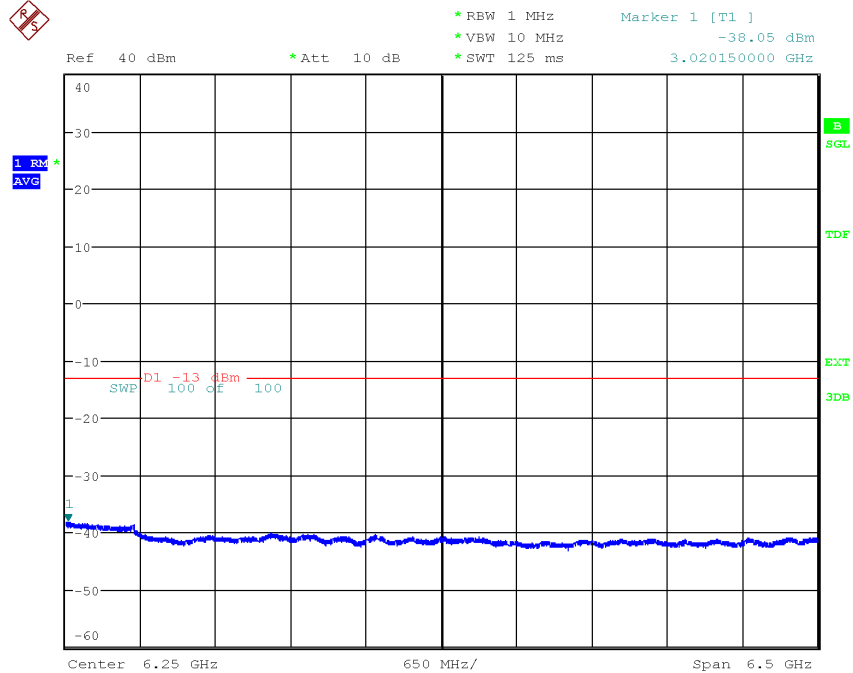
Diagram 3.8c, NR-FR1-TM1.1, \text{Tim}_{\text{NR}} , 3 GHz – 9.5 GHz, Port D:
