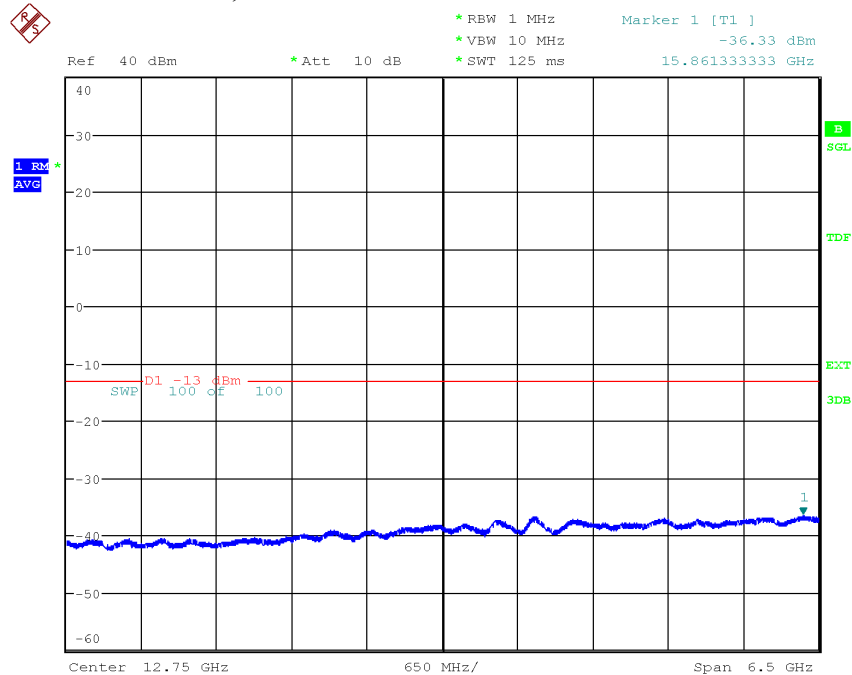
Diagram 3.20d, NR: NR-FR1-TM1.1, LTE: E-TM1.1, GSM: GMSK, \text{Tim}_{\text{NR}+\text{L}+\text{G}} , 9.5 GHz – 16 GHz, Port D:
