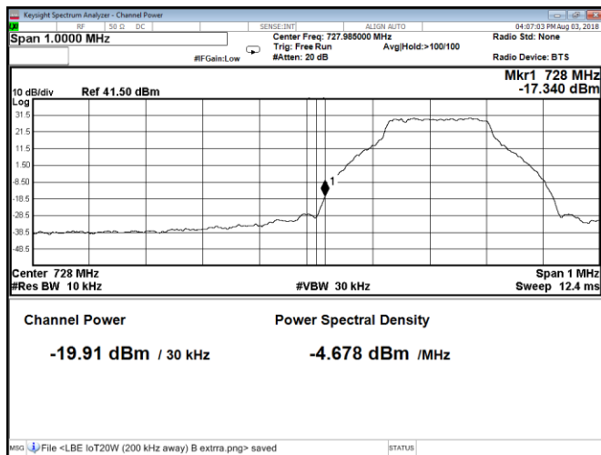
Figure 8.2-363: Conducted band edge emission at 728 MHz, Port C, Band 85A IoT stand-alone 200 kHz away from the band edge
