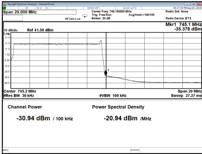
Figure 8.2-389: Conducted band edge emission at 745.1 MHz, Port A, QPSK, Band 85A IoT + LTE 10 MHz channel
