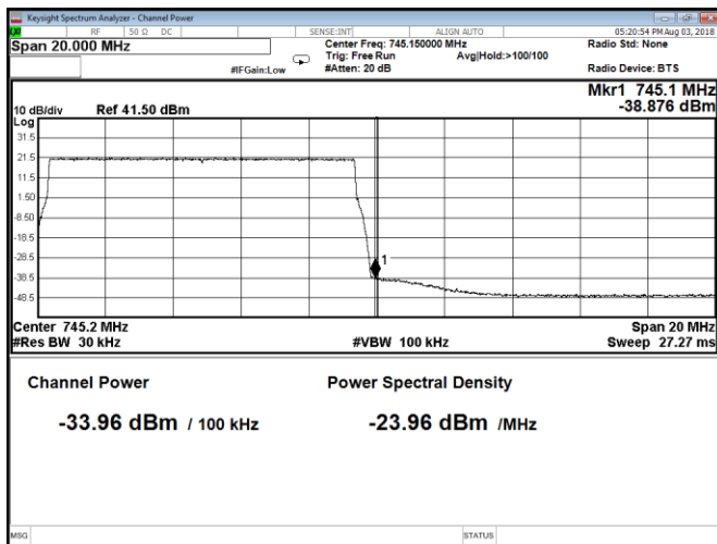
Figure 8.2-383: Conducted band edge emission at 745.1 MHz, Port C, QPSK, Band 85A 10 MHz channel
