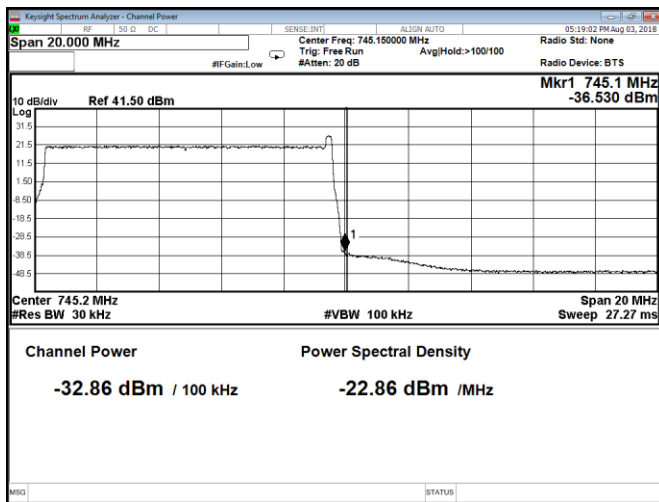
Figure 8.2-391: Conducted band edge emission at 745.1 MHz, Port C, QPSK, Band 85A IoT + LTE 10 MHz channel
