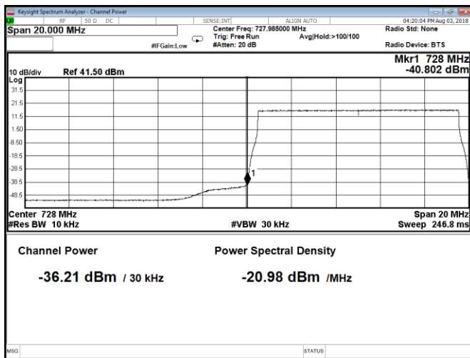
Figure 8.2-343: Conducted band edge emission at 728 MHz, Port C, QPSK, Band 85A 10 MHz channel
