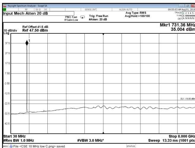
Figure 8.2-62: Conducted spurious emissions at Port B, QPSK, Band 85A low 10 MHz channel
