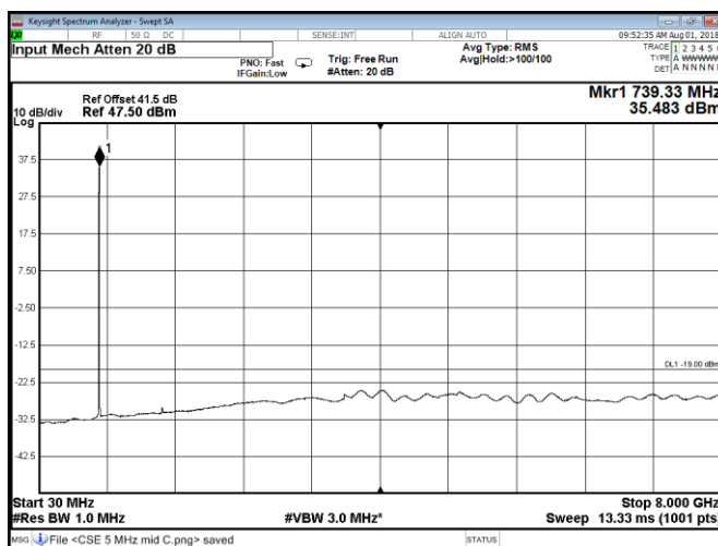
Figure 8.2-54: Conducted spurious emissions at Port B, QPSK, Band 85A mid 5 MHz channel
