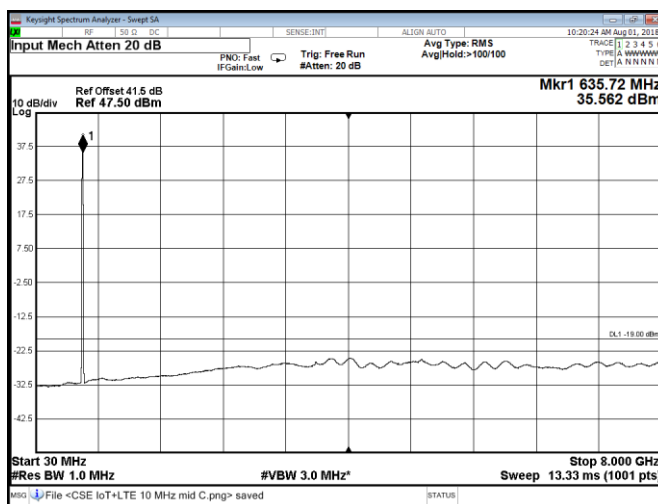
Figure 8.2-78: Conducted spurious emissions at Port B, QPSK, Band 71 mid 10 MHz channel + IoT carrier
