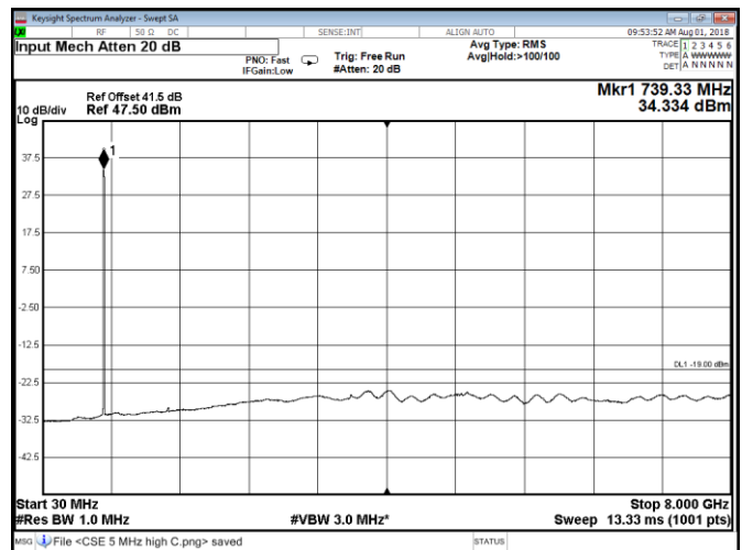
Figure 8.2-60: Conducted spurious emissions at Port D, QPSK, Band 85A high 5 MHz channel
