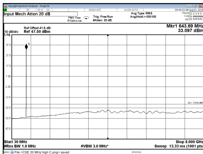
Figure 8.2-46: Conducted spurious emissions at Port B, QPSK, Band 71 high 20 MHz channel
