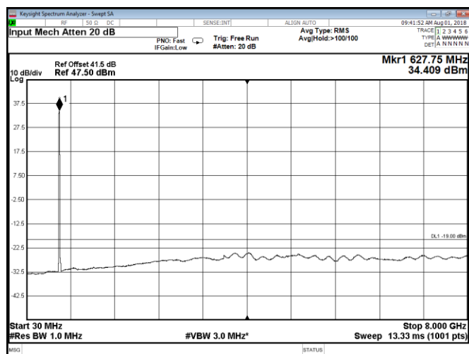
Figure 8.2-25: Conducted spurious emissions at Port A, QPSK, Band 71 low 15 MHz channel
