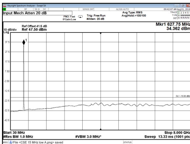
Figure 8.2-26: Conducted spurious emissions at Port B, QPSK, Band 71 low 15 MHz channel
