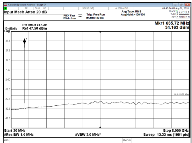
Figure 8.2-32: Conducted spurious emissions at Port D, QPSK, Band 71 mid 15 MHz channel
