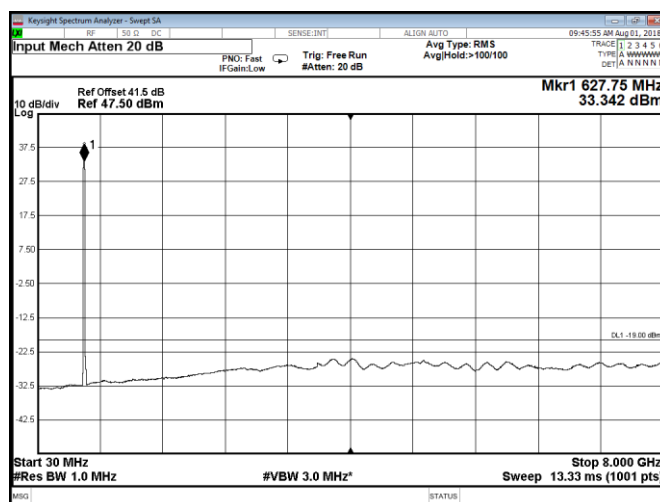
Figure 8.2-40: Conducted spurious emissions at Port D, QPSK, Band 71 low 20 MHz channel
