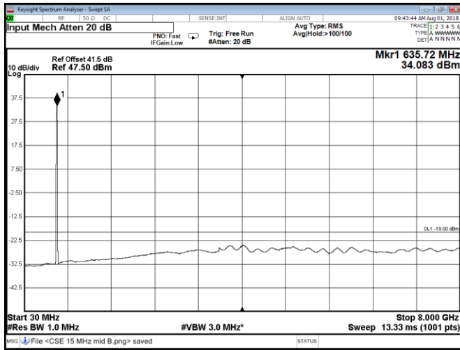
Figure 8.2-29: Conducted spurious emissions at Port A, QPSK, Band 71 mid 15 MHz channel
