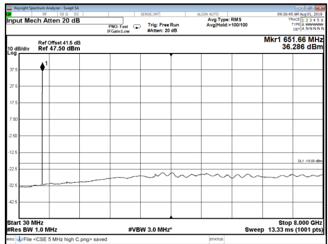
Figure 8.2-12: Conducted spurious emissions at Port D, QPSK, Band 71 high 5 MHz channel
