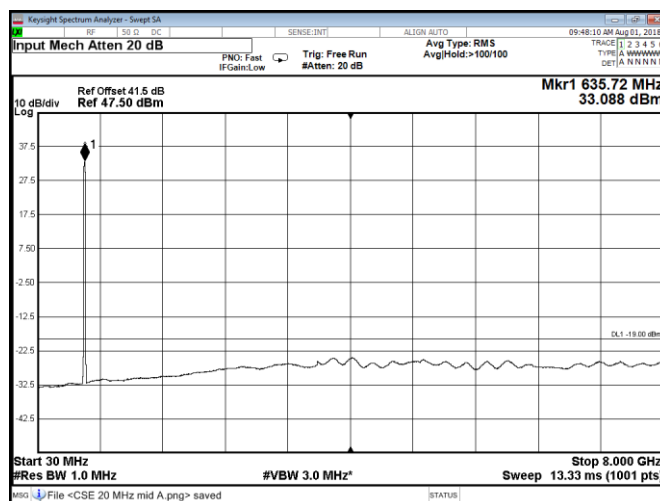
Figure 8.2-42: Conducted spurious emissions at Port B, QPSK, Band 71 mid 20 MHz channel
