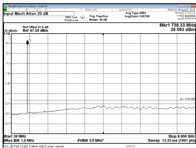
Figure 8.2-55: Conducted spurious emissions at Port C, QPSK, Band 85A mid 5 MHz channel
