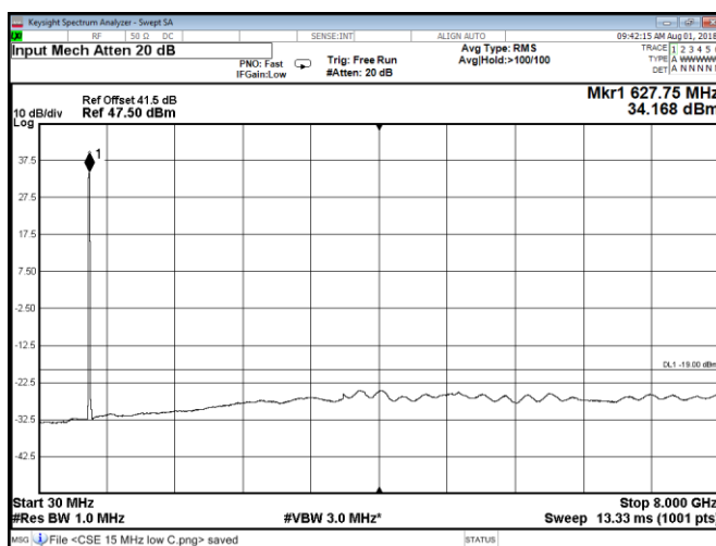
Figure 8.2-28: Conducted spurious emissions at Port D, QPSK, Band 71 low 15 MHz channel
