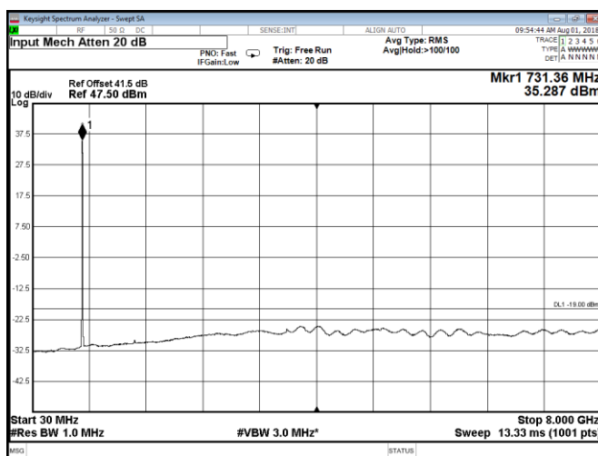
Figure 8.2-64: Conducted spurious emissions at Port D, QPSK, Band 85A low 10 MHz channel
