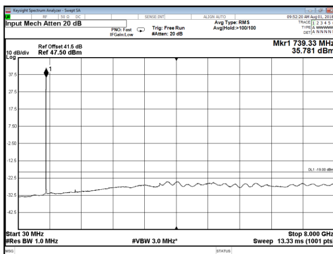
Figure 8.2-56: Conducted spurious emissions at Port D, QPSK, Band 85A mid 5 MHz channel
