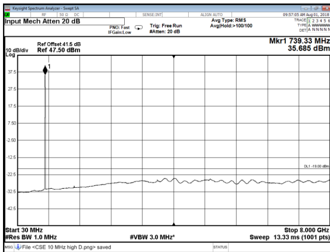
Figure 8.2-71: Conducted spurious emissions at Port C, QPSK, Band 85A high 10 MHz channel
