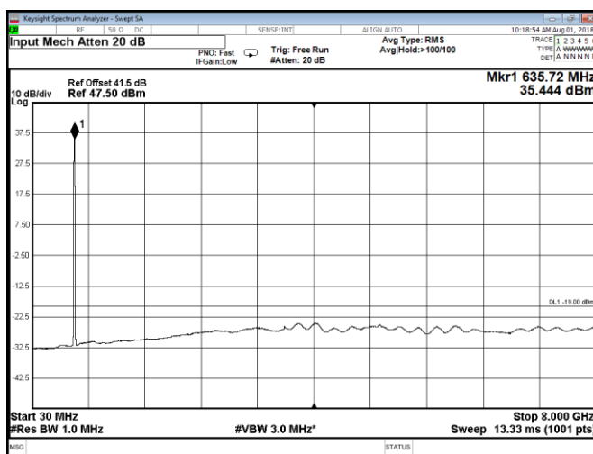
Figure 8.2-80: Conducted spurious emissions at Port D, QPSK, Band 71 mid 10 MHz channel + IoT carrier
