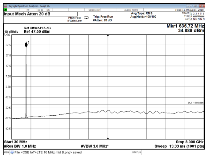
Figure 8.2-77: Conducted spurious emissions at Port A, QPSK, Band 71 mid 10 MHz channel + IoT carrier
