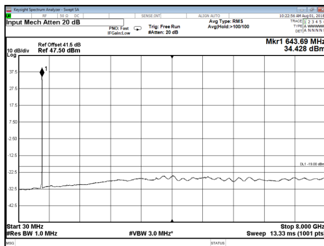
Figure 8.2-82: Conducted spurious emissions at Port B, QPSK, Band 71 high 10 MHz channel + IoT carrier
