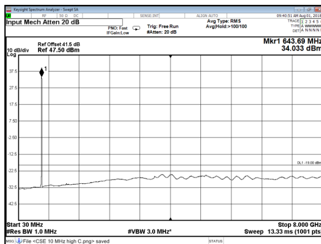
Figure 8.2-22: Conducted spurious emissions at Port B, QPSK, Band 71 high 10 MHz channel
