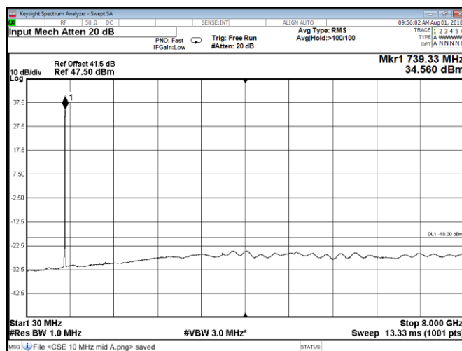
Figure 8.2-66: Conducted spurious emissions at Port B, QPSK, Band 85A mid 10 MHz channel
