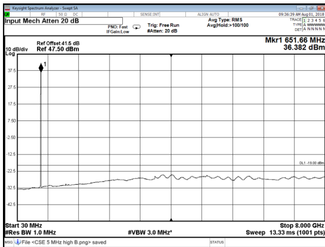
Figure 8.2-11: Conducted spurious emissions at Port C, QPSK, Band 71 high 5 MHz channel
