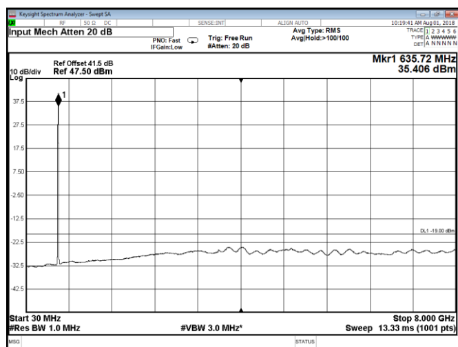
Figure 8.2-79: Conducted spurious emissions at Port C, QPSK, Band 71 mid 10 MHz channel + IoT carrier
