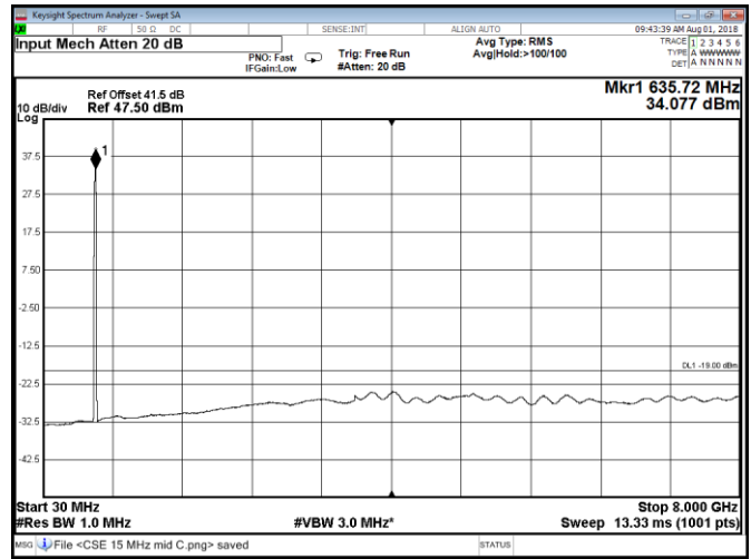
Figure 8.2-30: Conducted spurious emissions at Port B, QPSK, Band 71 mid 15 MHz channel
