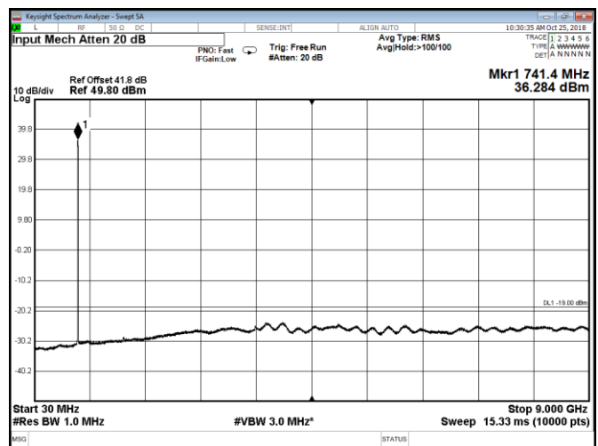
Figure 8.3-54: Conducted spurious emissions for 10 MHz mid channel with 2xIoT, with 40 W configuration at Port B
