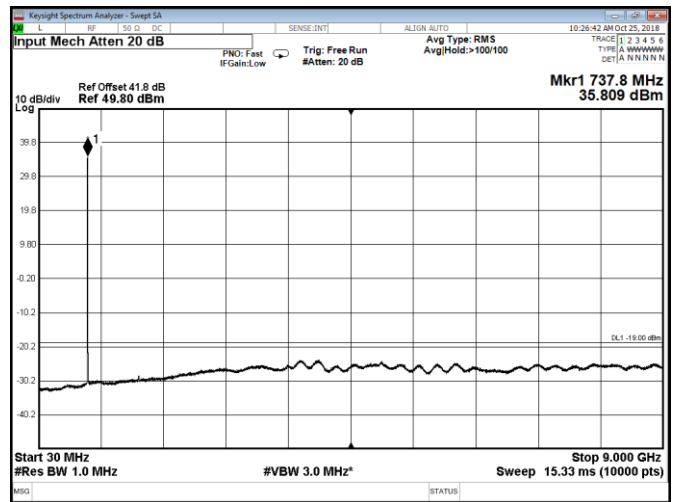
Figure 8.3-52: Conducted spurious emissions for 10 MHz low channel with IoT, with 40 W configuration at Port D
