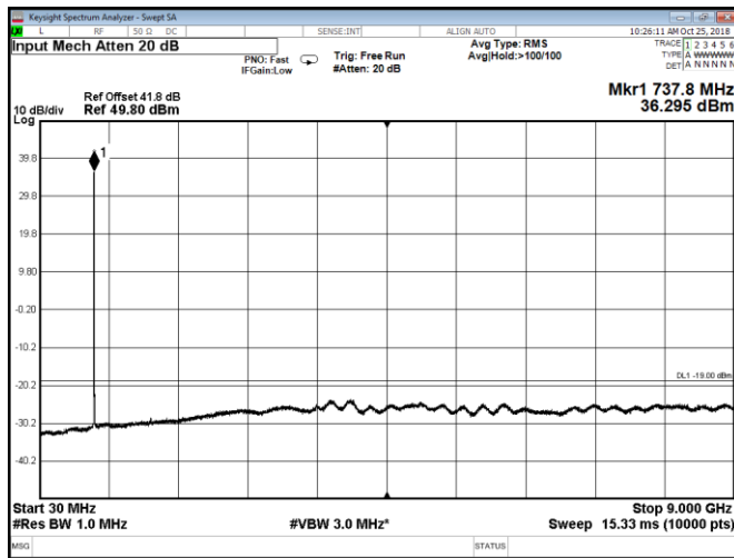
Figure 8.3-51: Conducted spurious emissions for 10 MHz low channel with IoT, with 40 W configuration at Port C
