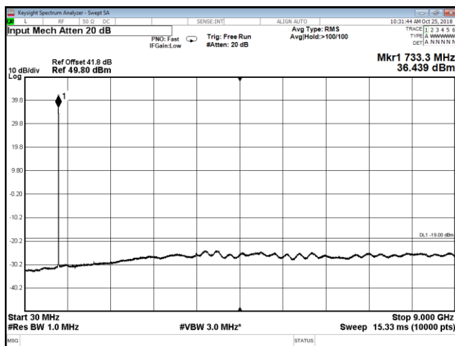
Figure 8.3-53: Conducted spurious emissions for 10 MHz mid channel with 2xIoT, with 40 W configuration at Port A
