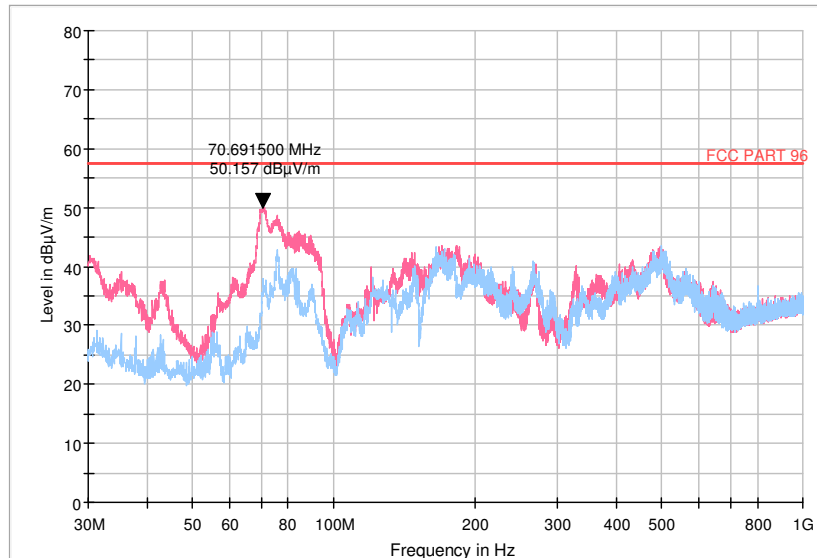
Range 30-1000MHz, Horizontal & Vertical
