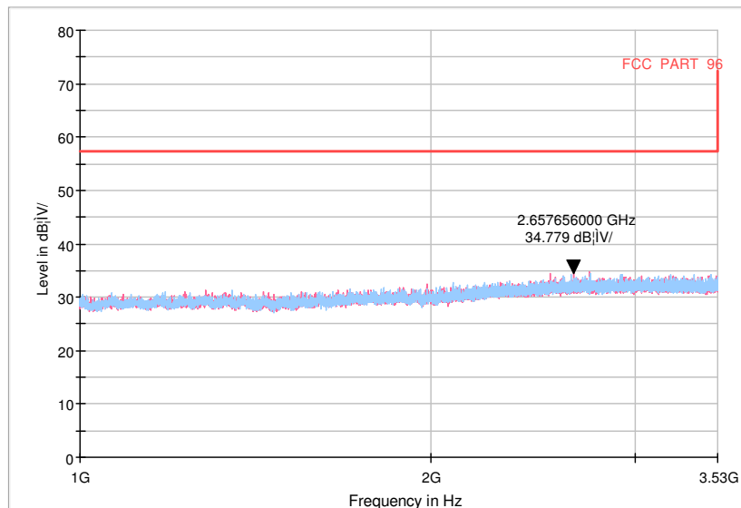
Range 1-3.53GHz, Horizontal & Vertical
